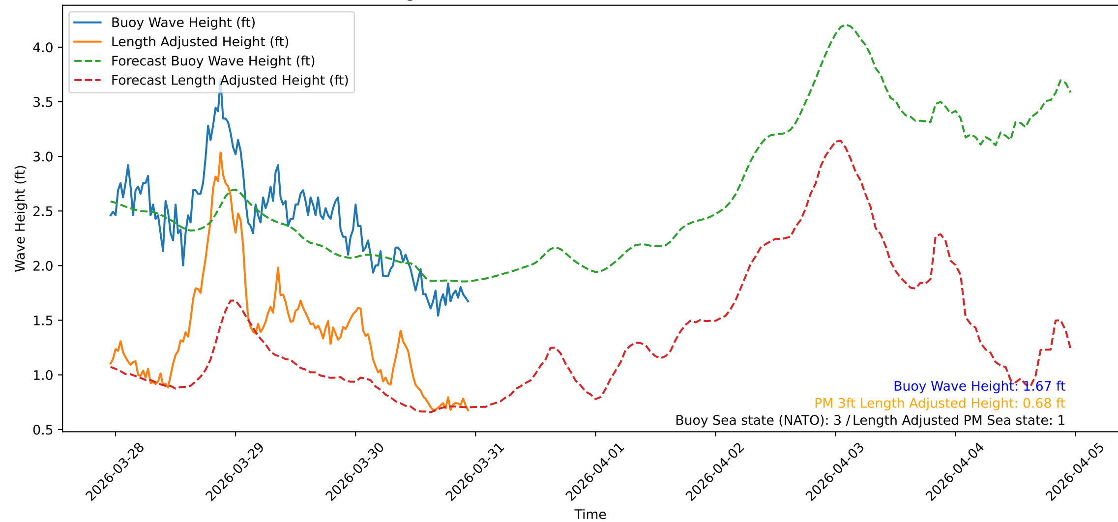
Wave Heights over Time for Green Beach at 2026-03-30 23:11:09
