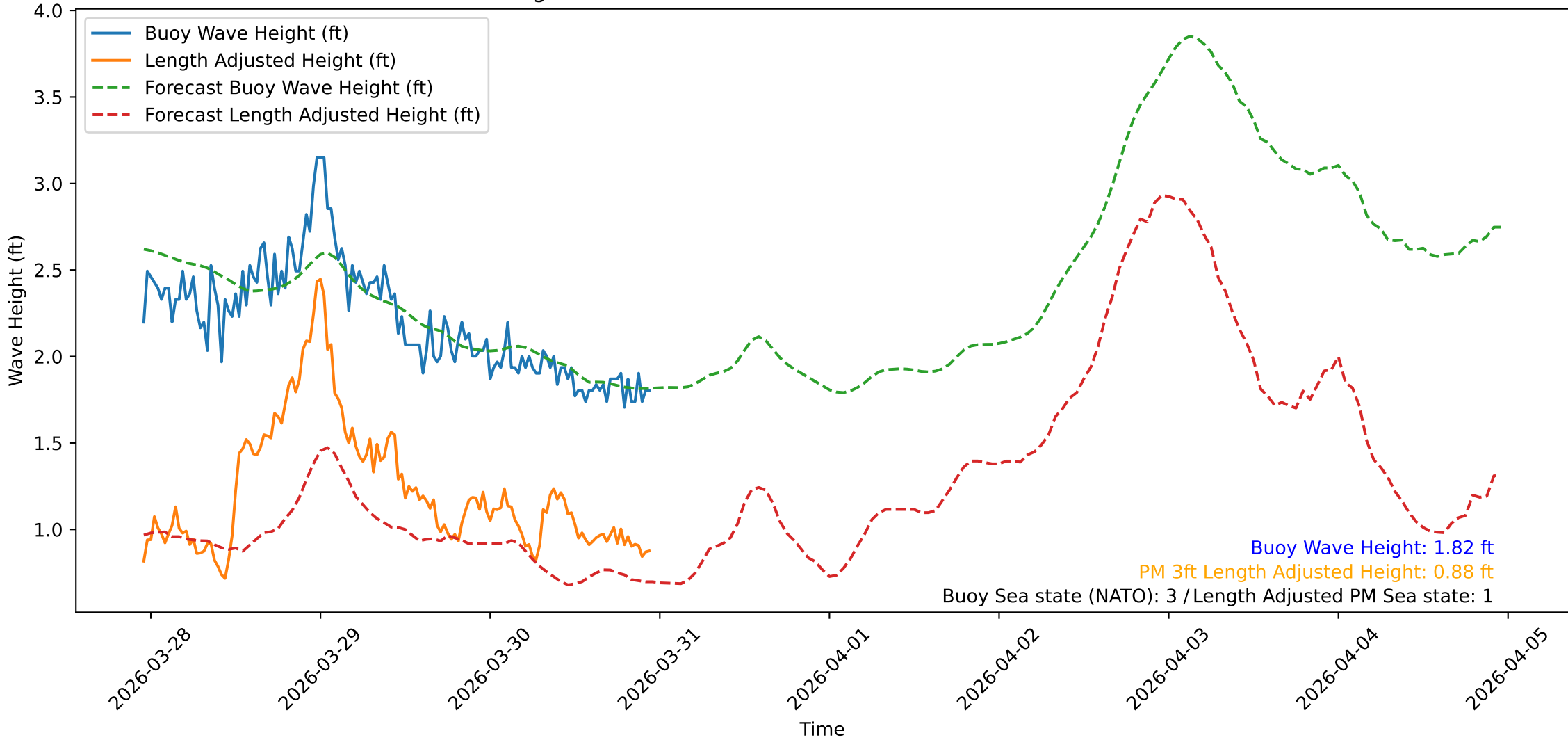
Wave Heights over Time for Oceanside Harbor at 2026-03-30 23:10:31
