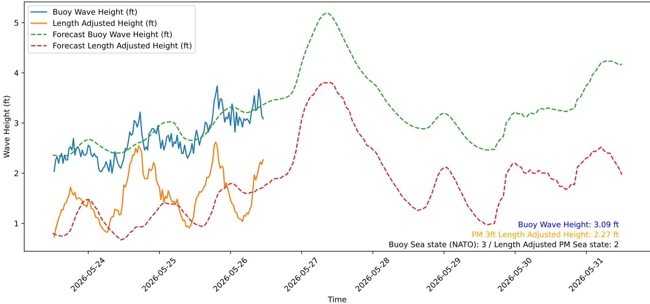
Wave Heights over Time for Red Beach at 2026-05-26 12:00:46
