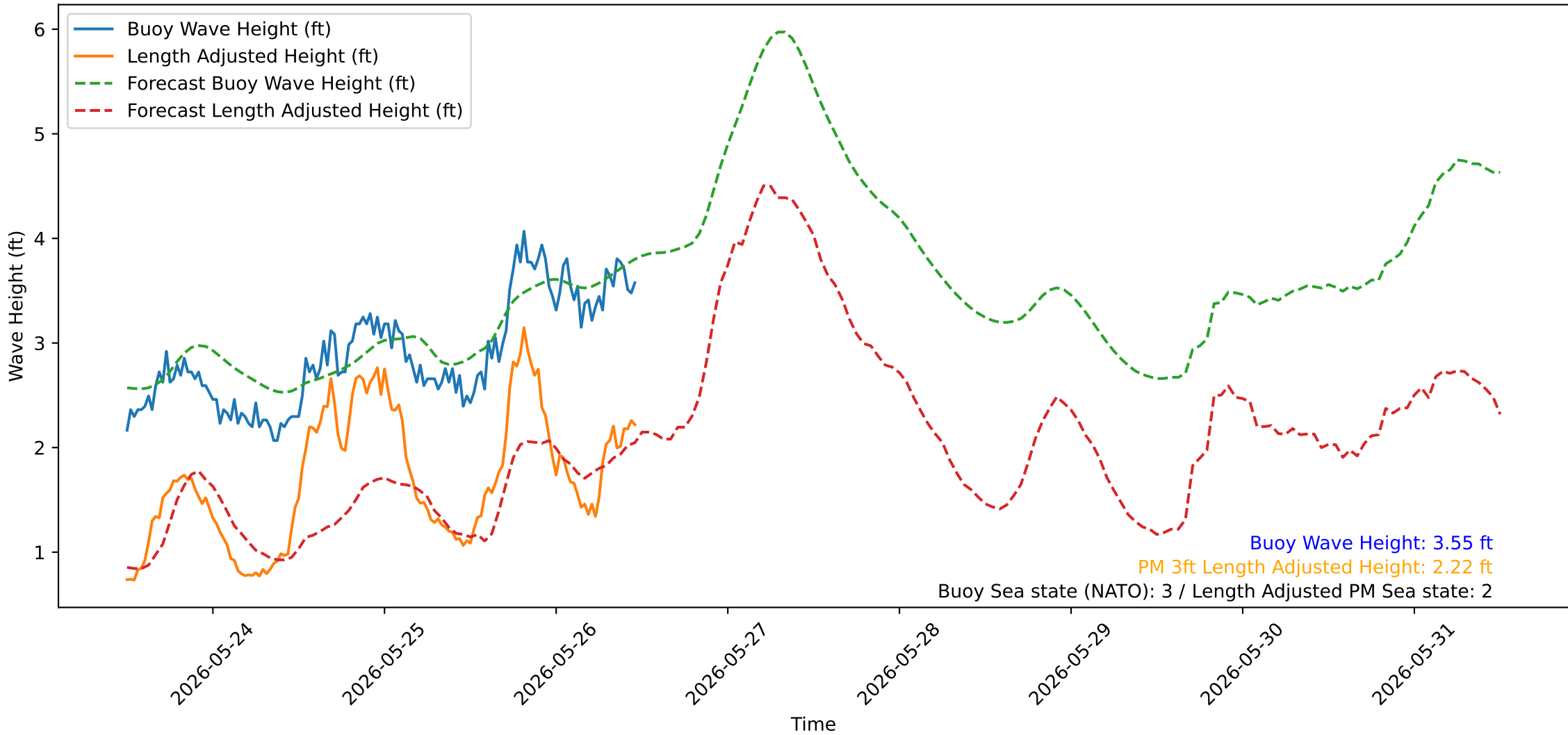
Wave Heights over Time for Green Beach at 2026-05-26 12:01:09
