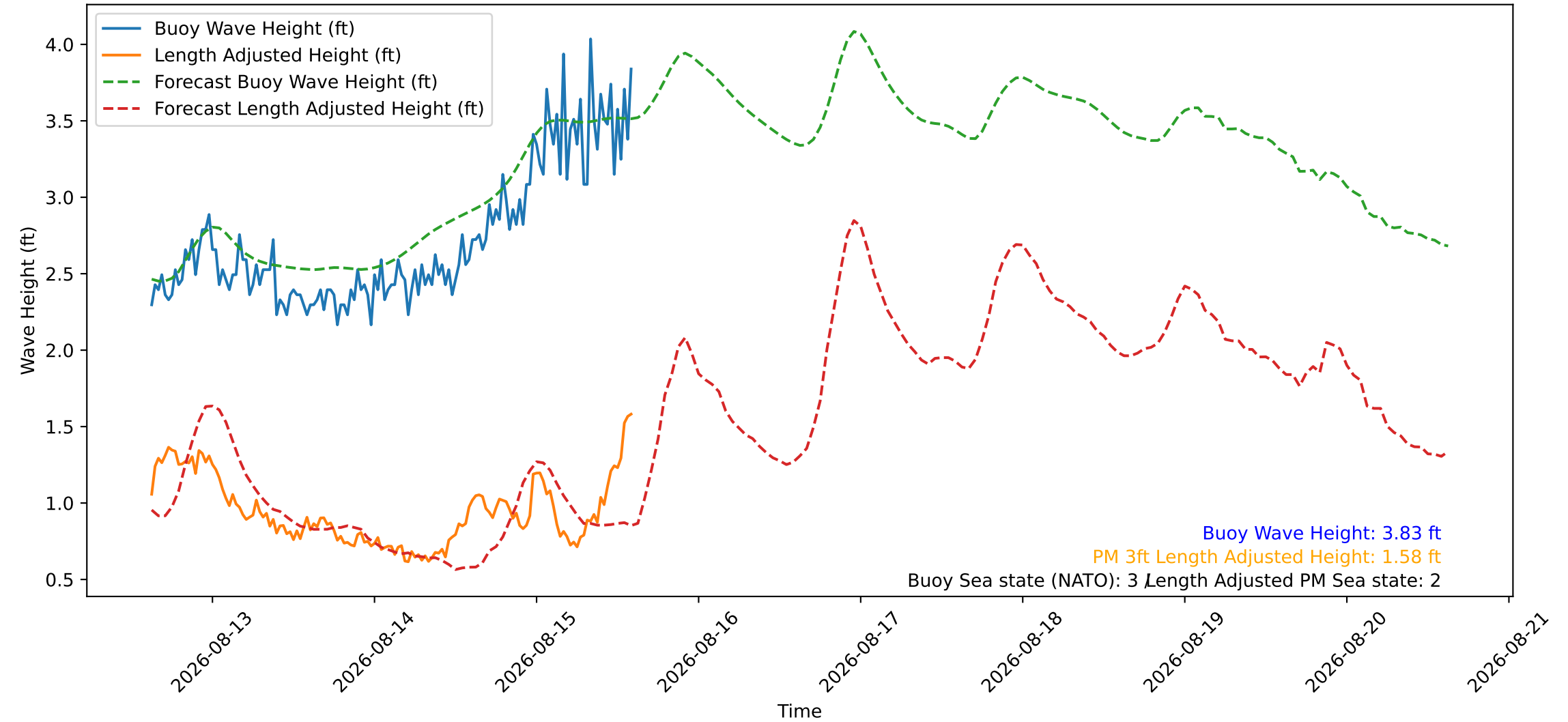
Wave Heights over Time for Red Beach at 2026-08-15 14:40:45
