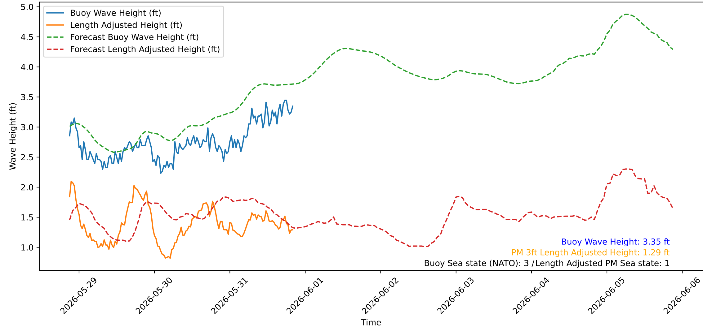
Wave Heights over Time for Red Beach at 2026-05-31 20:50:46
