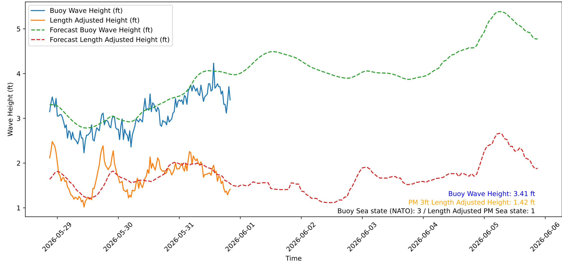
Wave Heights over Time for Oceanside Harbor at 2026-05-31 20:50:26
