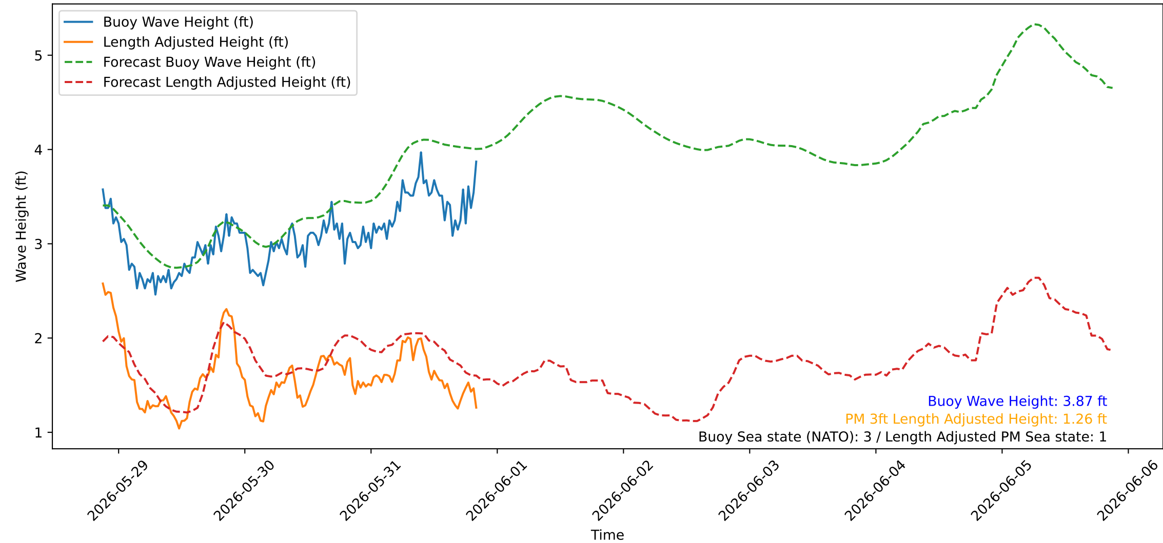
Wave Heights over Time for Green Beach at 2026-05-31 20:51:08
