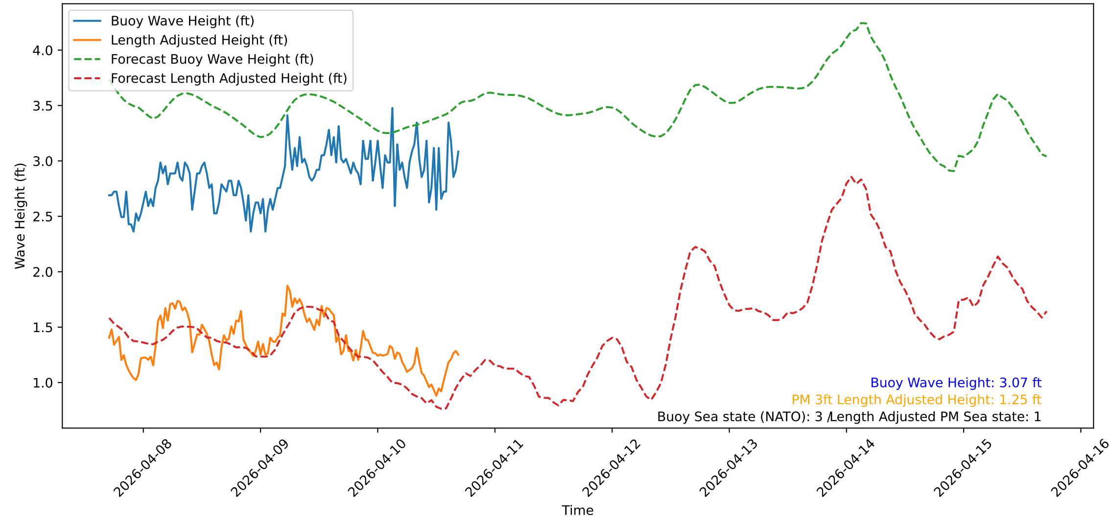
Wave Heights over Time for Green Beach at 2026-04-10 17:11:13
