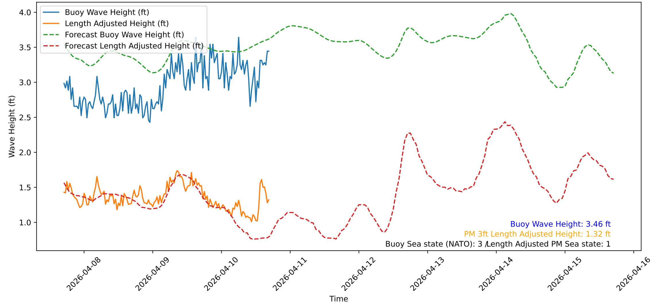
Wave Heights over Time for Oceanside Harbor at 2026-04-10 17:10:31
