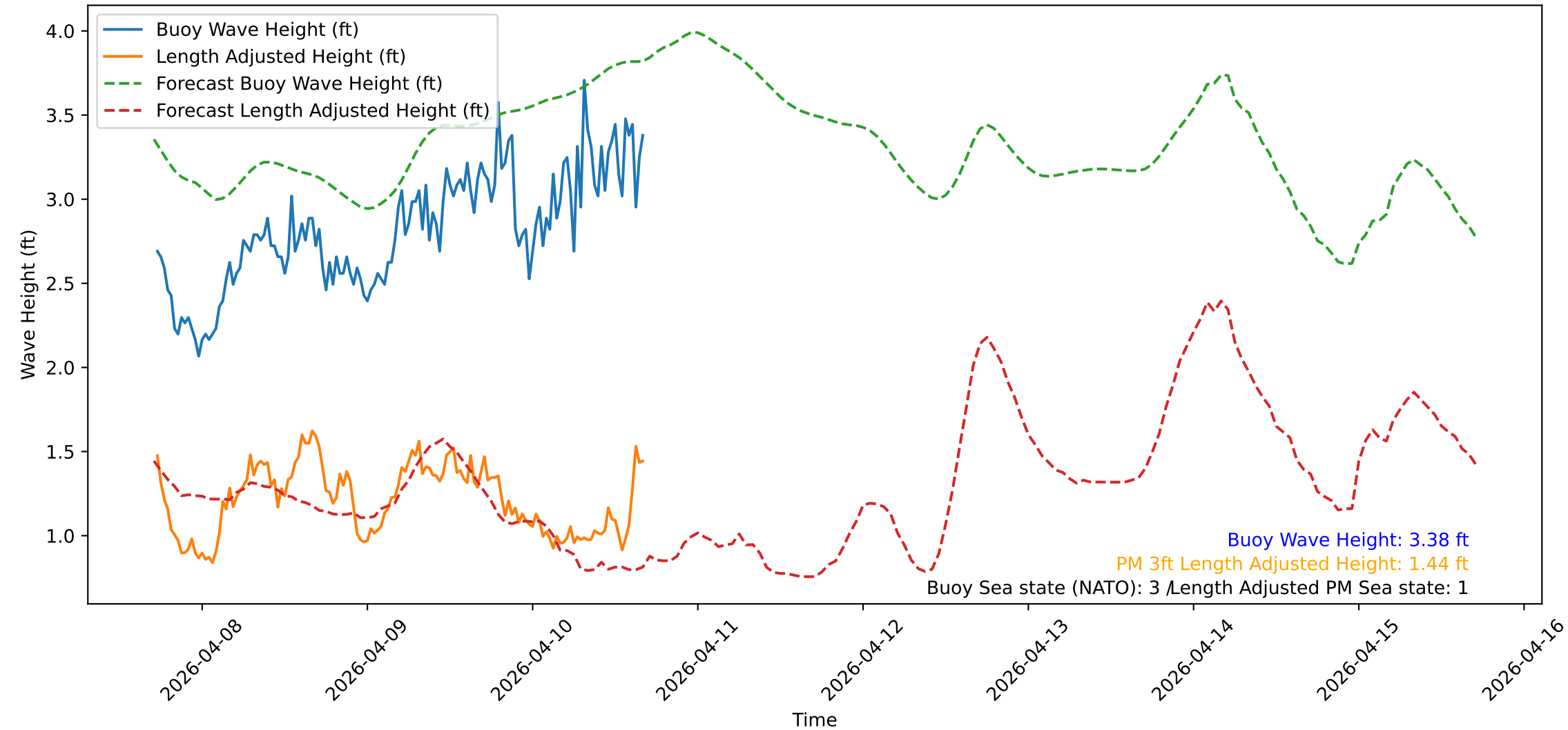
Wave Heights over Time for Red Beach at 2026-04-10 17:10:51
