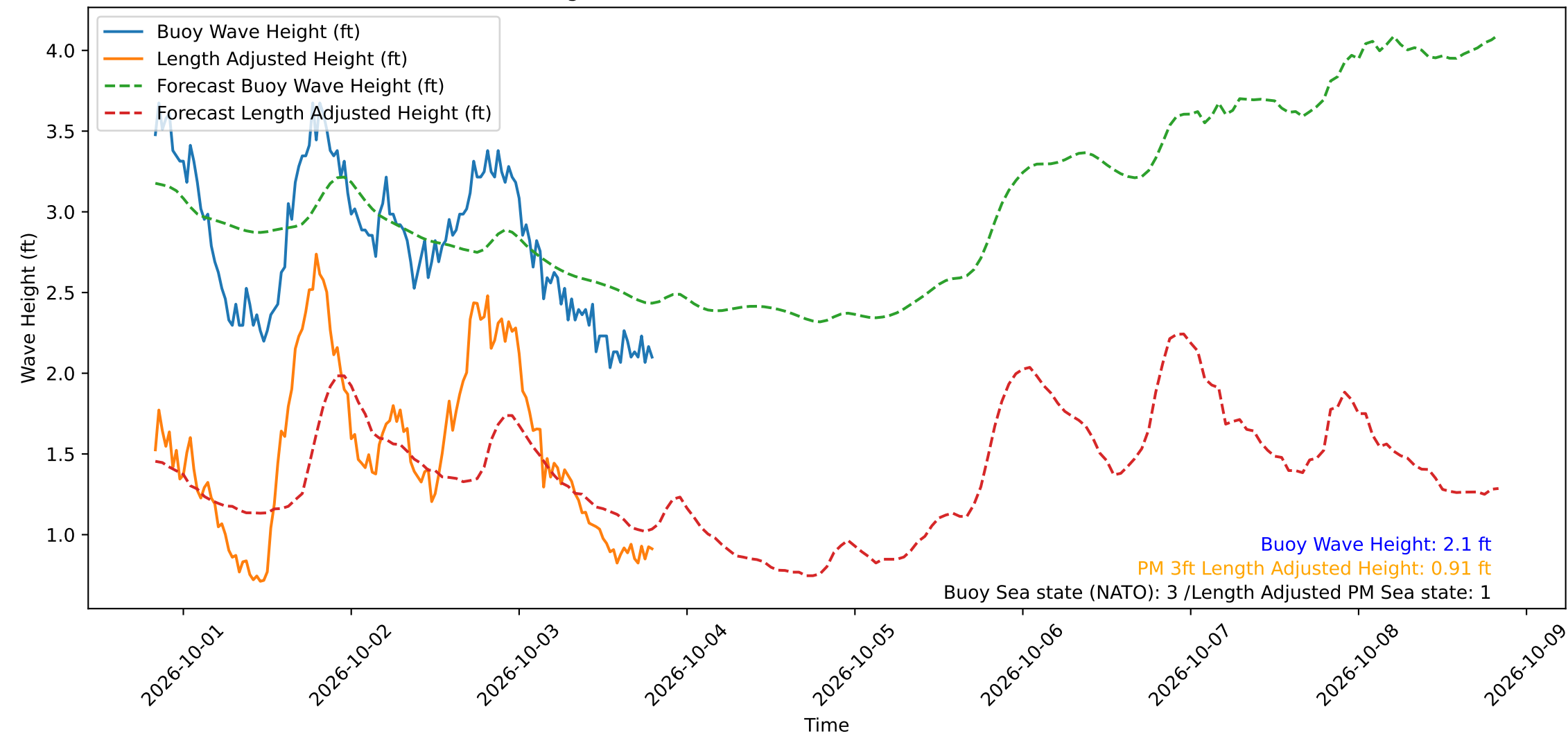
Wave Heights over Time for Green Beach at 2026-10-03 19:41:11
