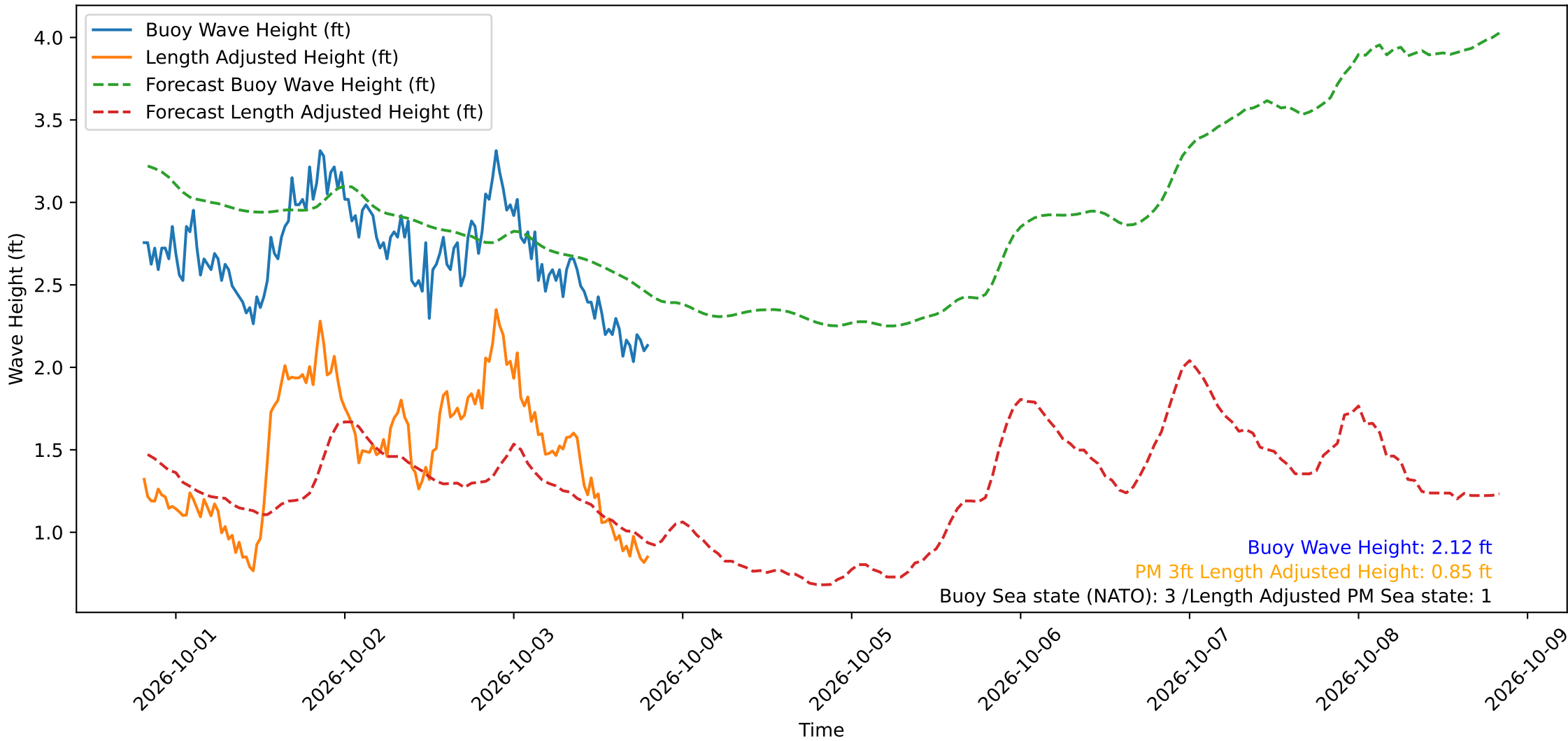
Wave Heights over Time for Oceanside Harbor at 2026-10-03 19:40:29
