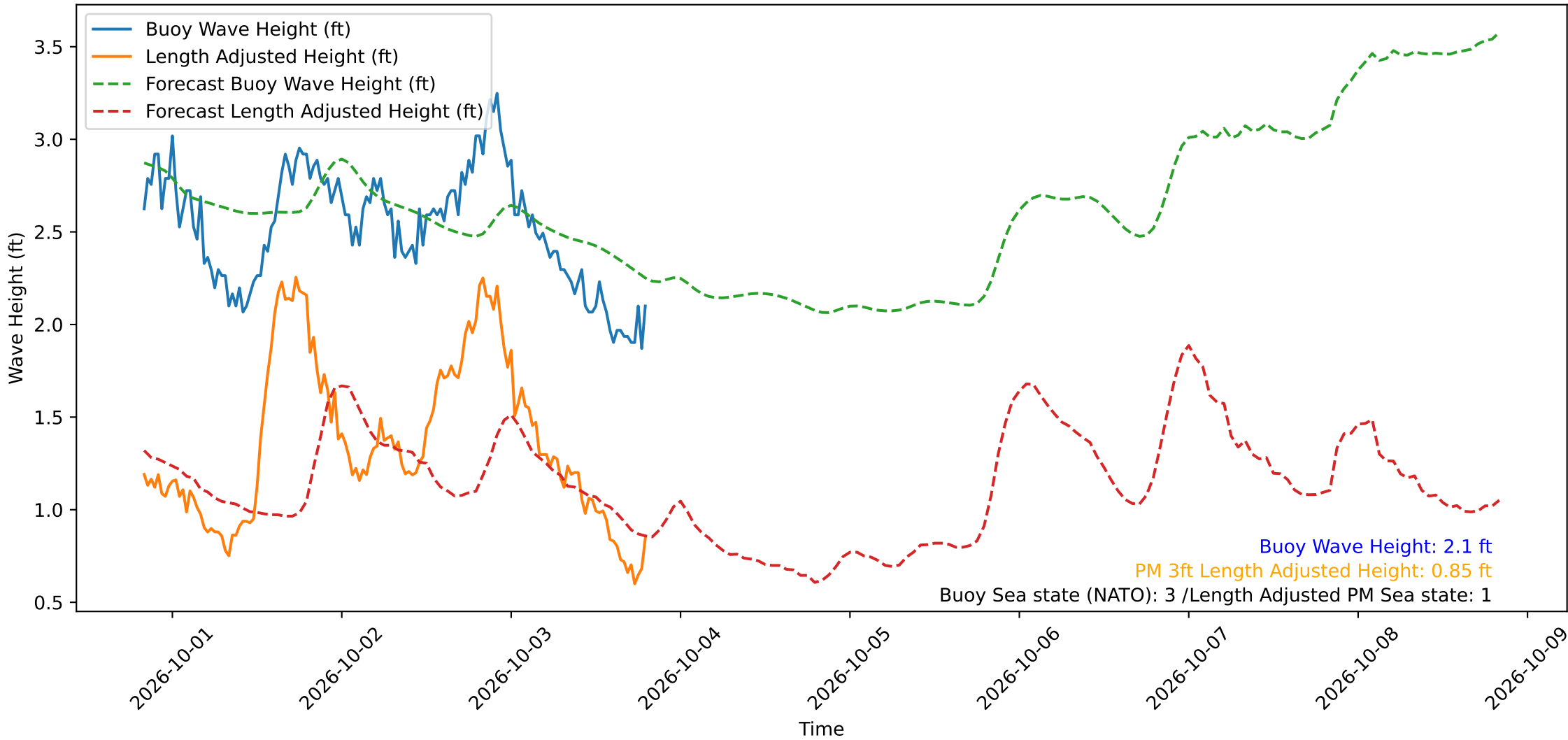
Wave Heights over Time for Red Beach at 2026-10-03 19:40:49
