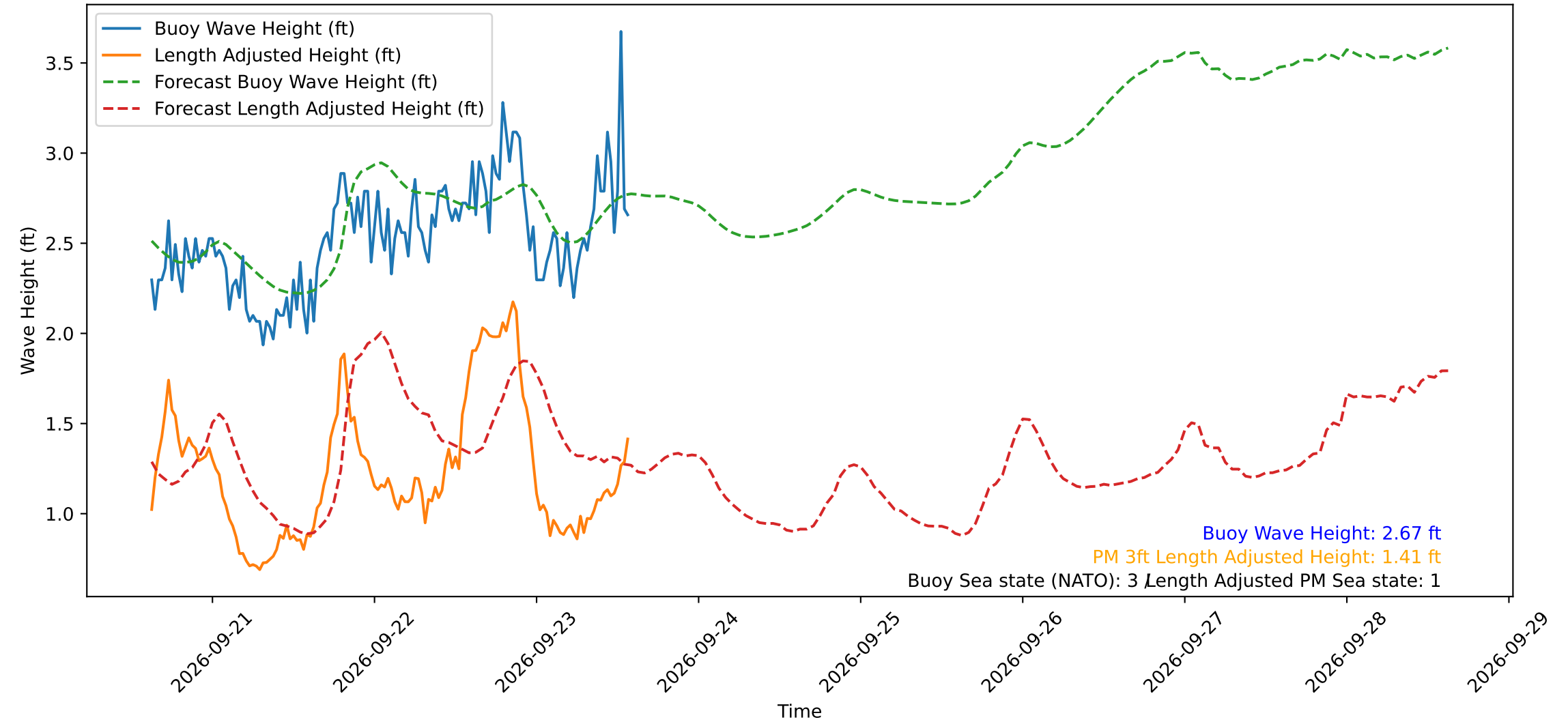
Wave Heights over Time for Red Beach at 2026-09-23 14:30:49
