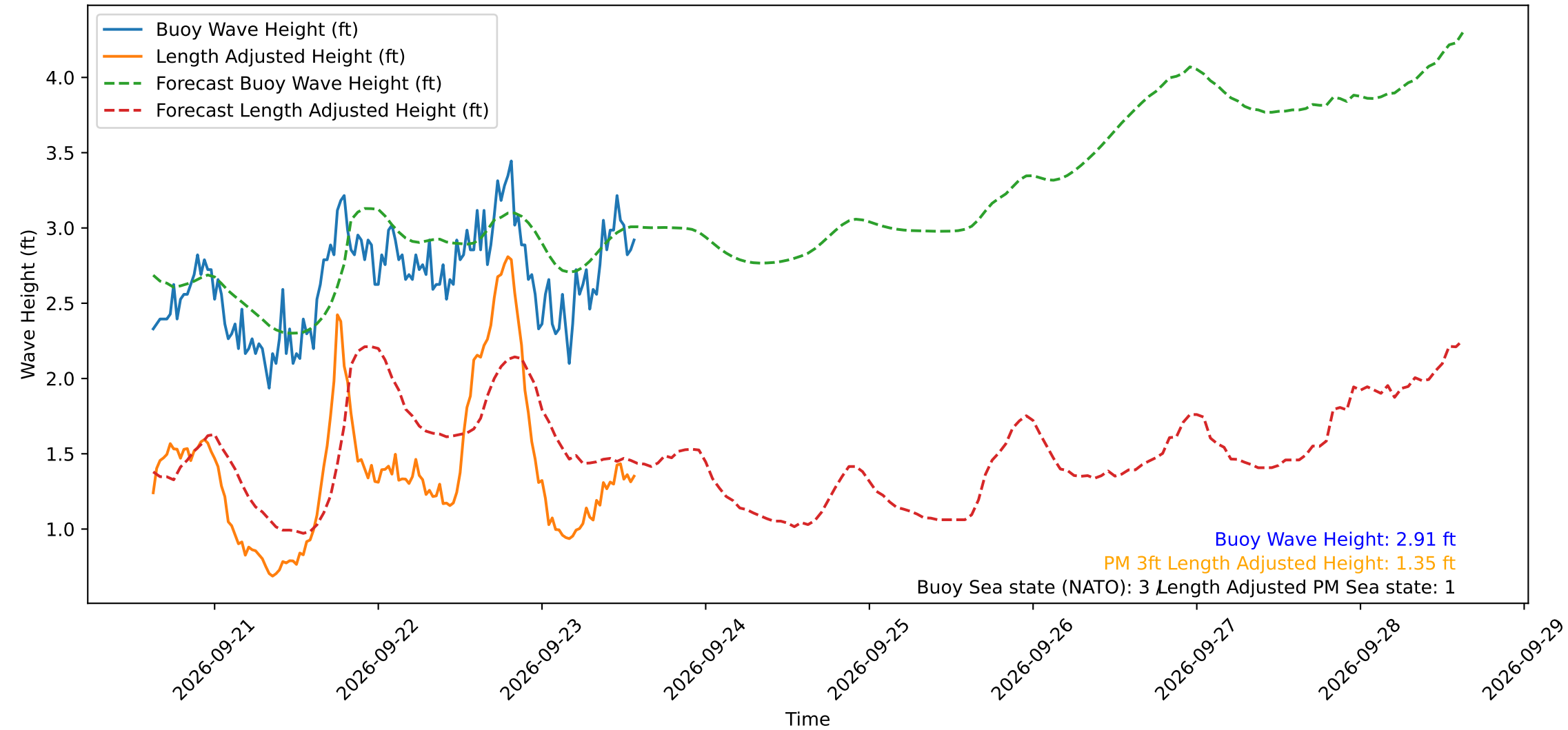
Wave Heights over Time for Green Beach at 2026-09-23 14:31:12
