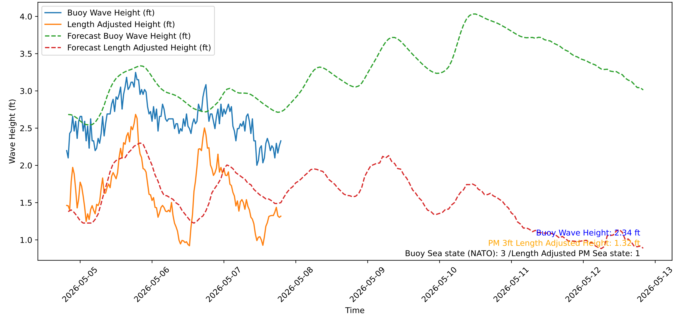
Wave Heights over Time for Oceanside Harbor at 2026-05-07 19:40:32
