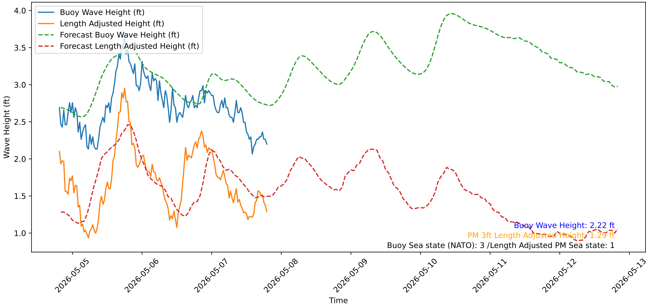
Wave Heights over Time for Green Beach at 2026-05-07 19:41:14
