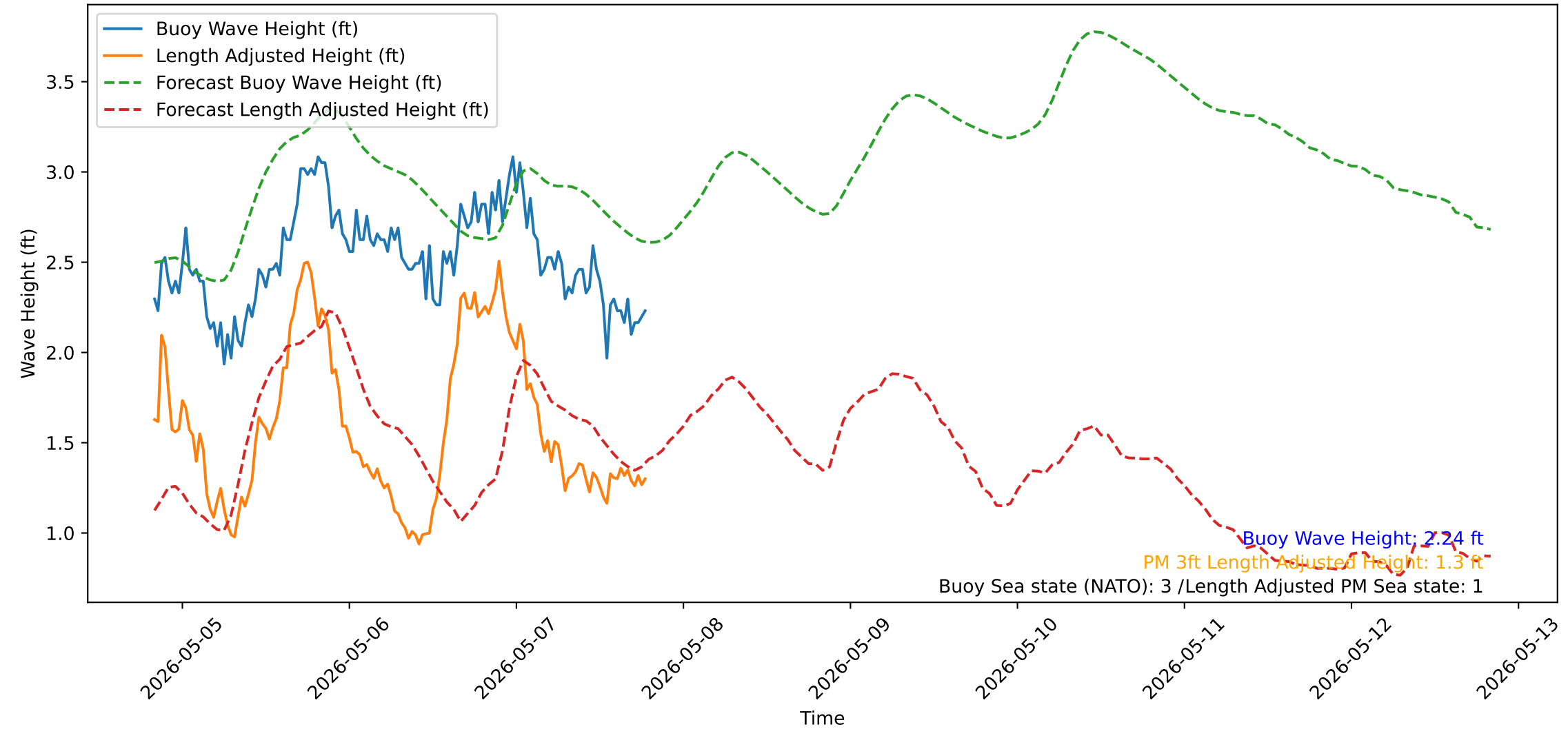
Wave Heights over Time for Red Beach at 2026-05-07 19:40:51
