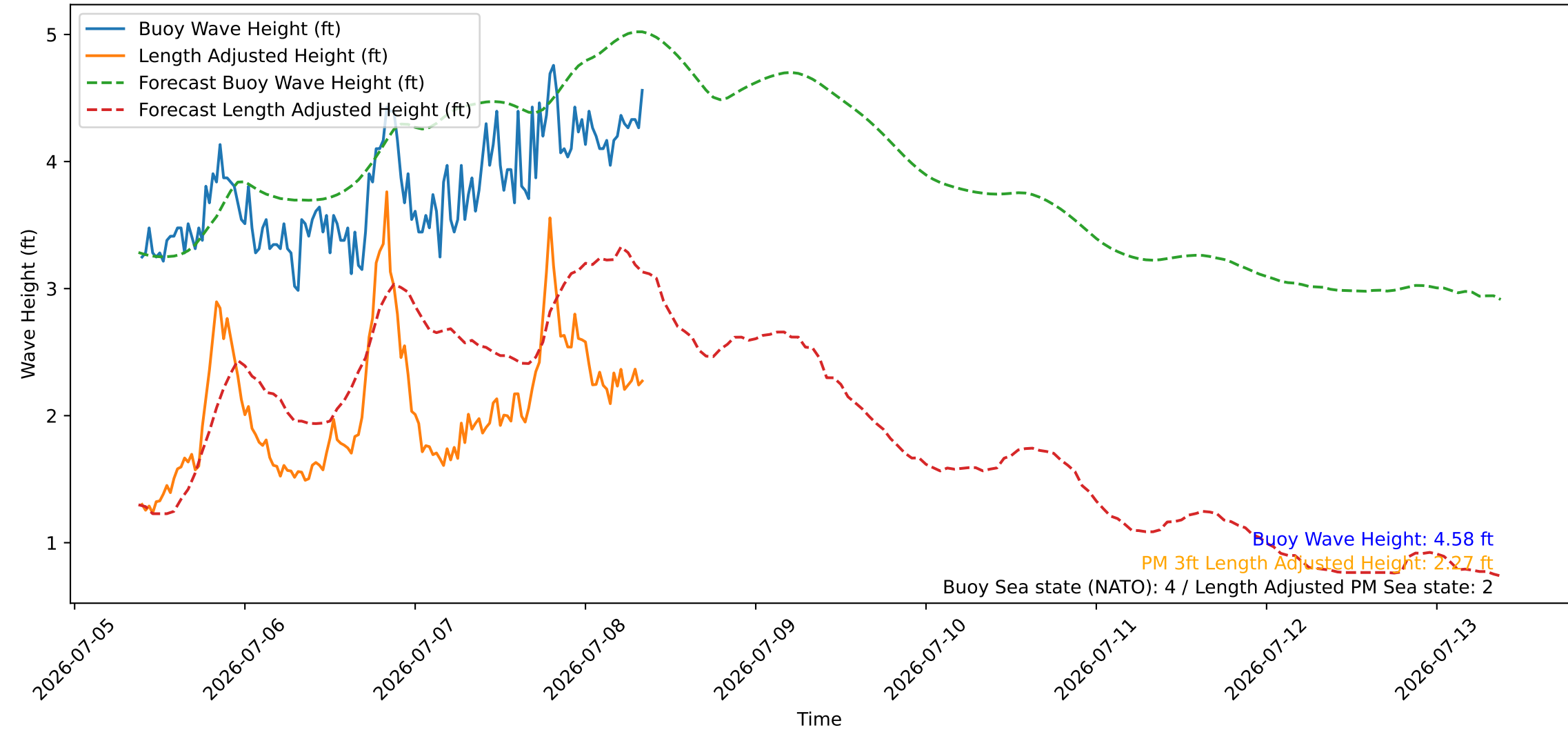
Wave Heights over Time for Green Beach at 2026-07-08 09:21:09
