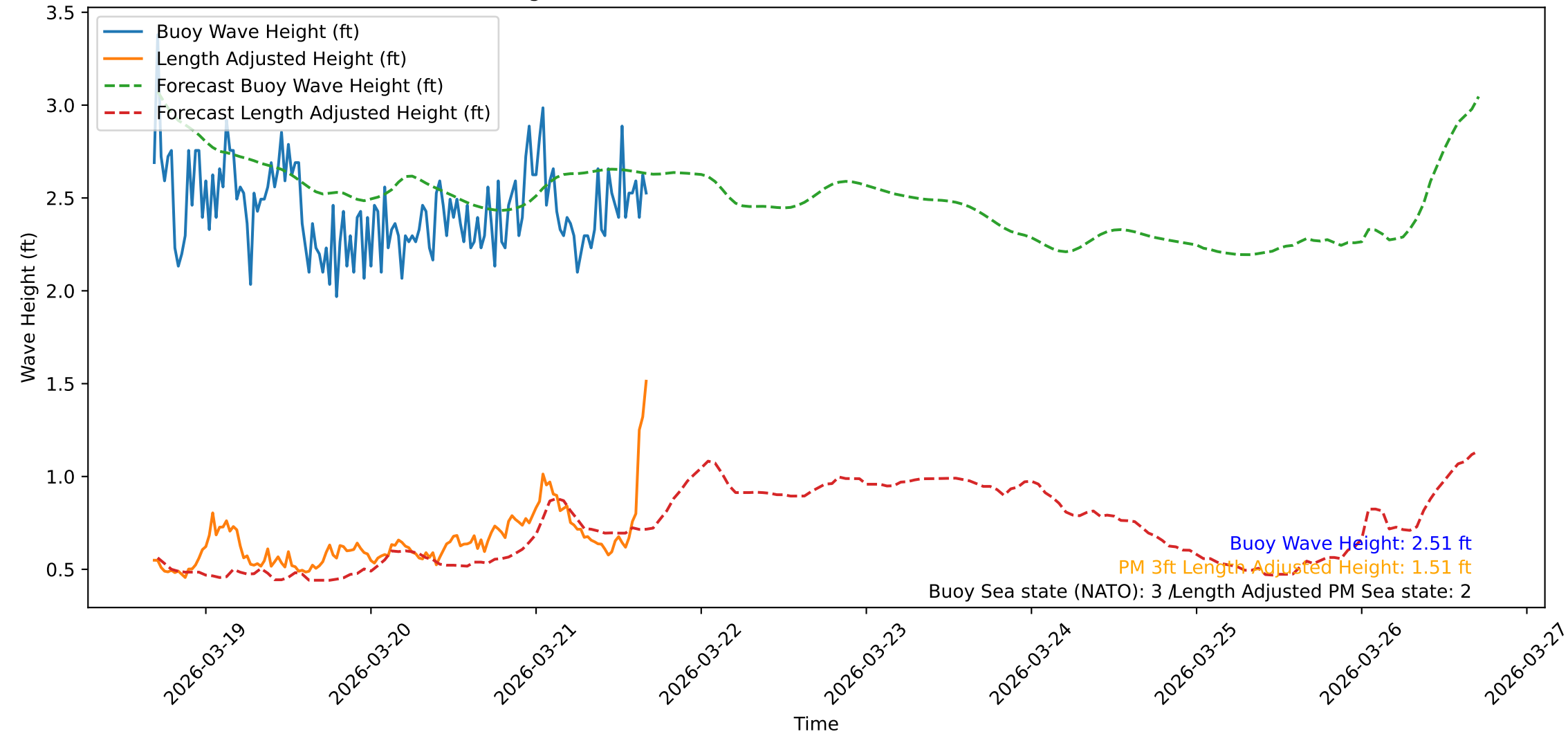
Wave Heights over Time for Oceanside Harbor at 2026-03-21 16:40:31
