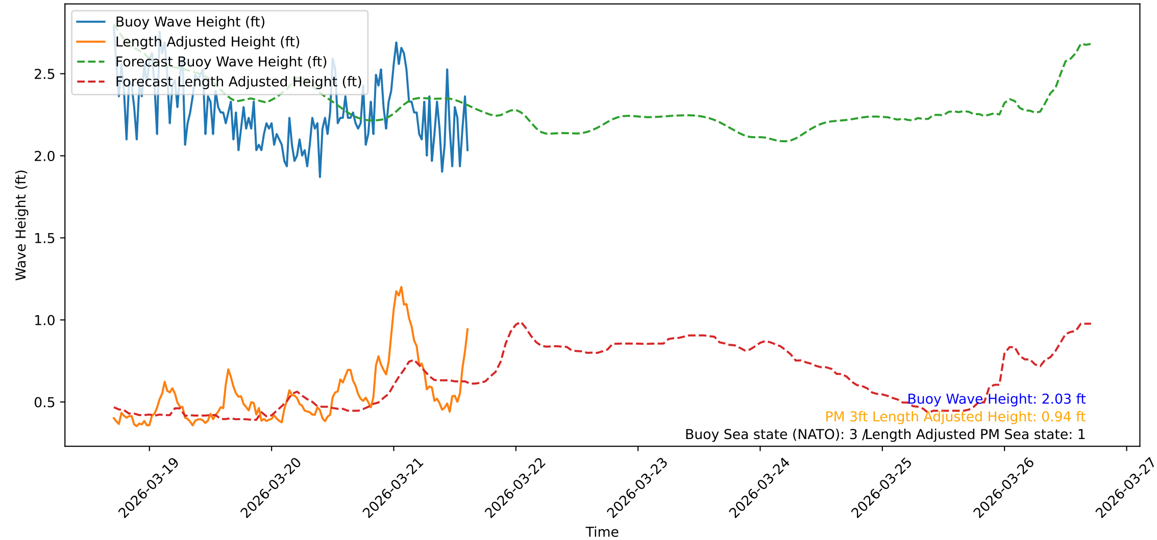
Wave Heights over Time for Red Beach at 2026-03-21 16:40:47
