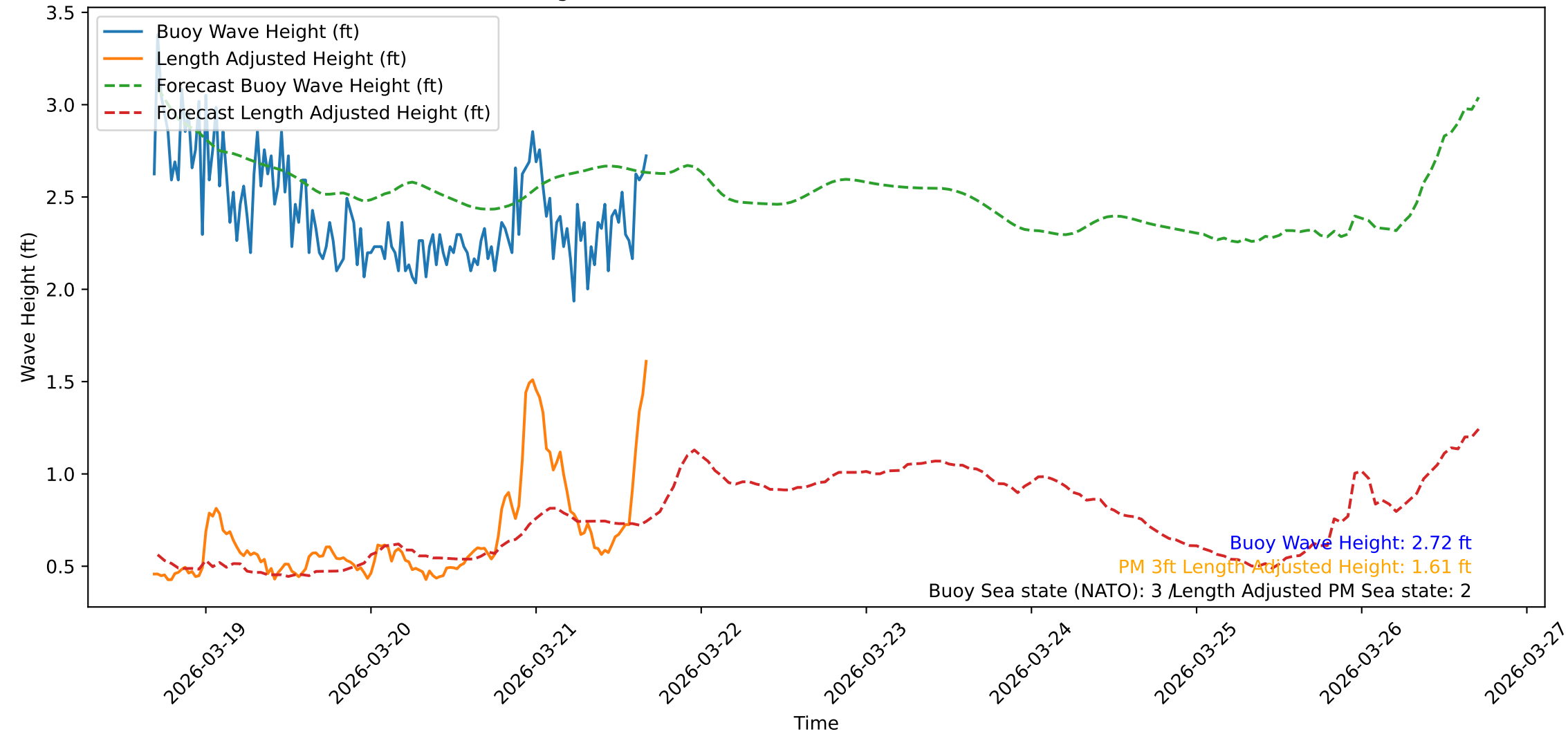
Wave Heights over Time for Green Beach at 2026-03-21 16:41:10
