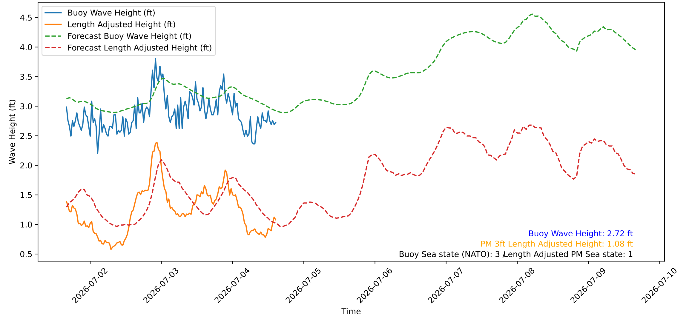
Wave Heights over Time for Red Beach at 2026-07-04 15:40:45
