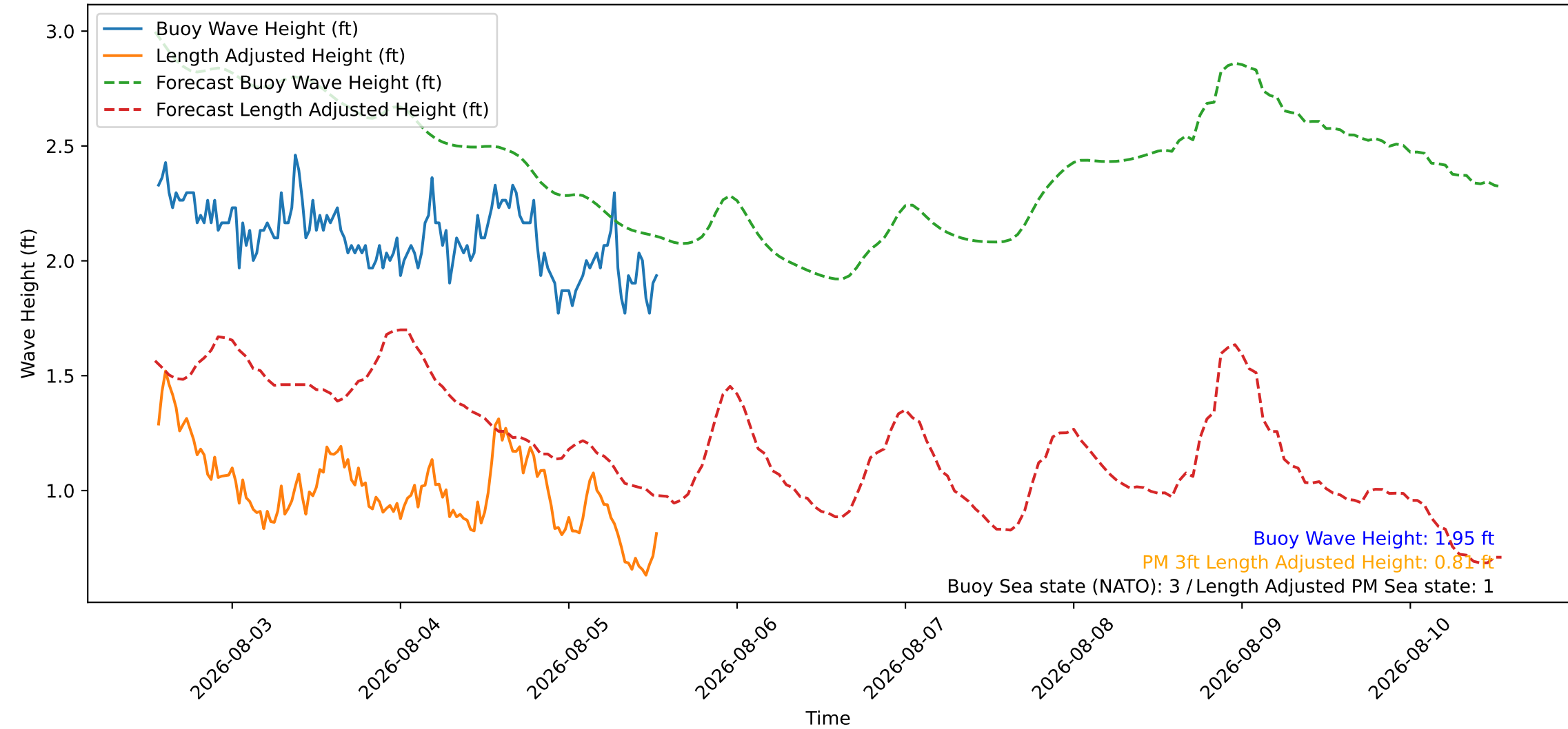
Wave Heights over Time for Red Beach at 2026-08-05 13:20:46
