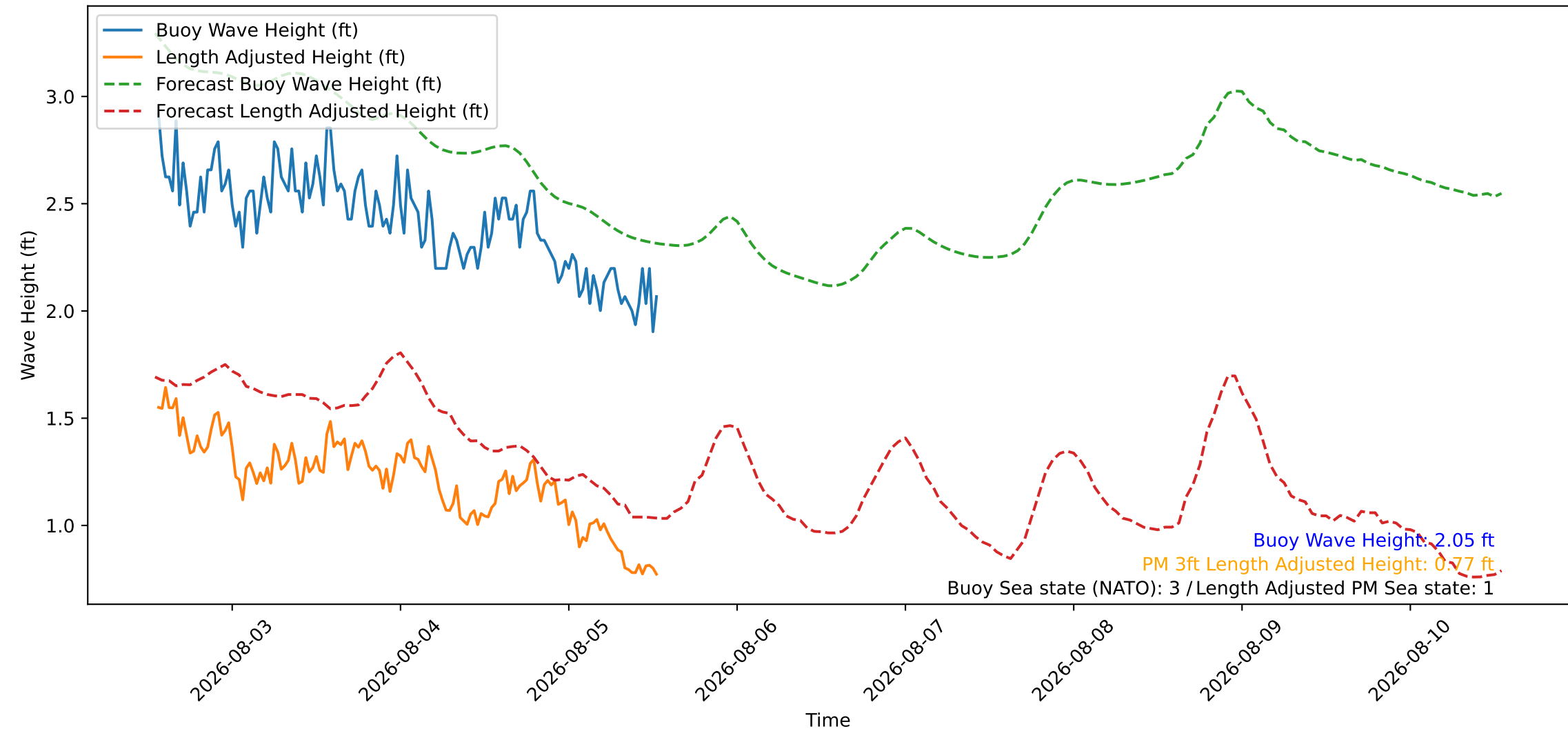
Wave Heights over Time for Oceanside Harbor at 2026-08-05 13:20:26
