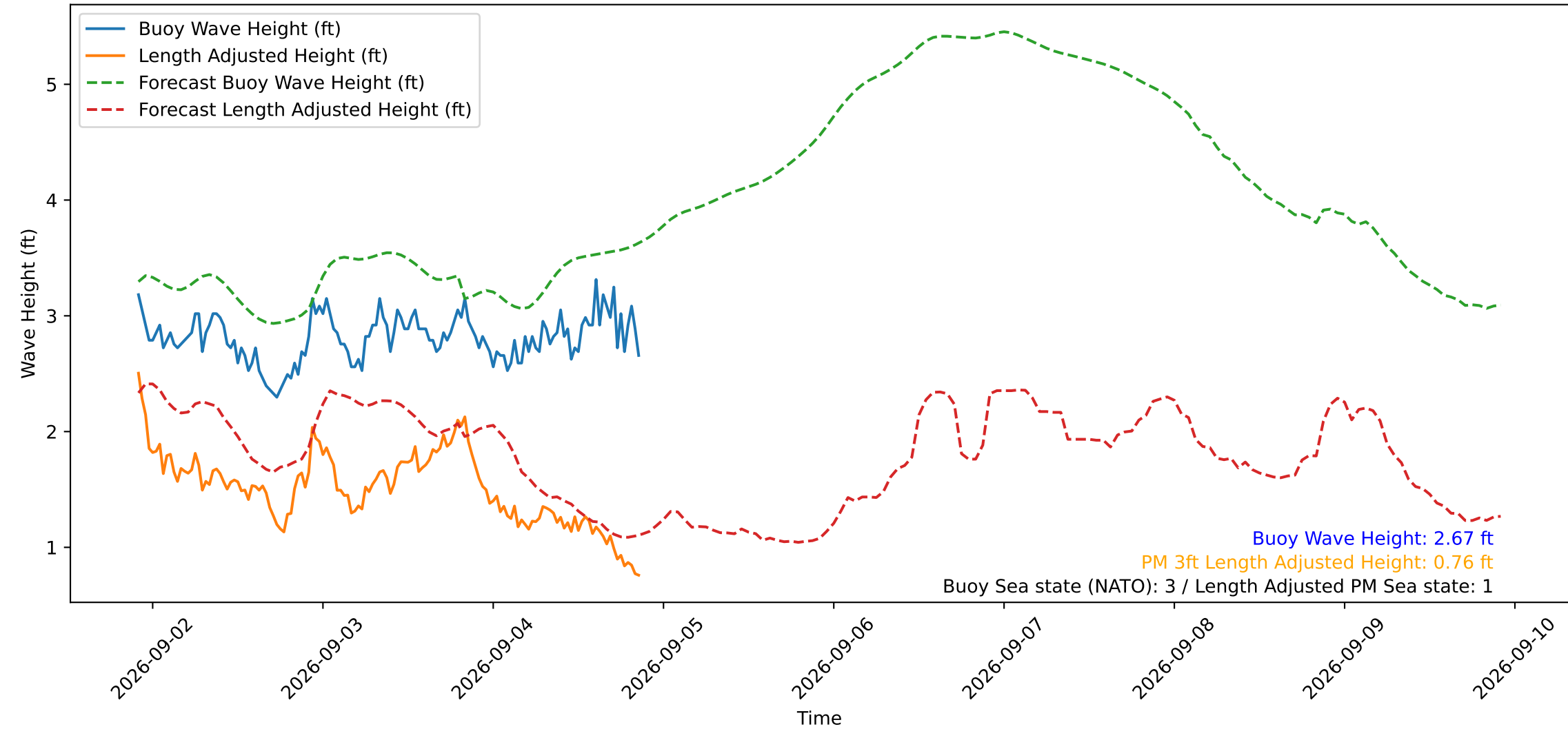
Wave Heights over Time for Red Beach at 2026-09-04 21:30:49
