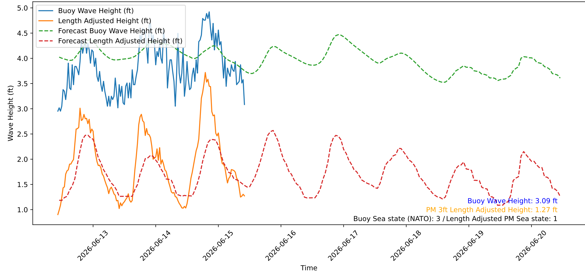
Wave Heights over Time for Green Beach at 2026-06-15 10:41:09
