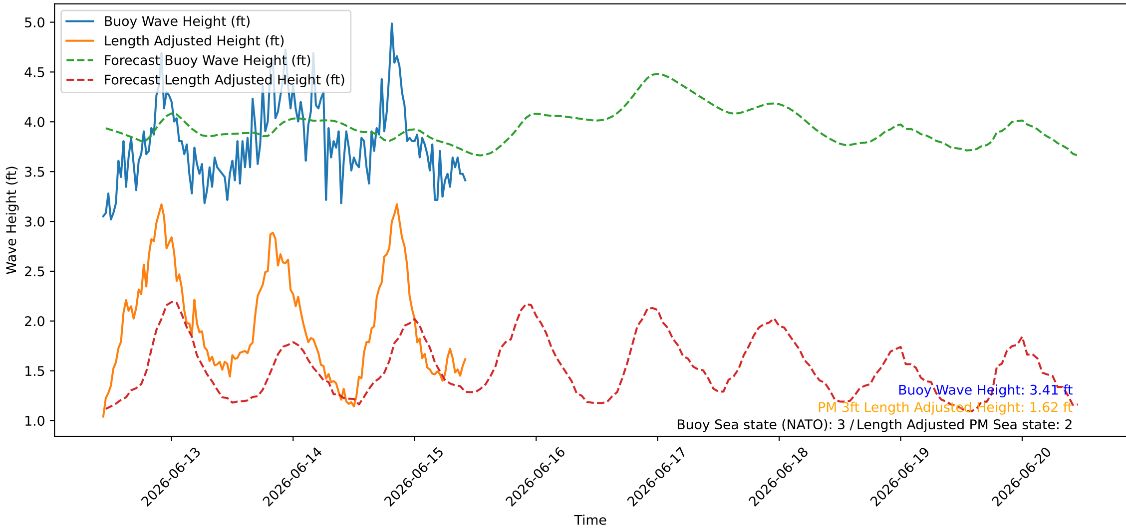
Wave Heights over Time for Oceanside Harbor at 2026-06-15 10:40:26
