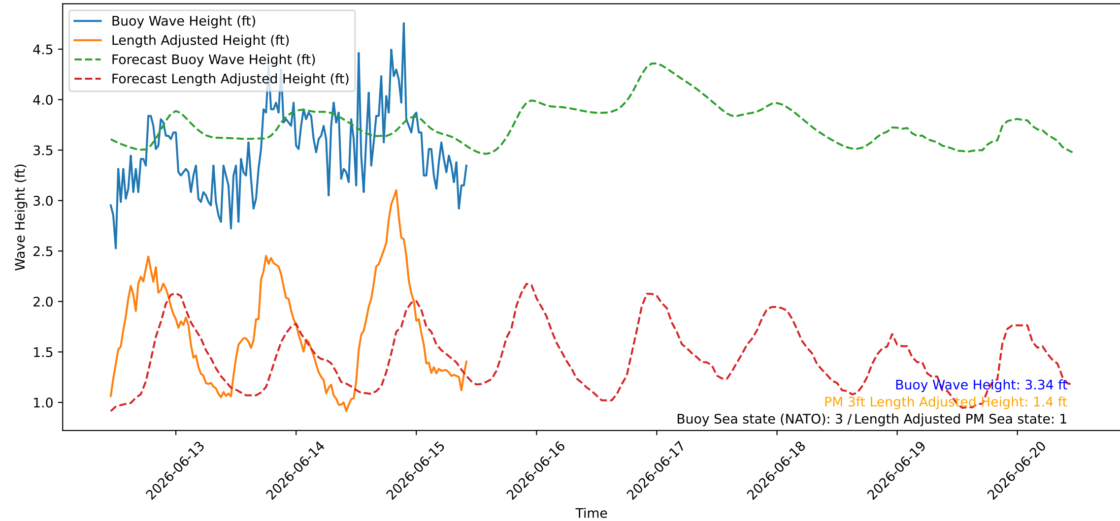
Wave Heights over Time for Red Beach at 2026-06-15 10:40:46
