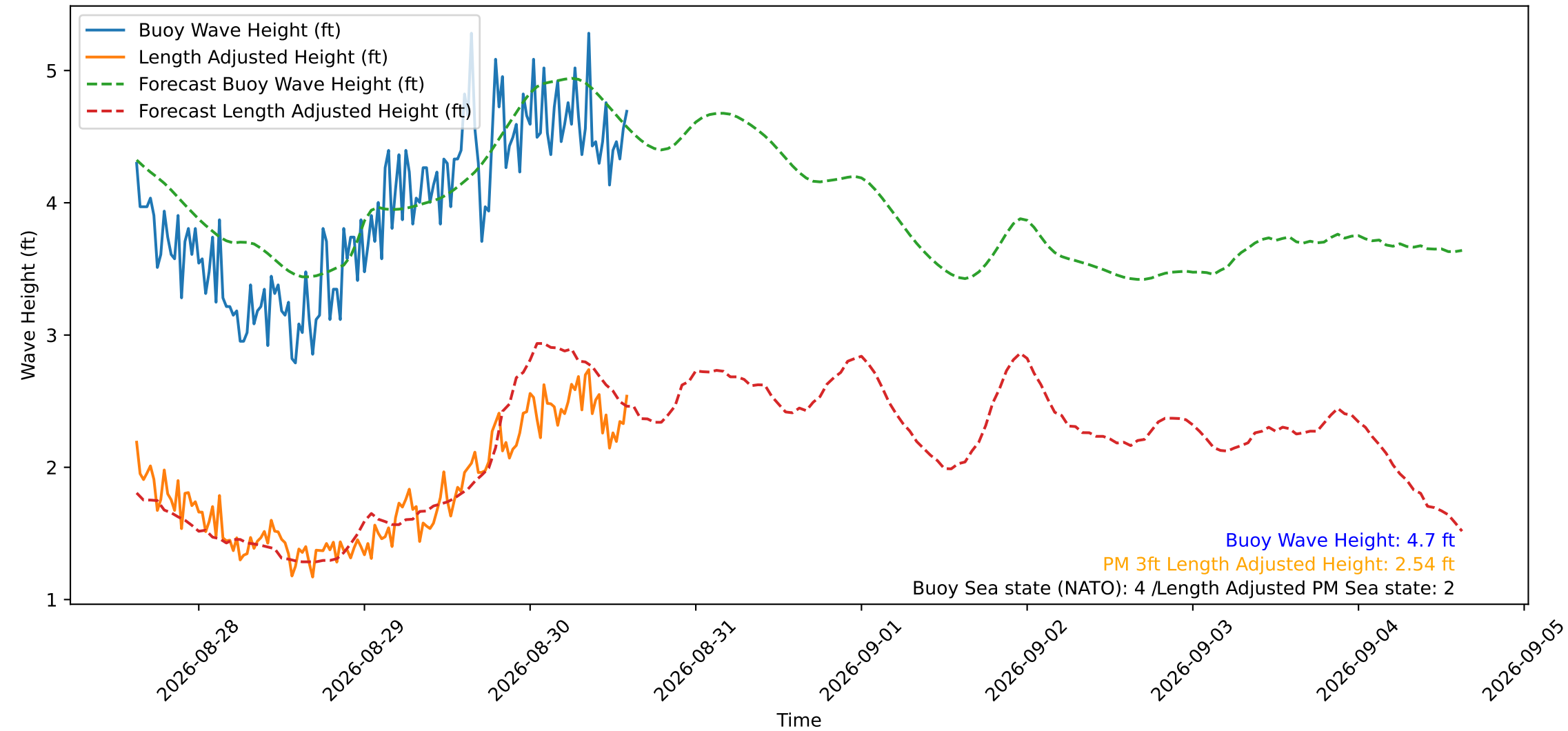
Wave Heights over Time for Oceanside Harbor at 2026-08-30 14:50:30
