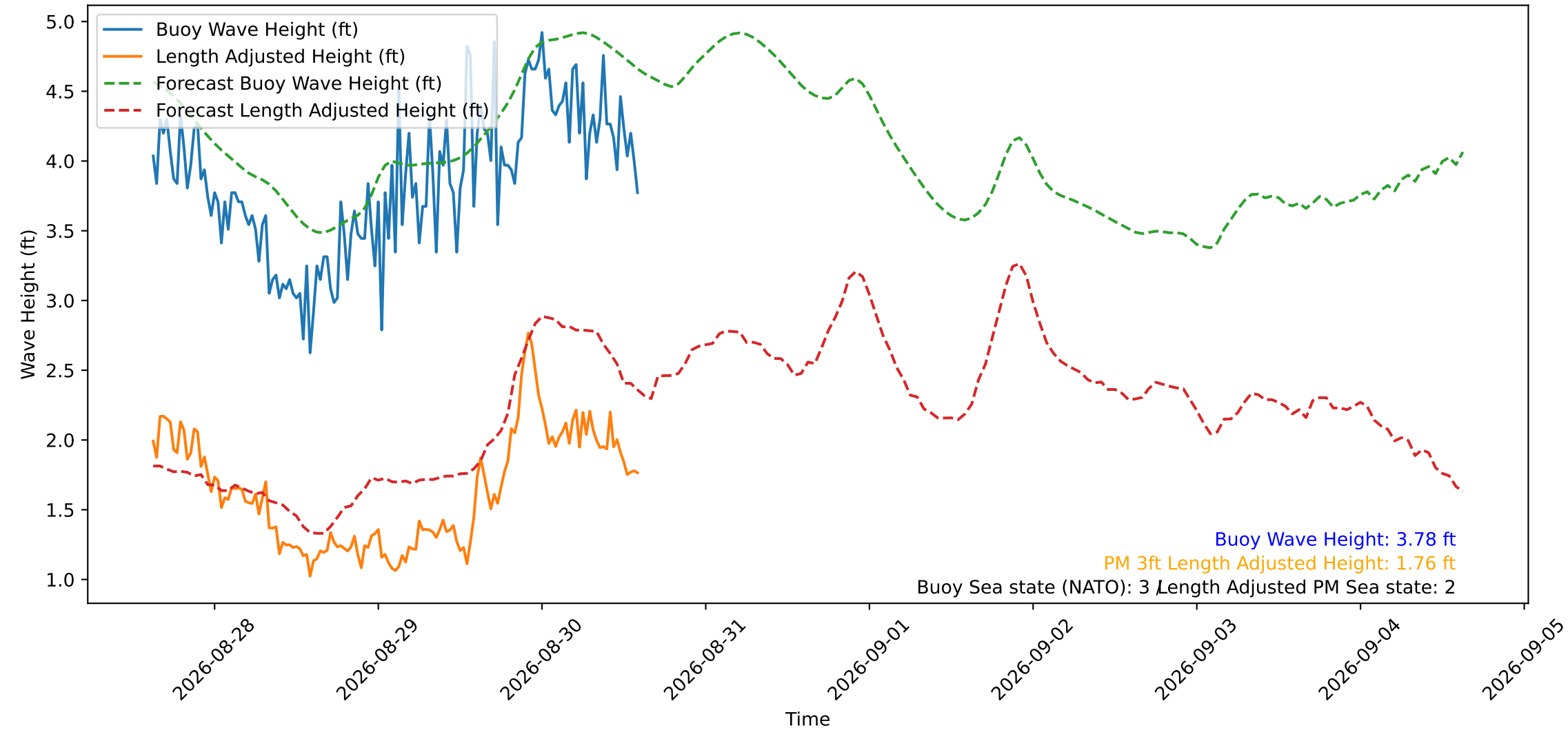
Wave Heights over Time for Green Beach at 2026-08-30 14:51:15
