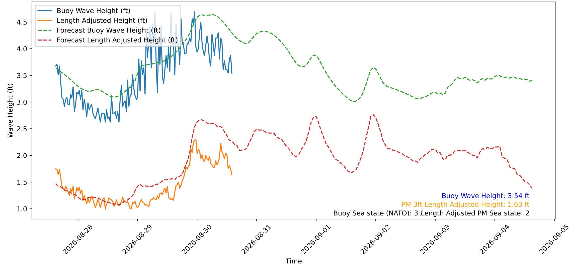
Wave Heights over Time for Red Beach at 2026-08-30 14:50:51
