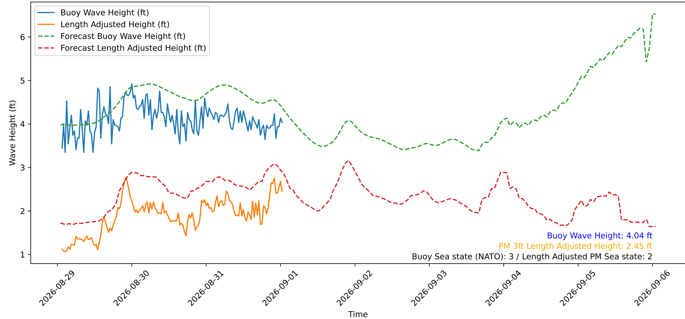
Wave Heights over Time for Green Beach at 2026-09-01 01:21:14
