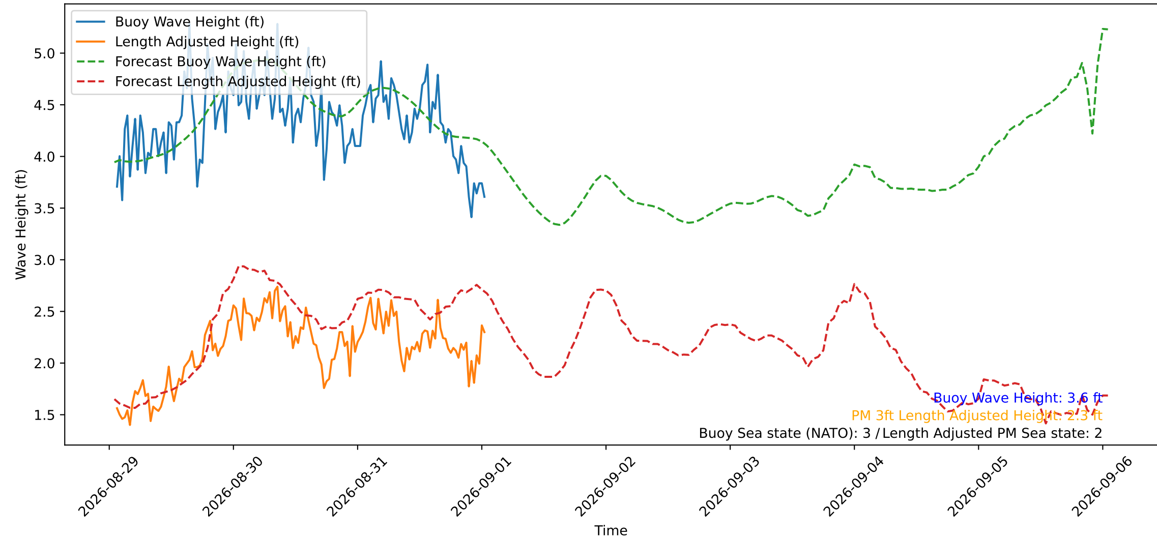
Wave Heights over Time for Oceanside Harbor at 2026-09-01 01:20:29
