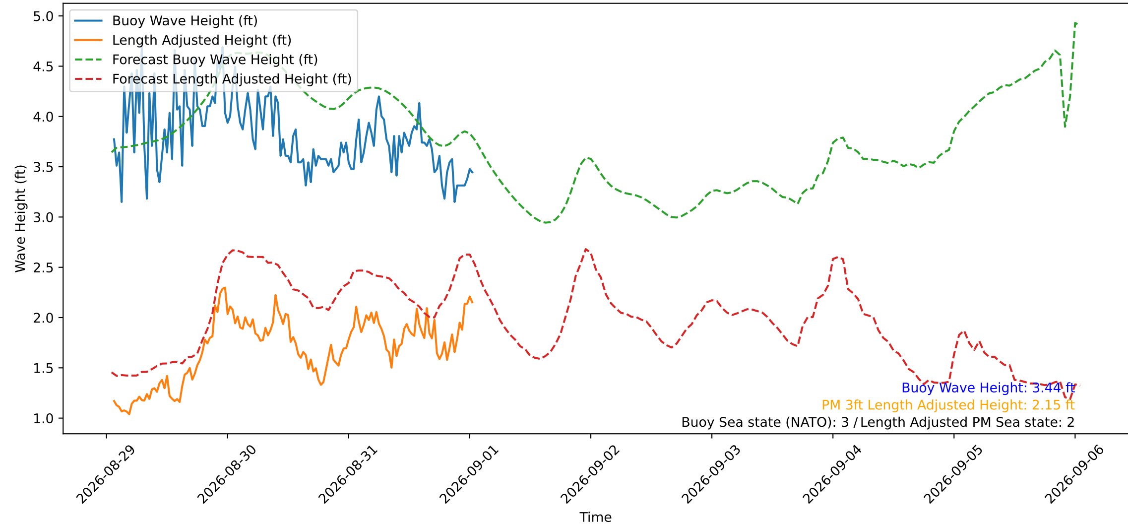
Wave Heights over Time for Red Beach at 2026-09-01 01:20:50
