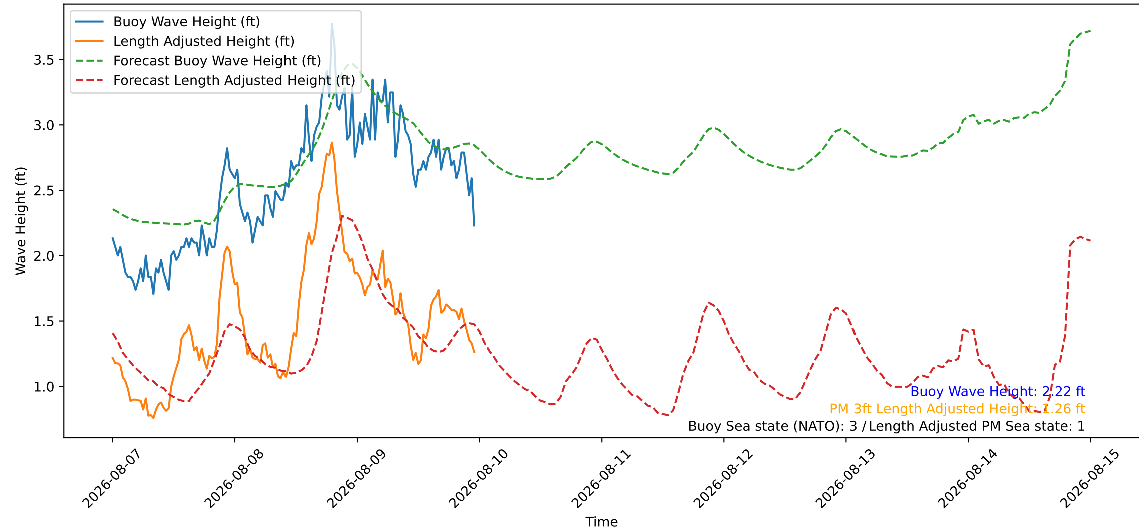
Wave Heights over Time for Green Beach at 2026-08-09 23:51:09
