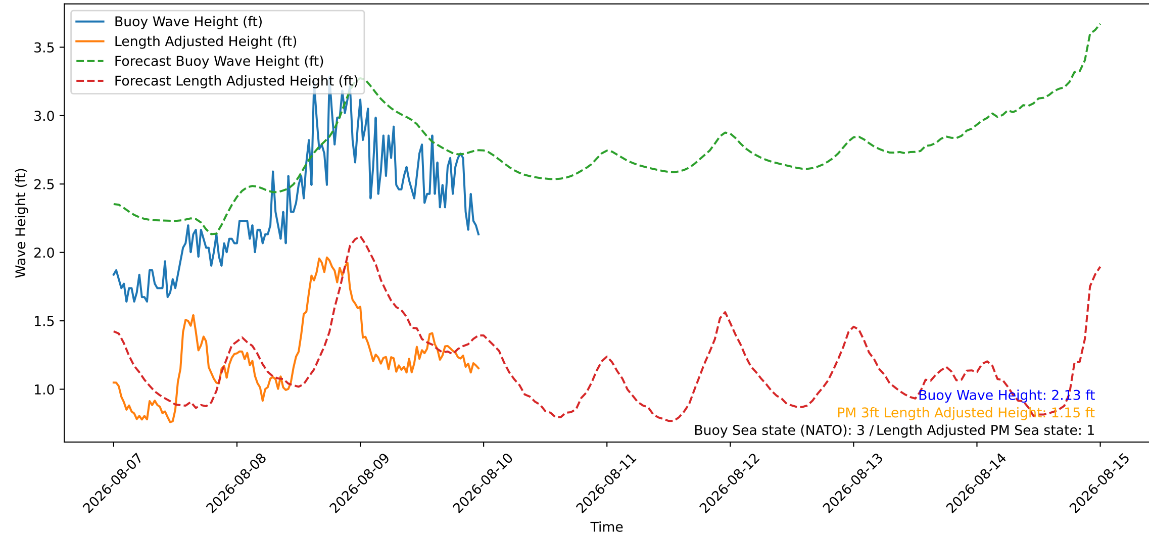
Wave Heights over Time for Oceanside Harbor at 2026-08-09 23:50:26
