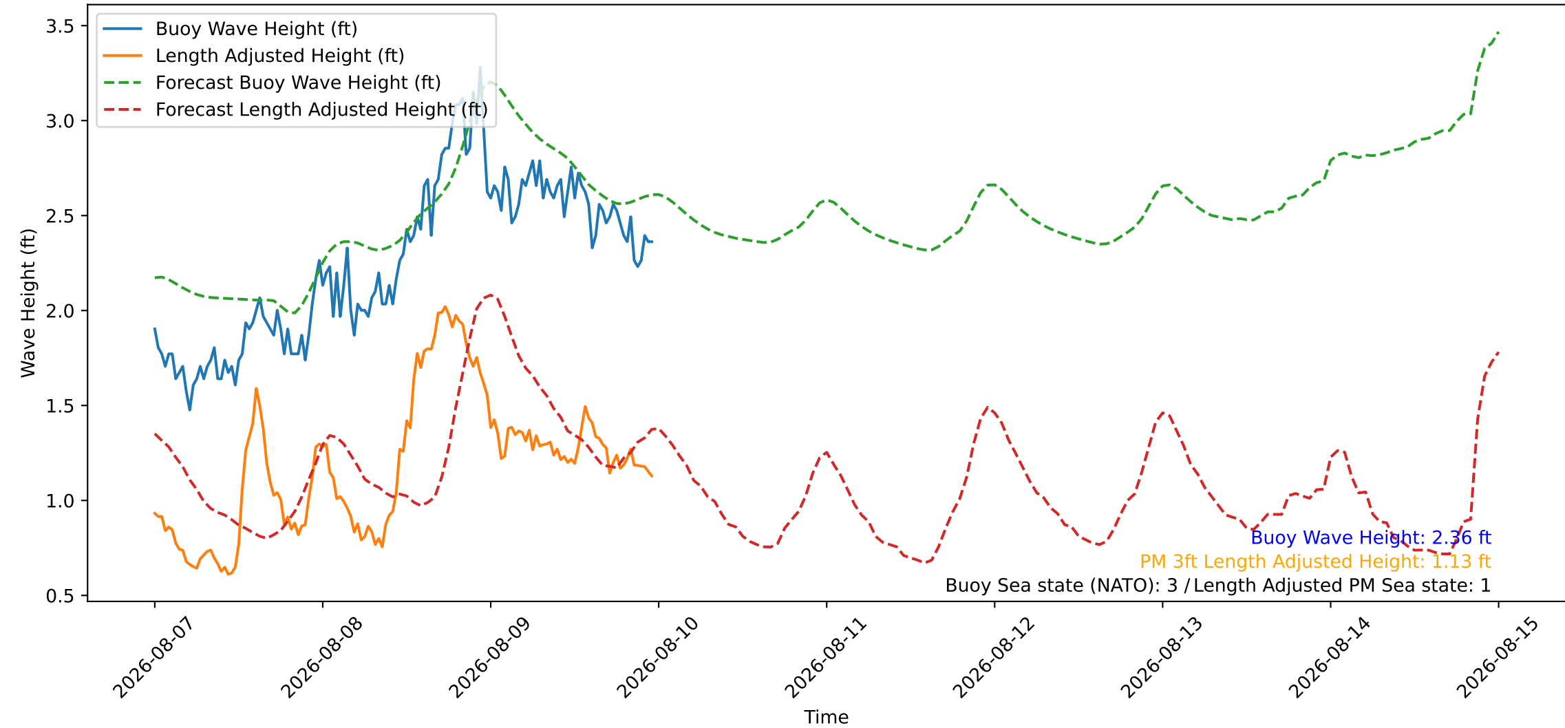
Wave Heights over Time for Red Beach at 2026-08-09 23:50:47
