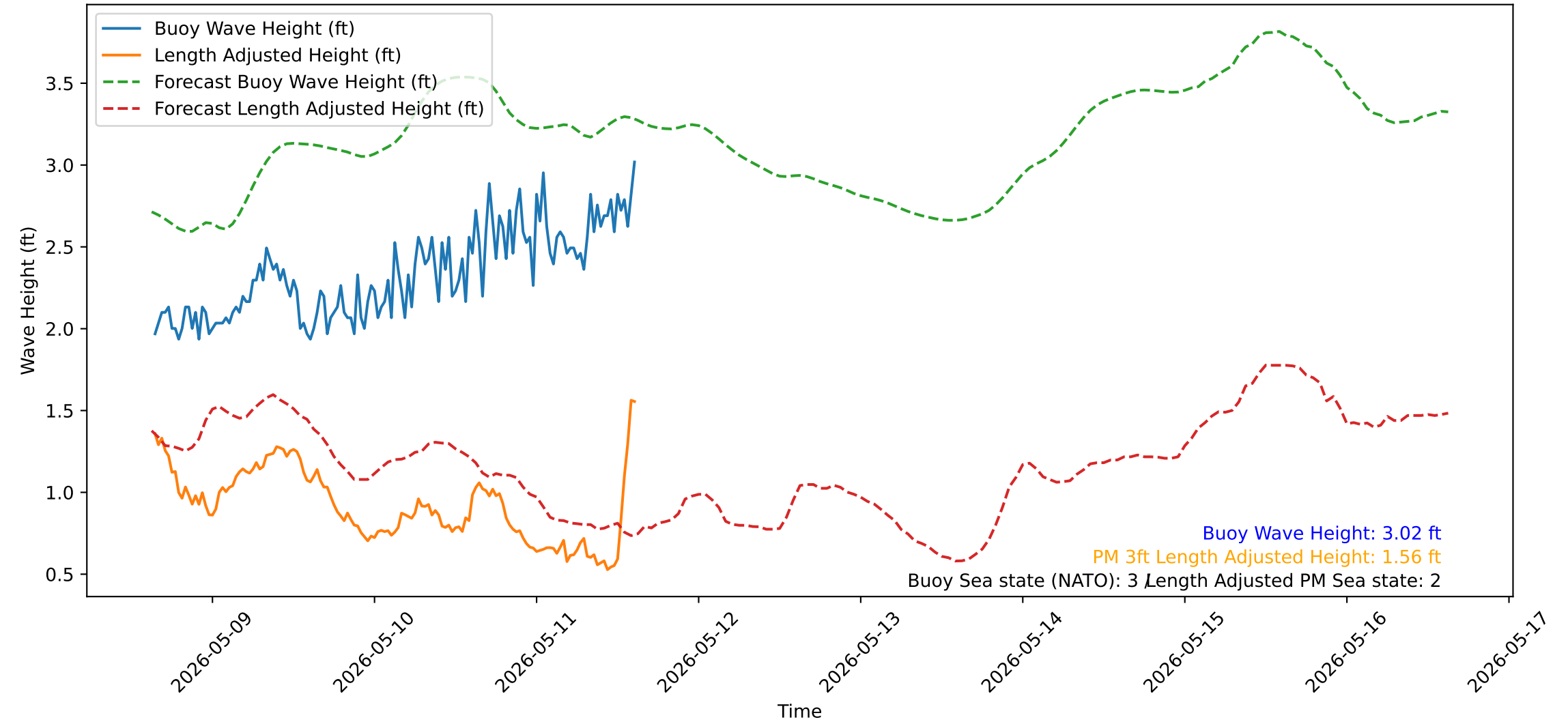
Wave Heights over Time for Red Beach at 2026-05-11 15:10:50
