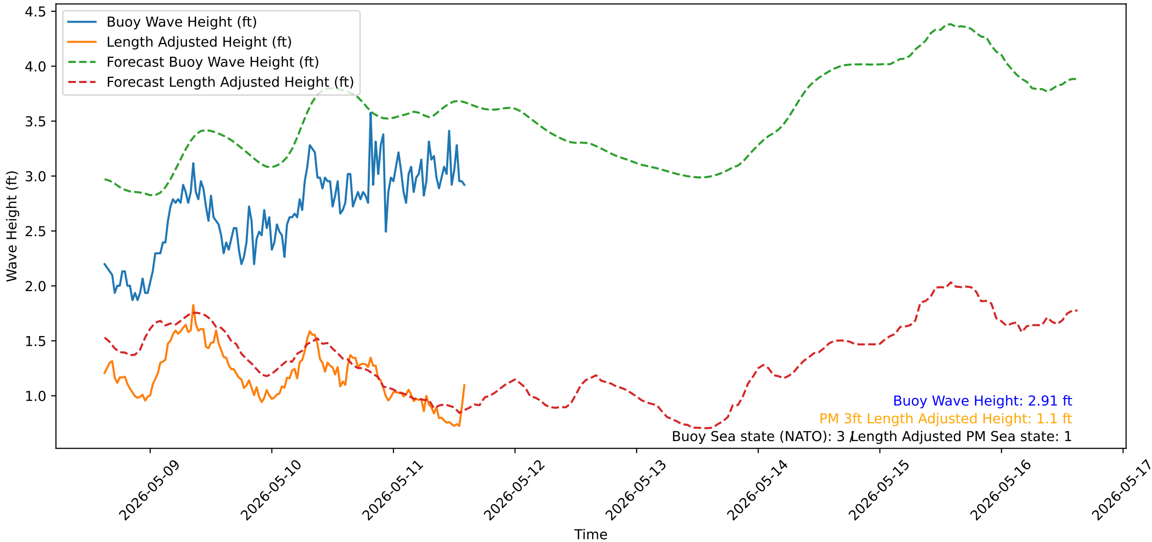
Wave Heights over Time for Oceanside Harbor at 2026-05-11 15:10:31
