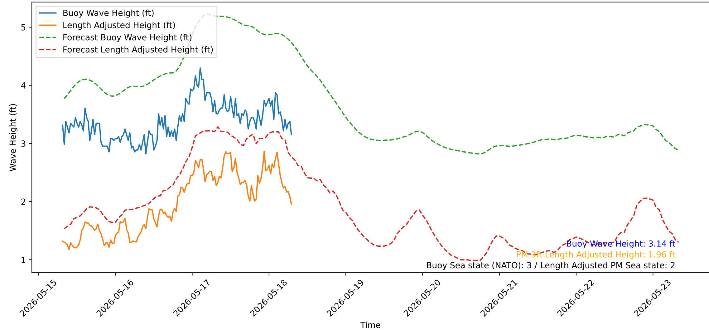
Wave Heights over Time for Oceanside Harbor at 2026-05-18 07:40:32
