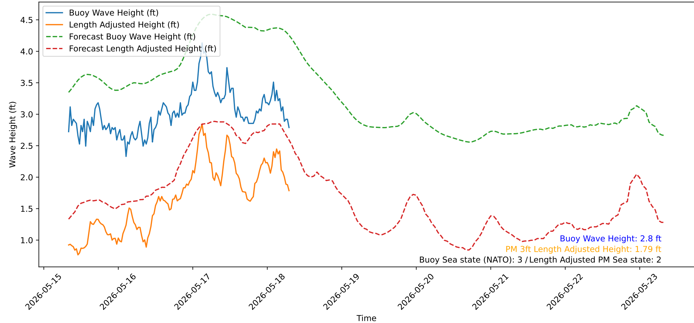
Wave Heights over Time for Red Beach at 2026-05-18 07:40:52
