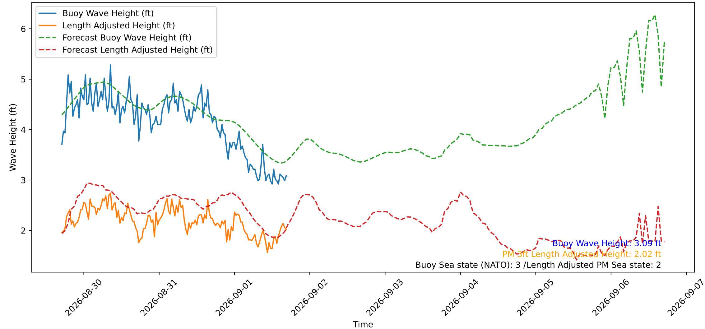
Wave Heights over Time for Oceanside Harbor at 2026-09-01 17:10:30
