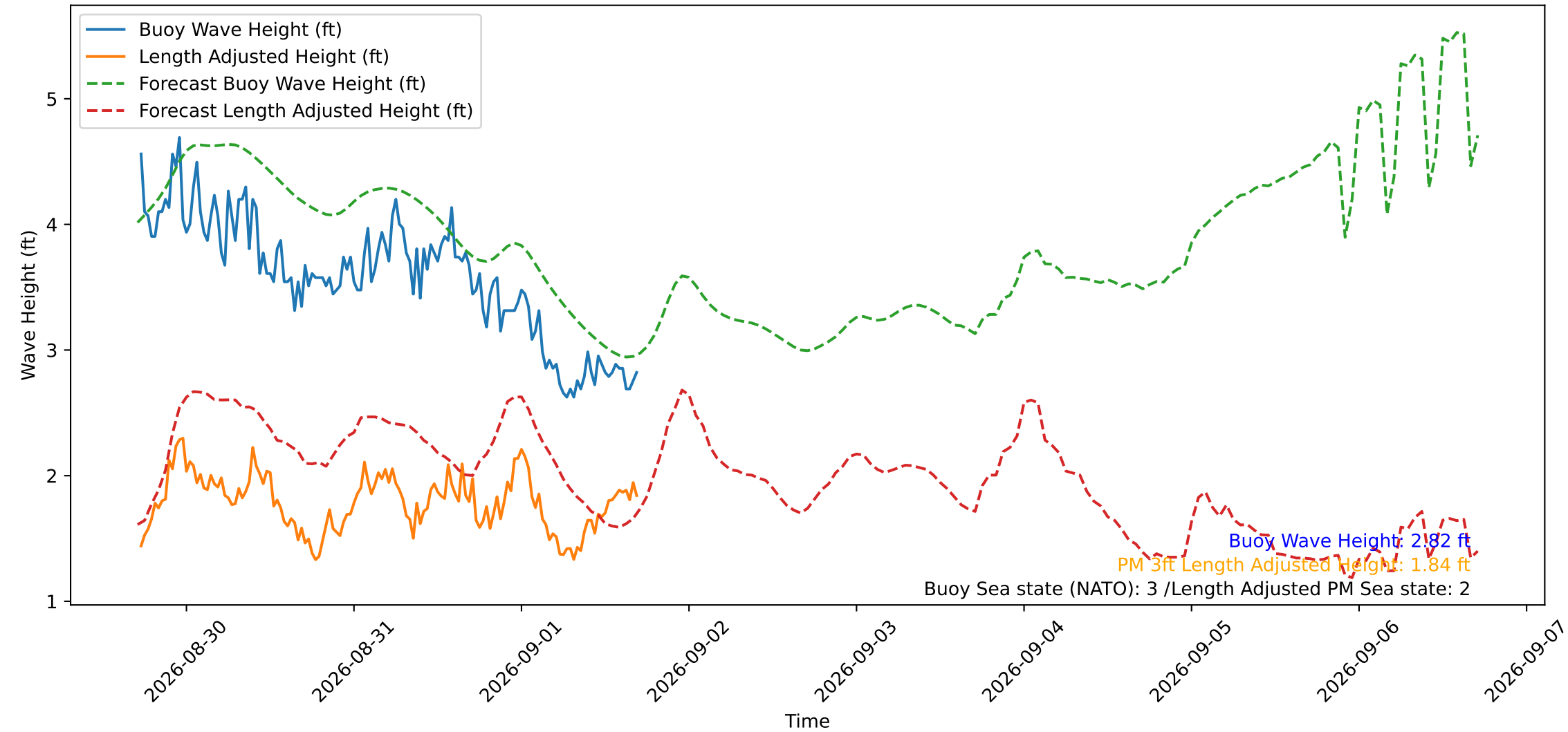
Wave Heights over Time for Red Beach at 2026-09-01 17:10:50
