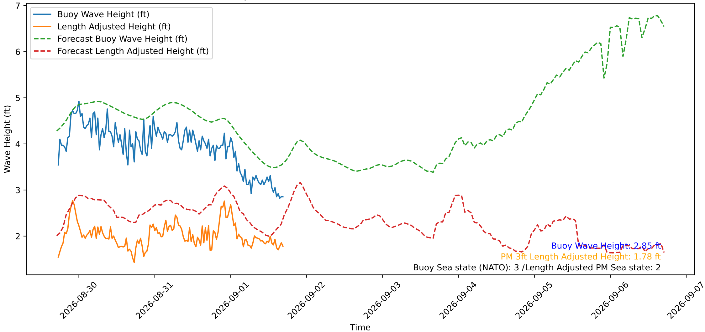
Wave Heights over Time for Green Beach at 2026-09-01 17:11:12
