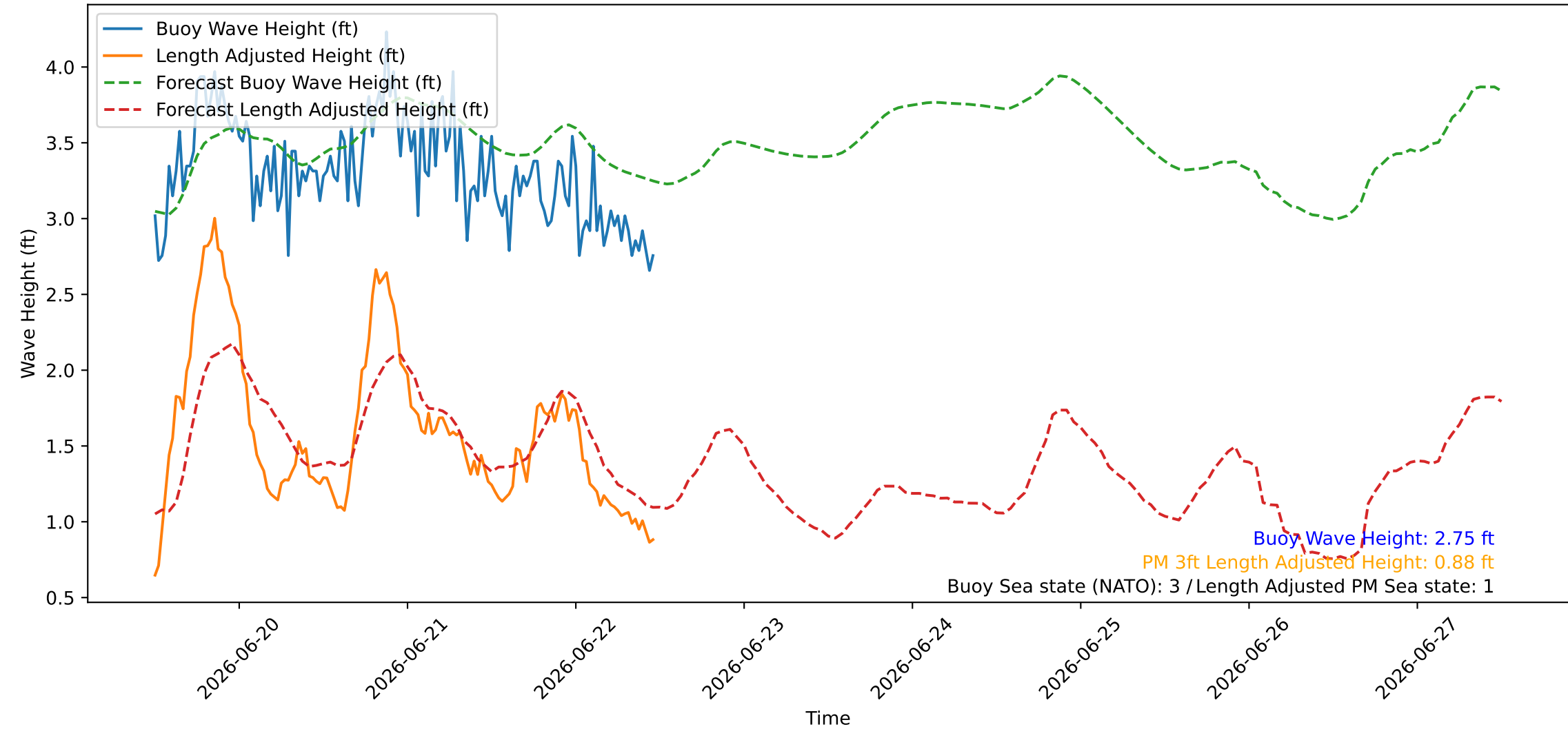
Wave Heights over Time for Green Beach at 2026-06-22 11:51:09
