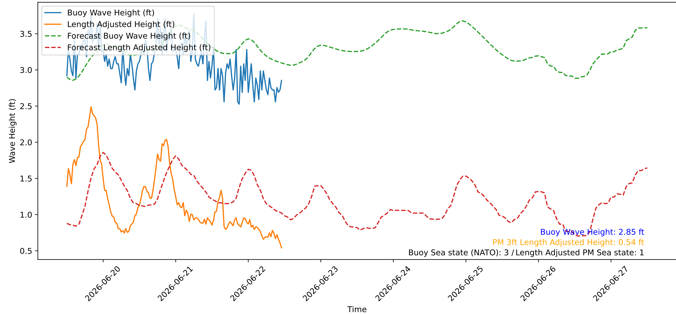
Wave Heights over Time for Red Beach at 2026-06-22 11:50:47
