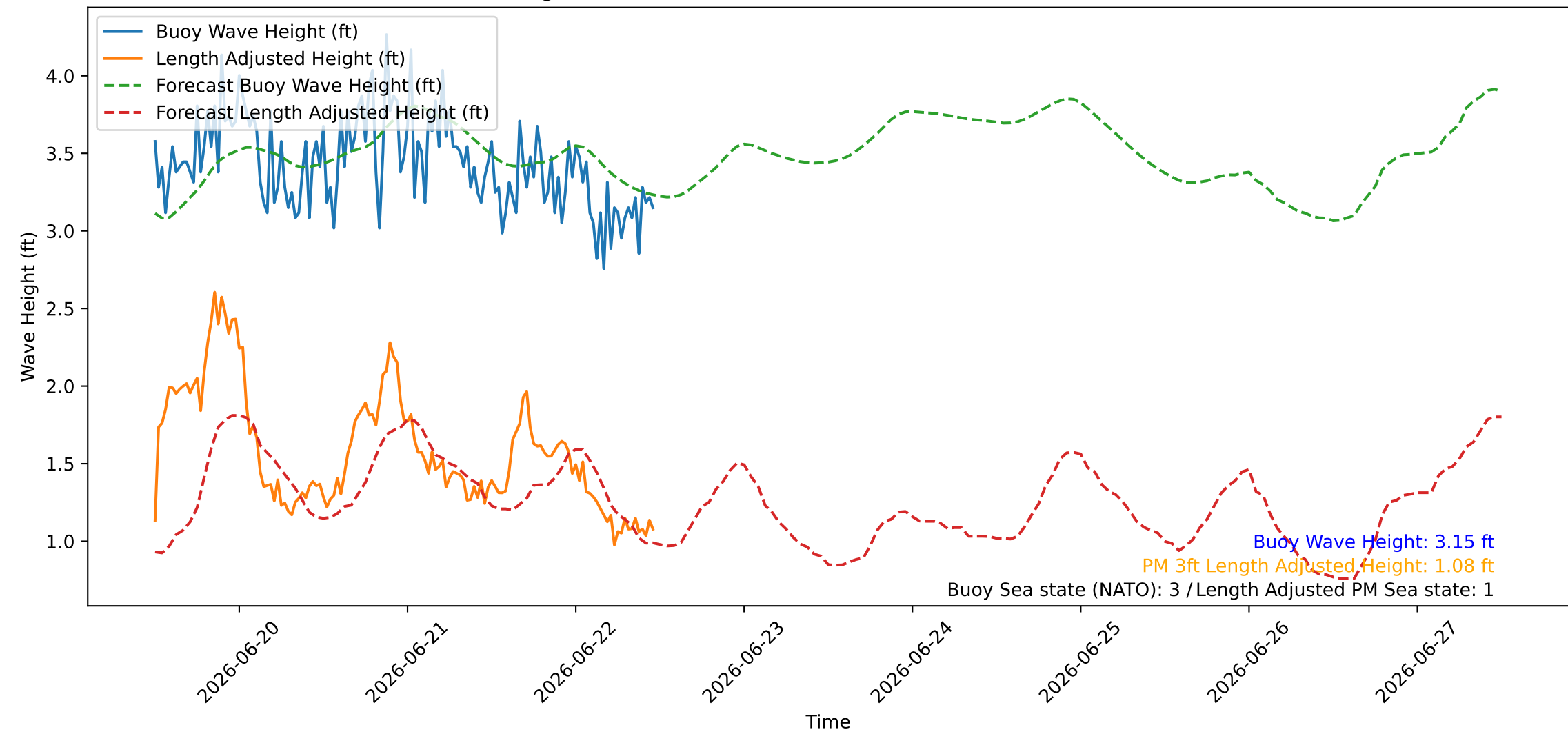
Wave Heights over Time for Oceanside Harbor at 2026-06-22 11:50:26
