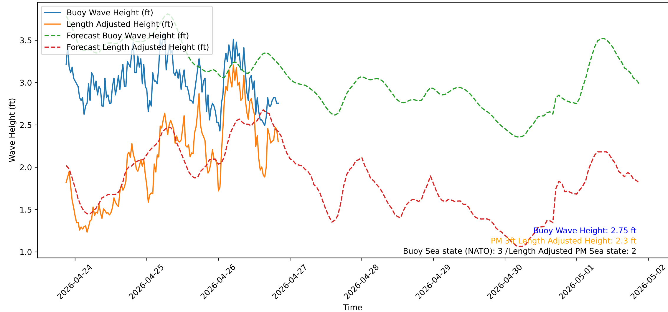
Wave Heights over Time for Green Beach at 2026-04-26 20:51:14
