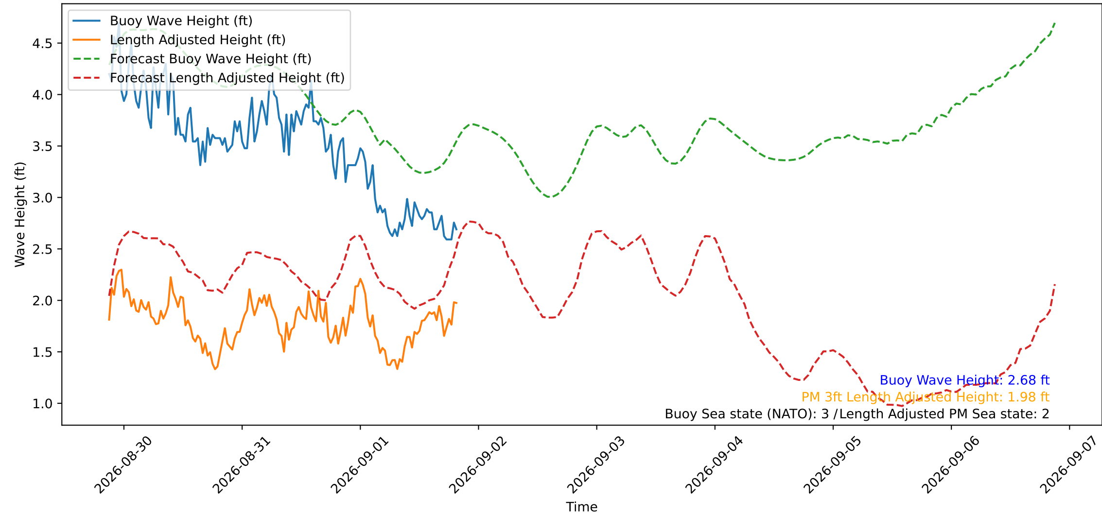
Wave Heights over Time for Red Beach at 2026-09-01 20:30:49
