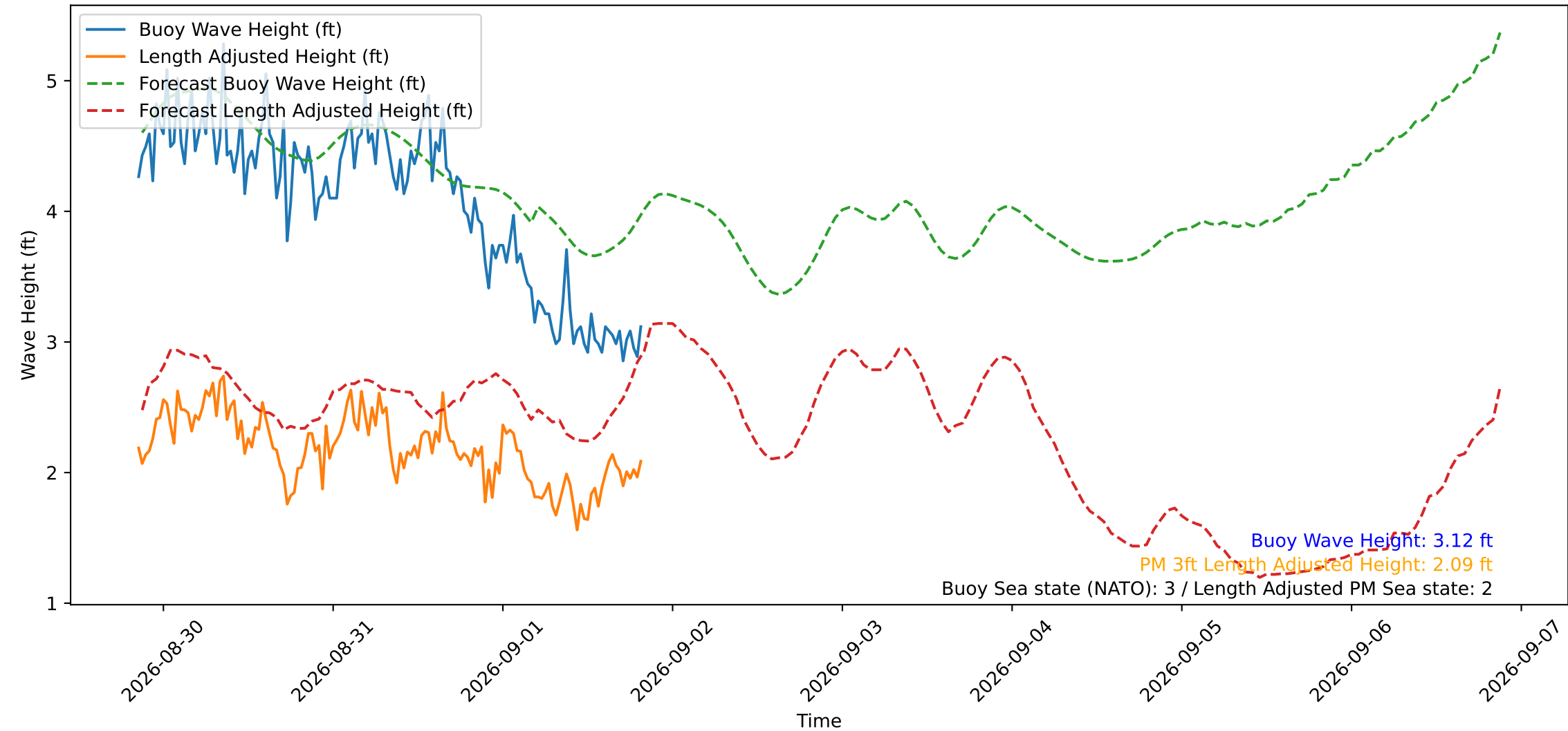
Wave Heights over Time for Oceanside Harbor at 2026-09-01 20:30:30
