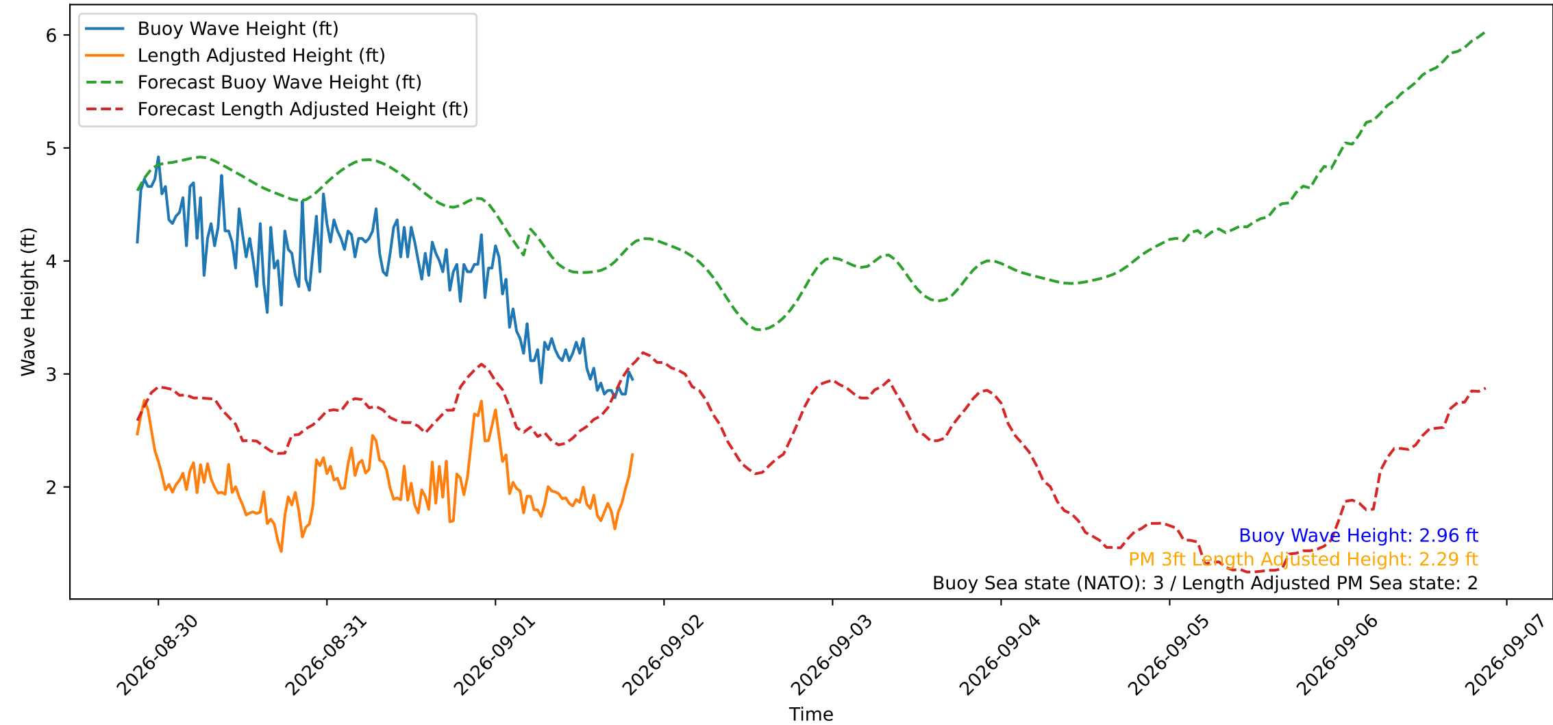
Wave Heights over Time for Green Beach at 2026-09-01 20:31:12
