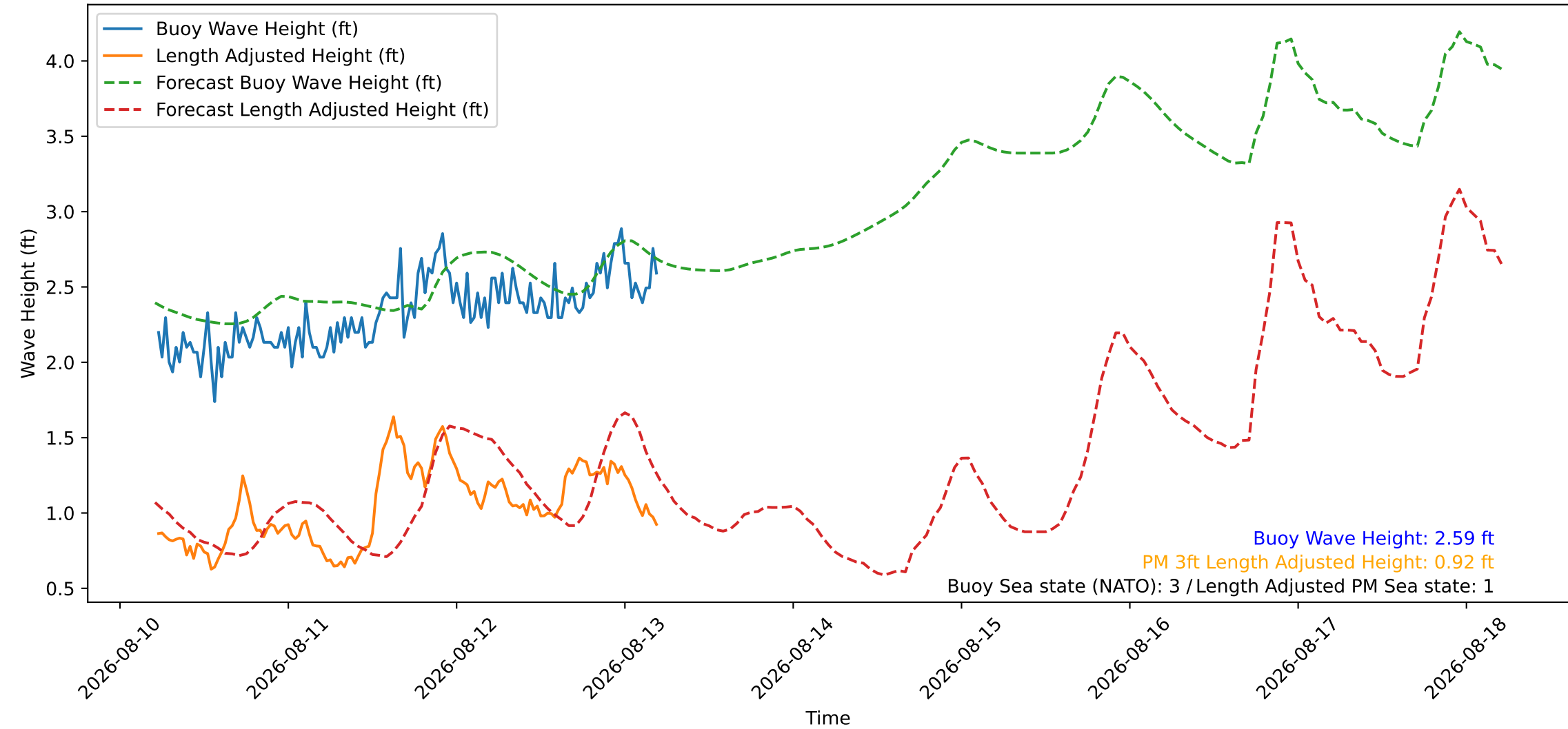
Wave Heights over Time for Red Beach at 2026-08-13 05:20:47
