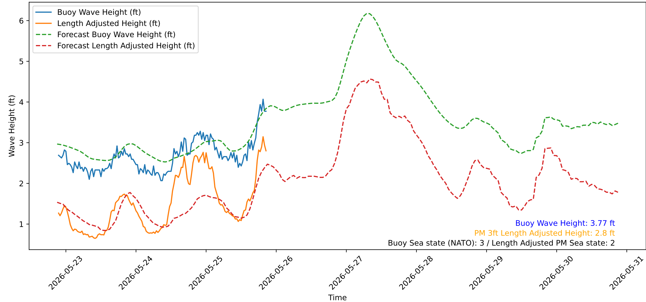
Wave Heights over Time for Green Beach at 2026-05-25 21:21:13
