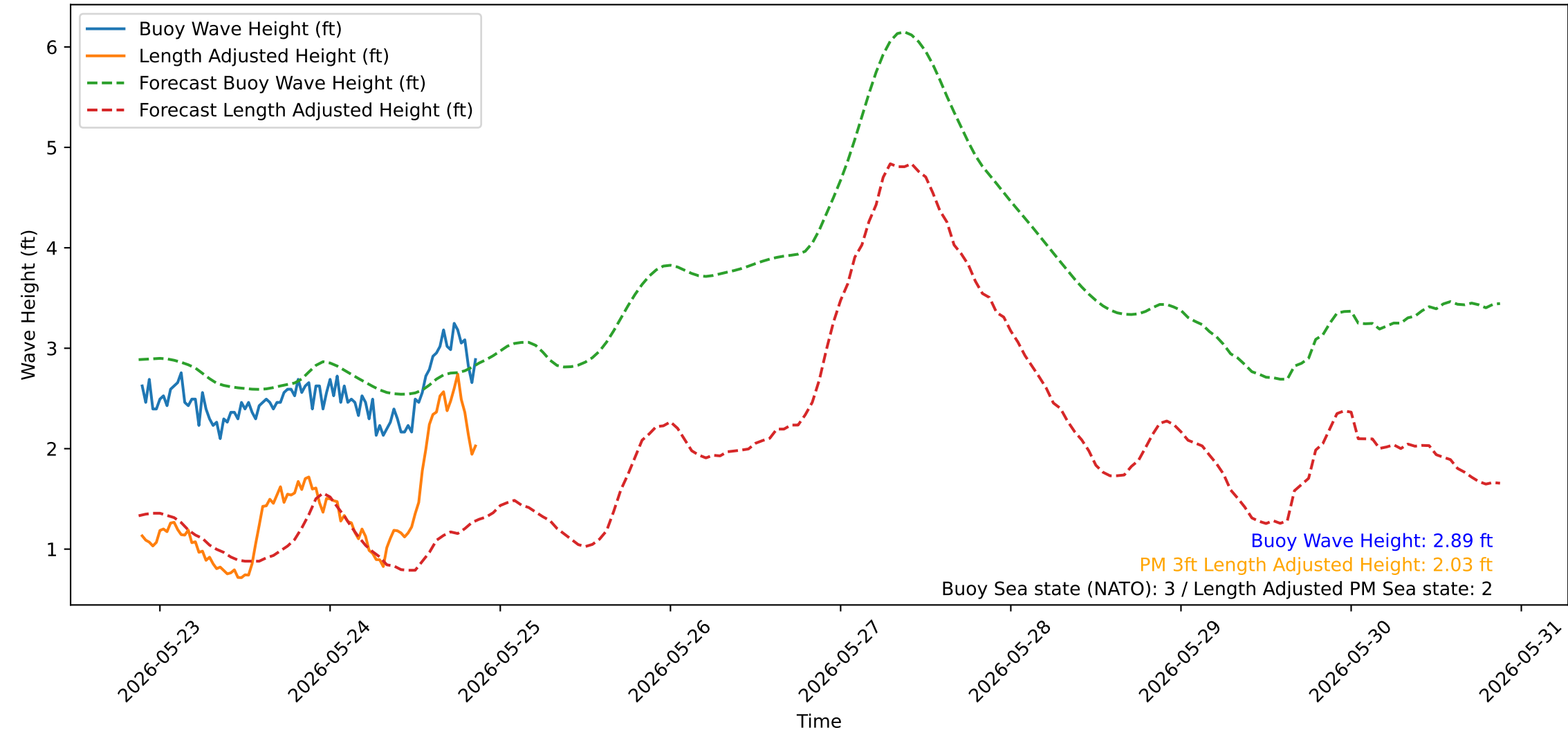
Wave Heights over Time for Oceanside Harbor at 2026-05-25 21:20:29
