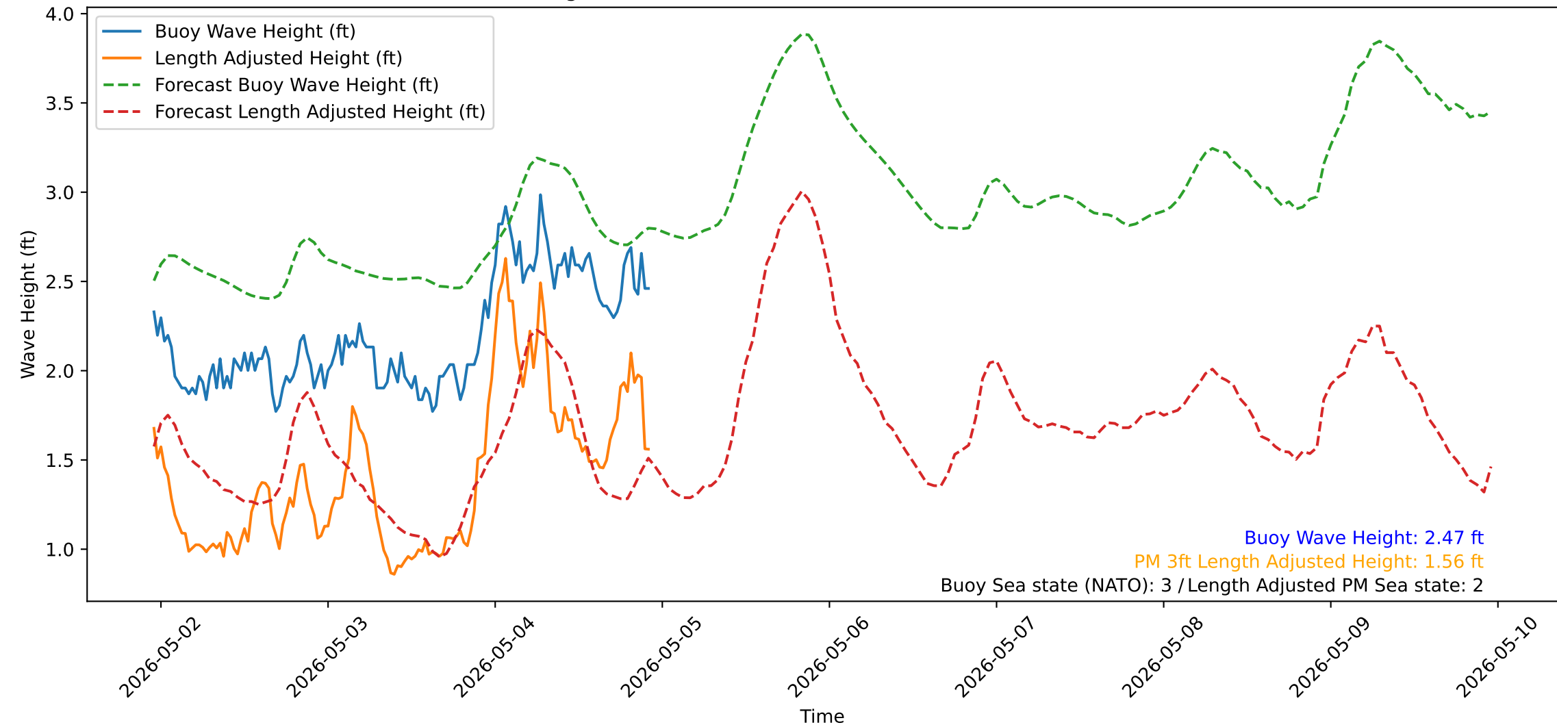
Wave Heights over Time for Green Beach at 2026-05-04 23:01:13
