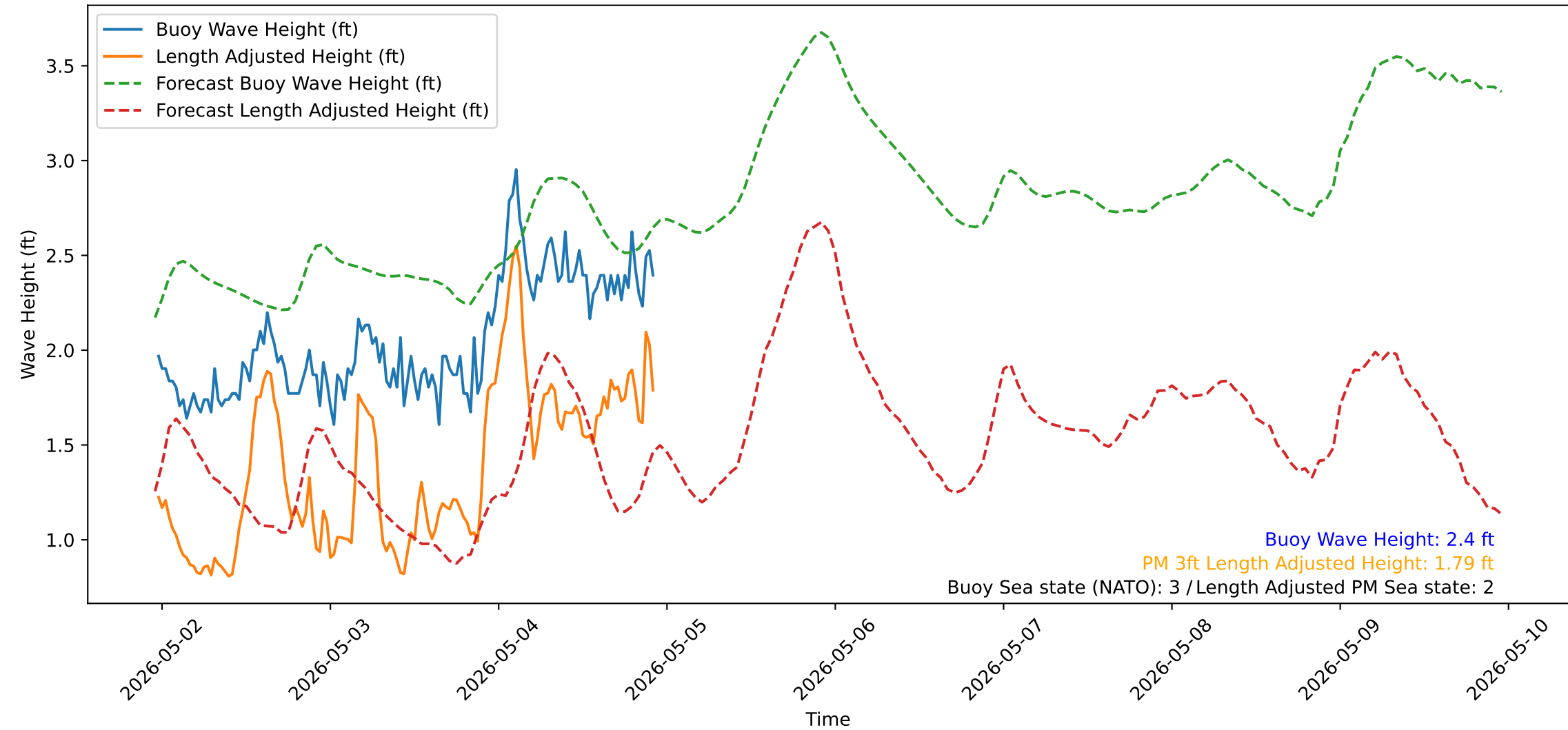
Wave Heights over Time for Red Beach at 2026-05-04 23:00:50
