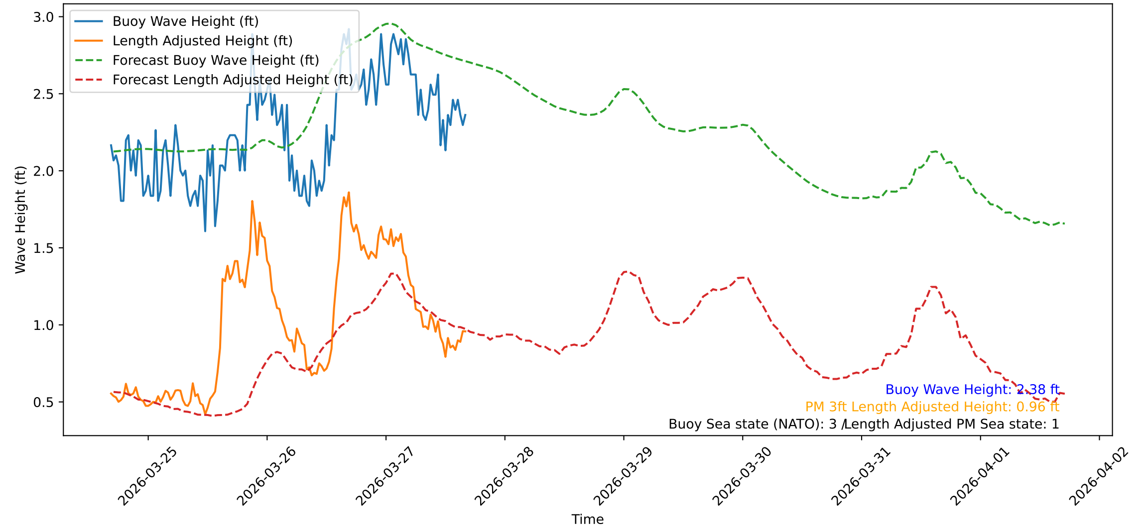
Wave Heights over Time for Oceanside Harbor at 2026-03-27 16:40:31
