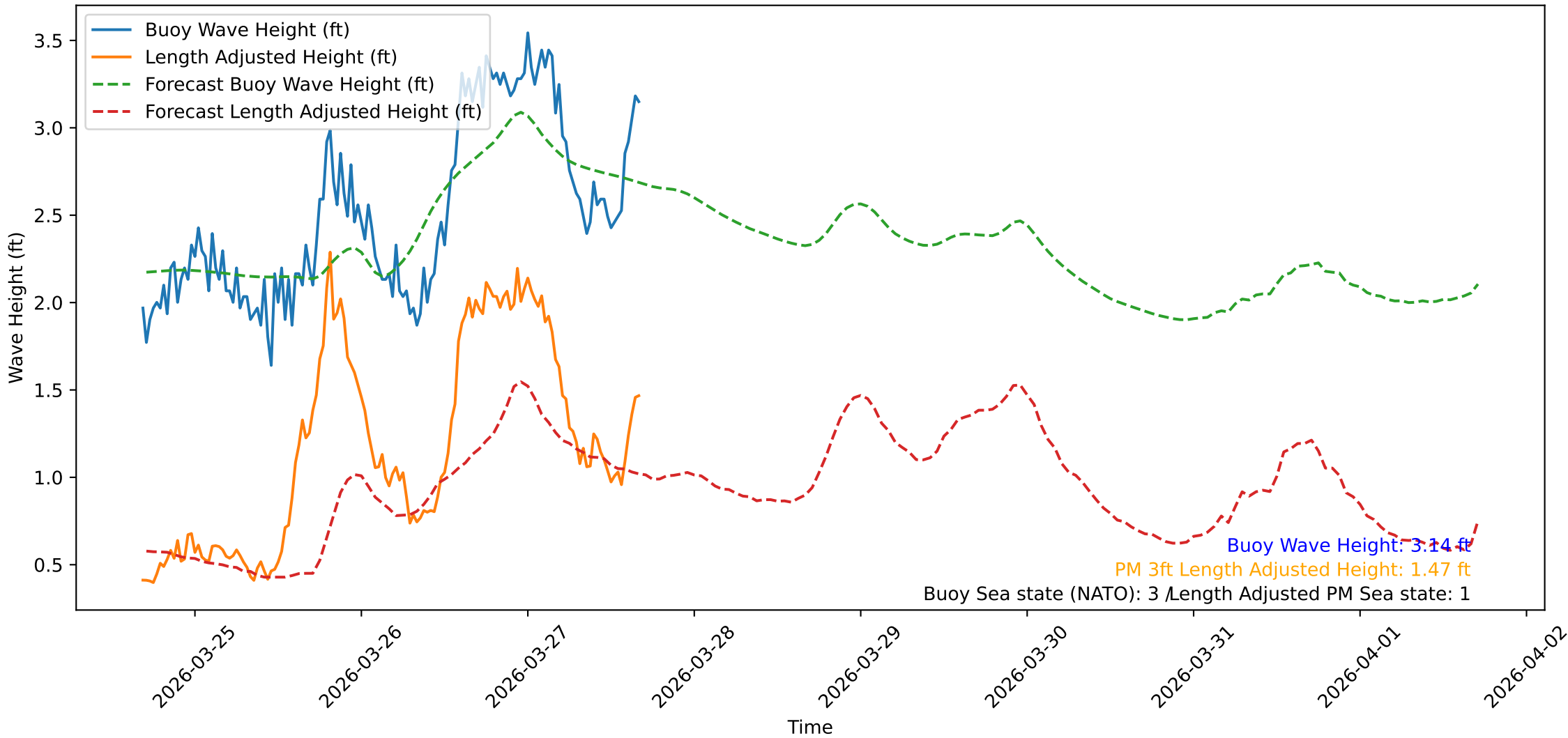
Wave Heights over Time for Green Beach at 2026-03-27 16:41:10
