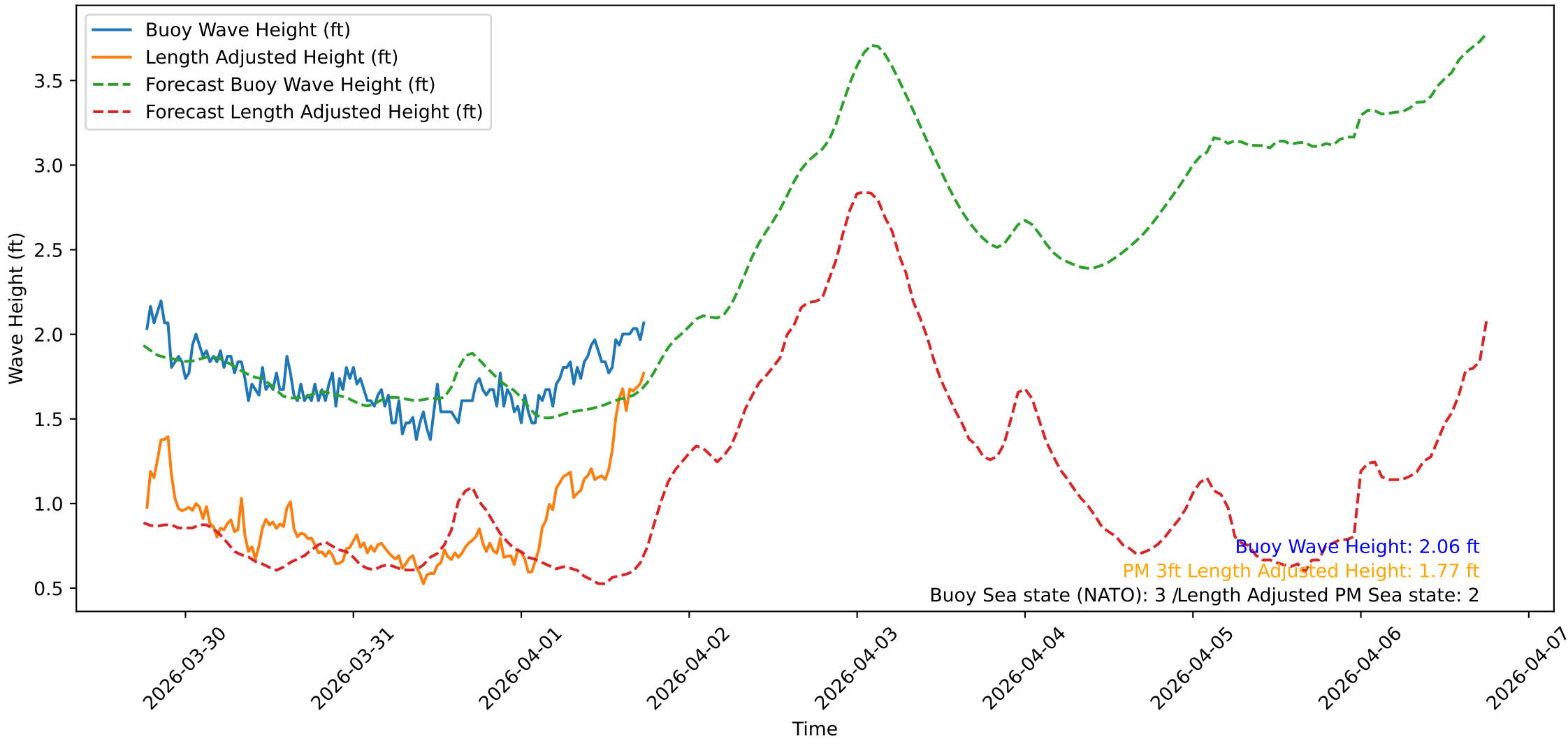
Wave Heights over Time for Red Beach at 2026-04-01 18:20:47
