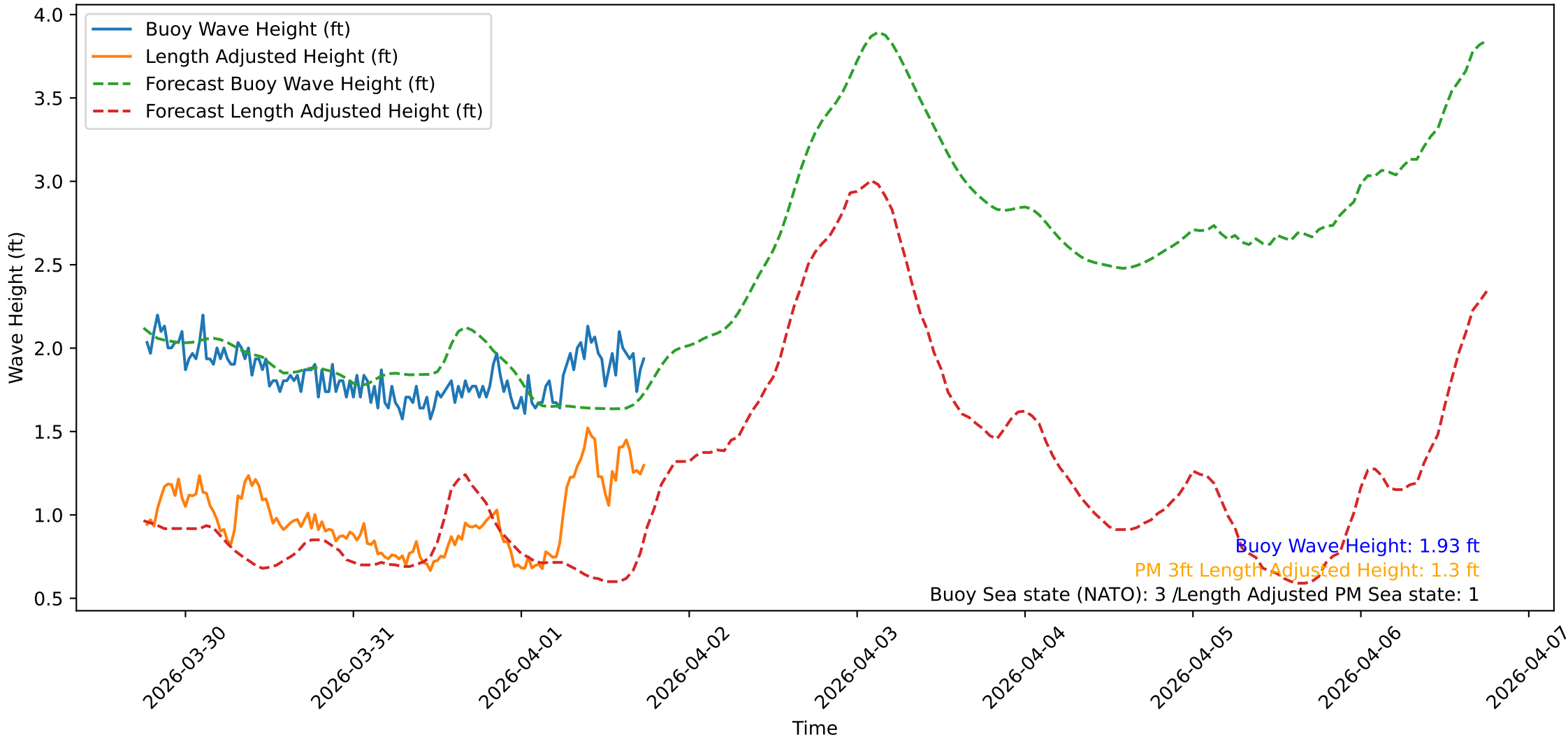
Wave Heights over Time for Oceanside Harbor at 2026-04-01 18:20:31
