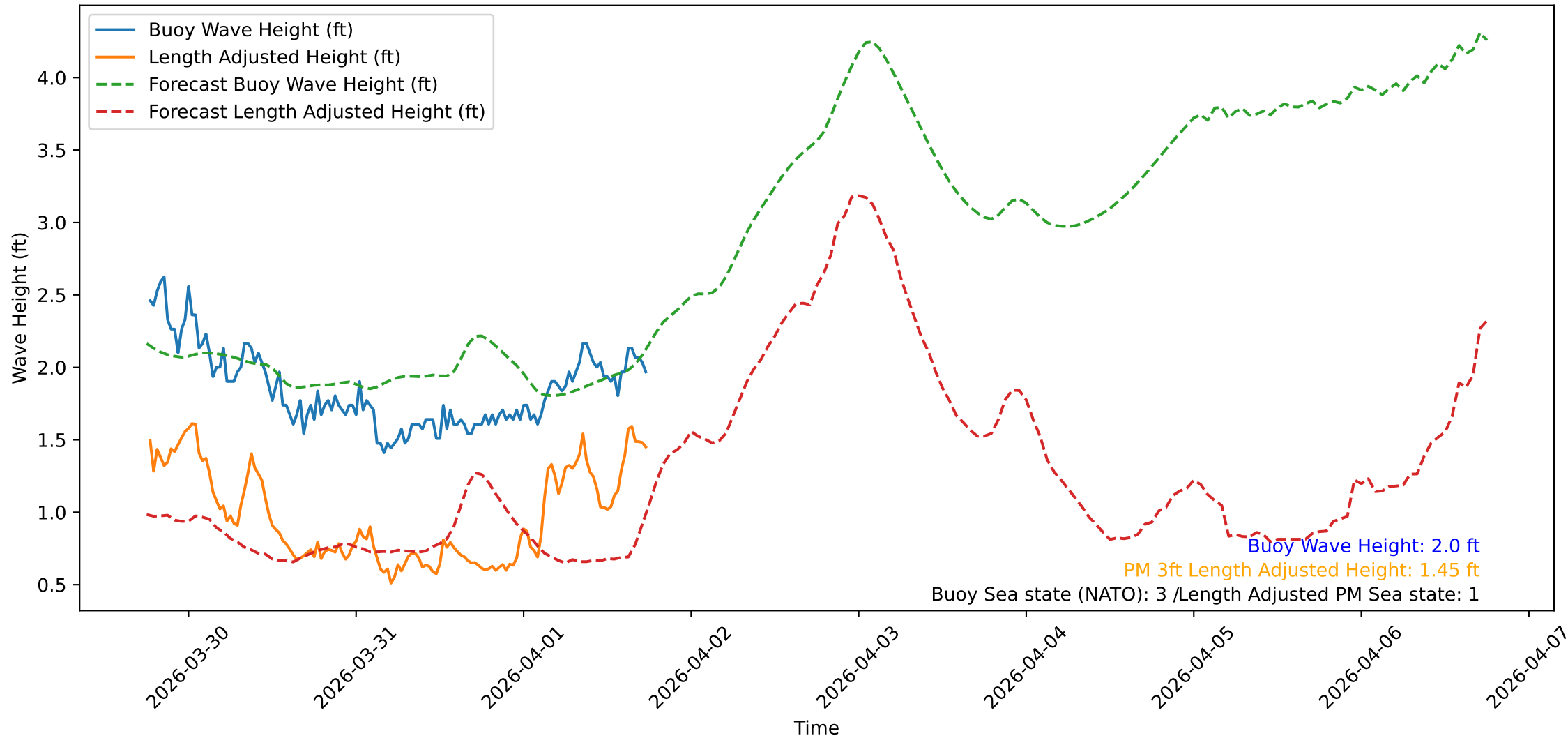
Wave Heights over Time for Green Beach at 2026-04-01 18:21:09
