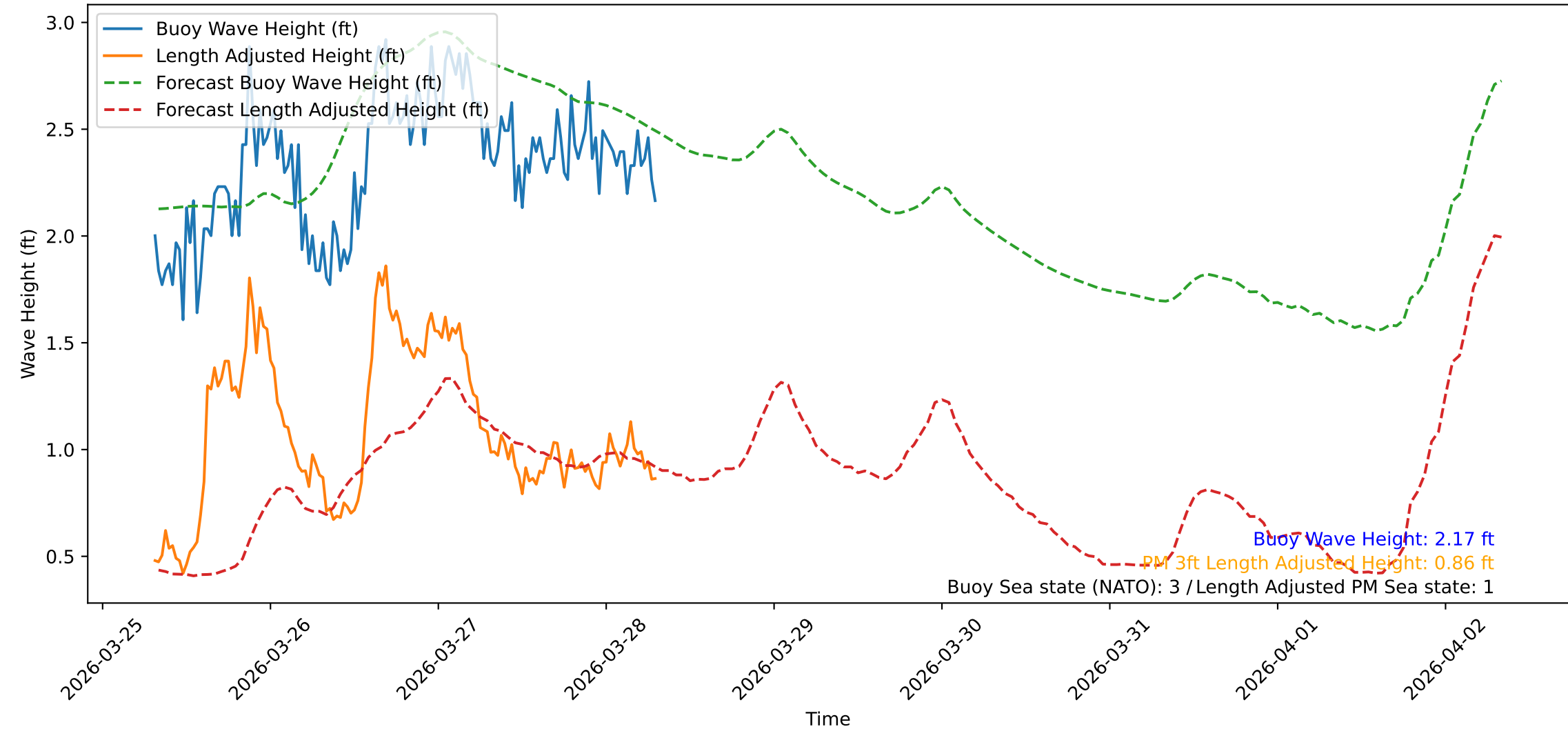
Wave Heights over Time for Oceanside Harbor at 2026-03-28 07:40:31
