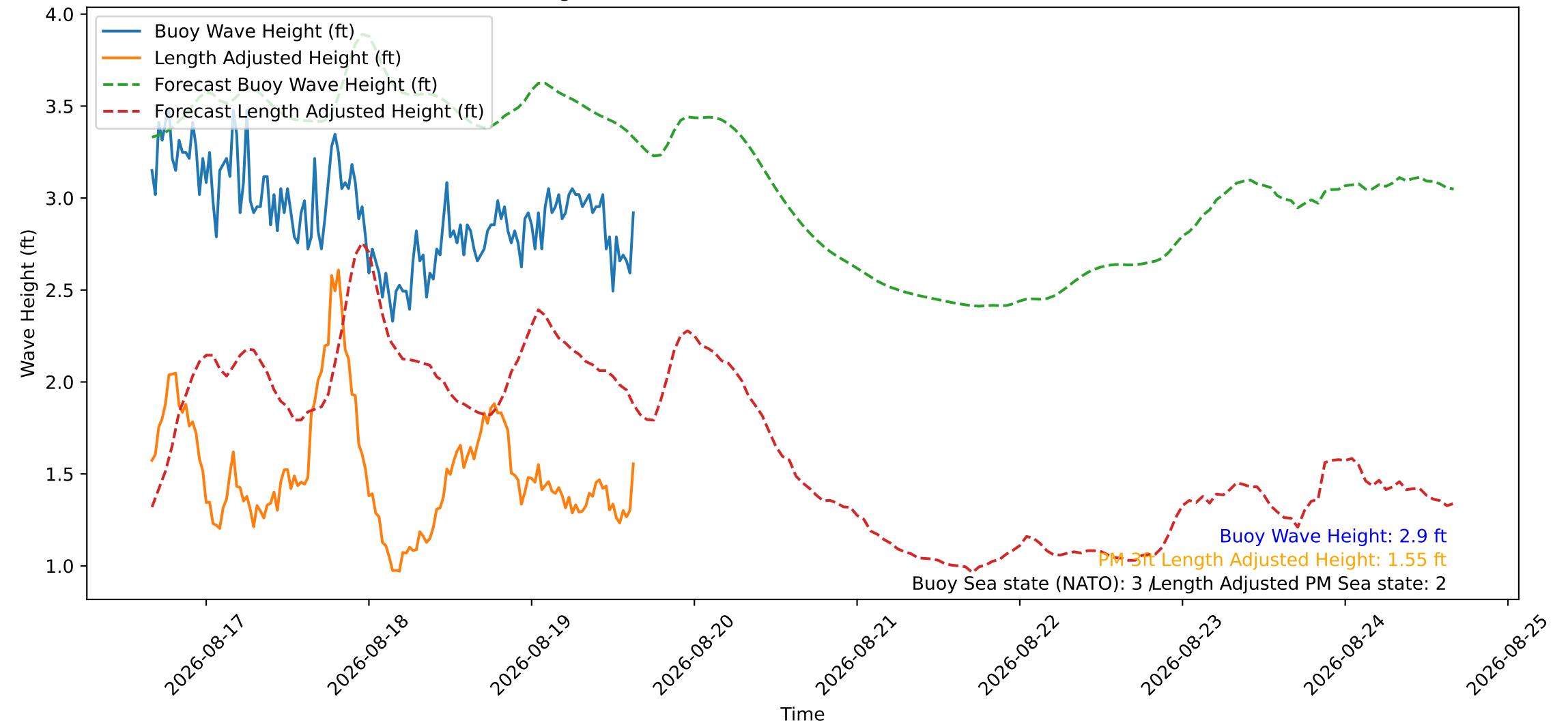
Wave Heights over Time for Red Beach at 2026-08-19 15:50:47
