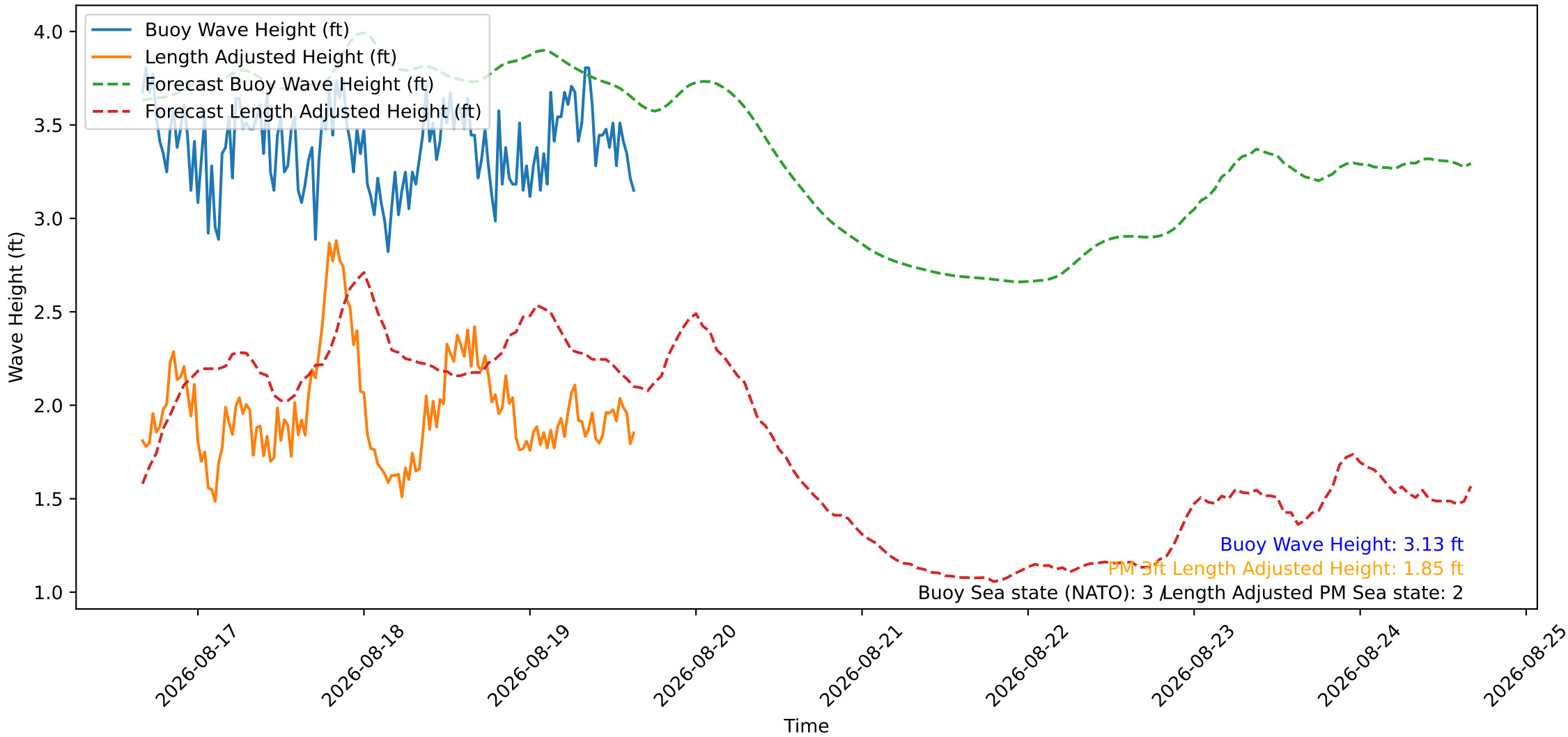
Wave Heights over Time for Oceanside Harbor at 2026-08-19 15:50:26
