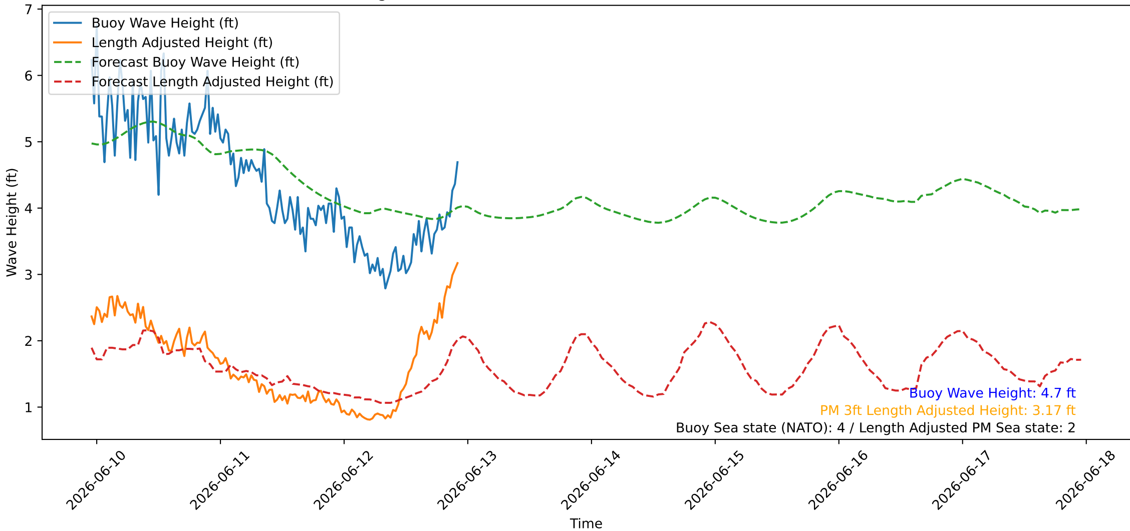
Wave Heights over Time for Oceanside Harbor at 2026-06-12 23:00:26
