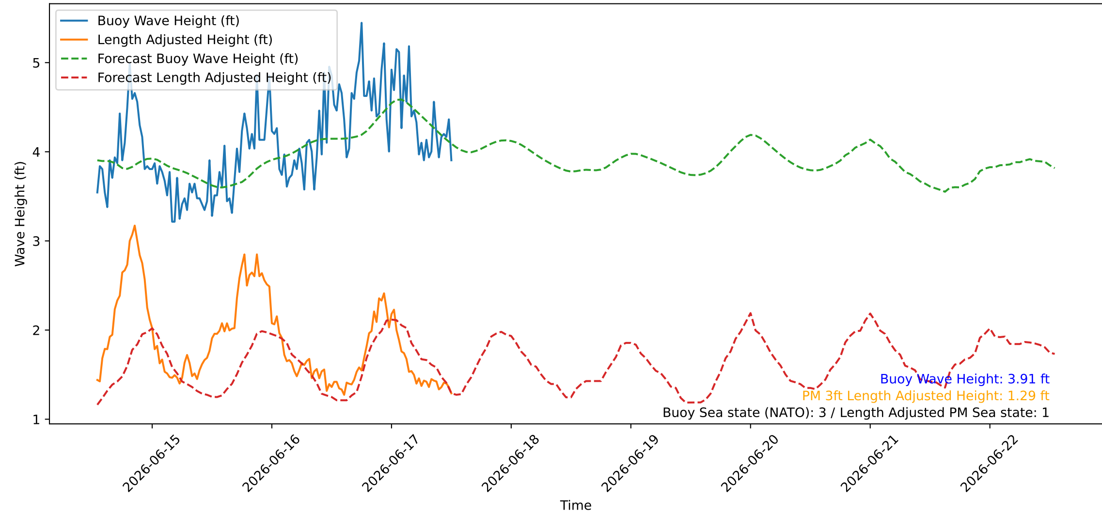
Wave Heights over Time for Oceanside Harbor at 2026-06-17 13:00:26
