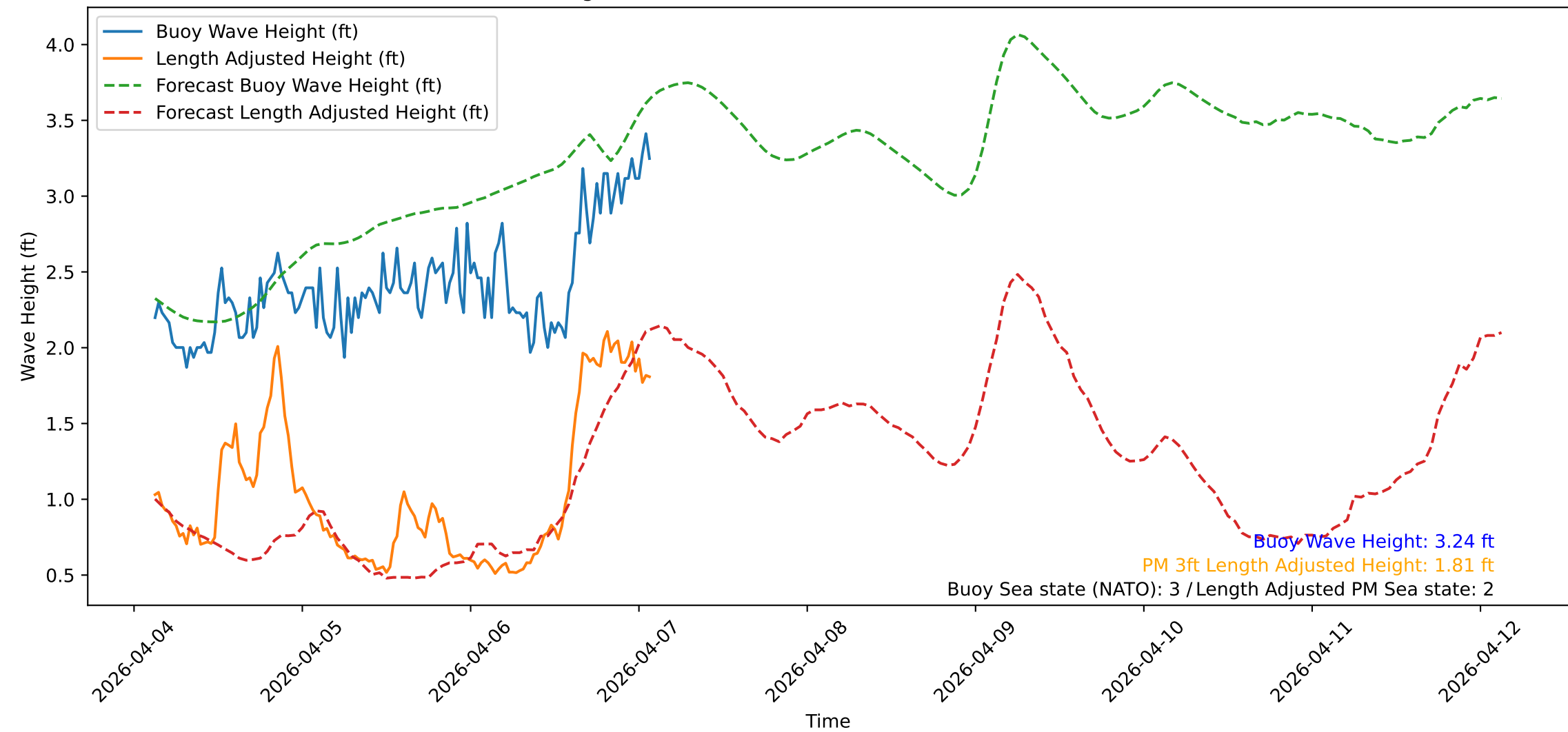
Wave Heights over Time for Red Beach at 2026-04-07 02:50:48
