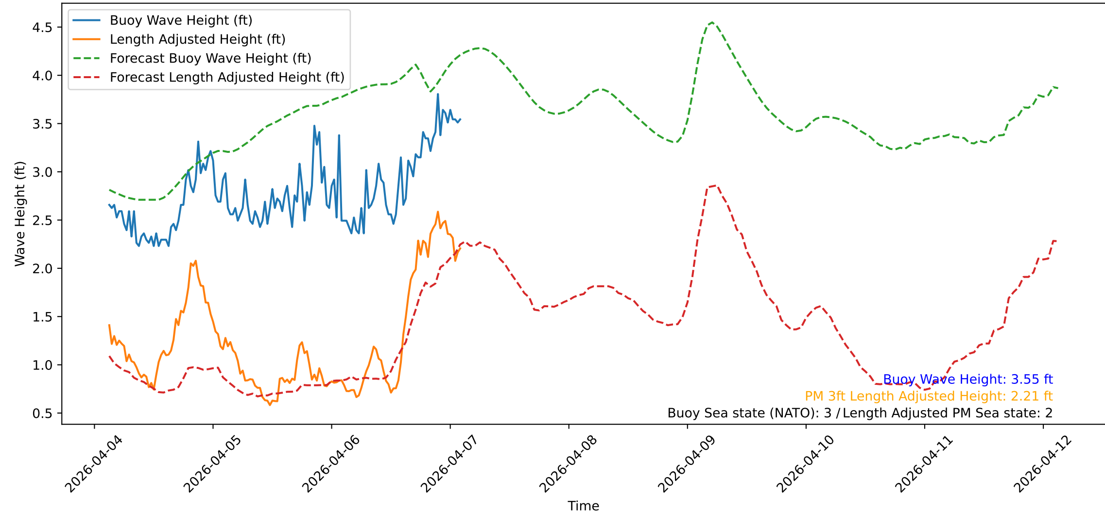
Wave Heights over Time for Green Beach at 2026-04-07 02:51:11
