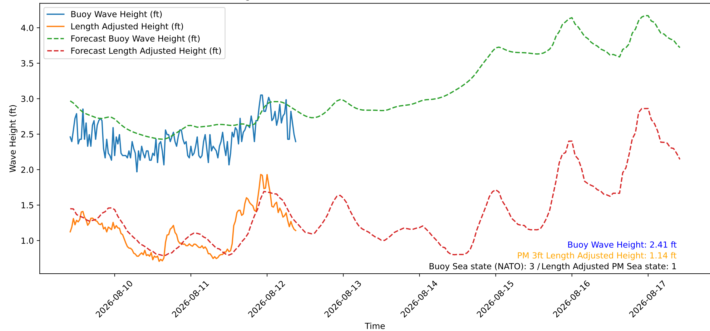
Wave Heights over Time for Oceanside Harbor at 2026-08-12 09:50:26
