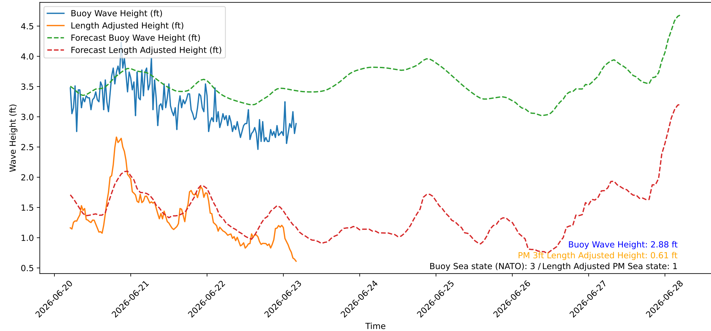
Wave Heights over Time for Green Beach at 2026-06-23 05:01:07
