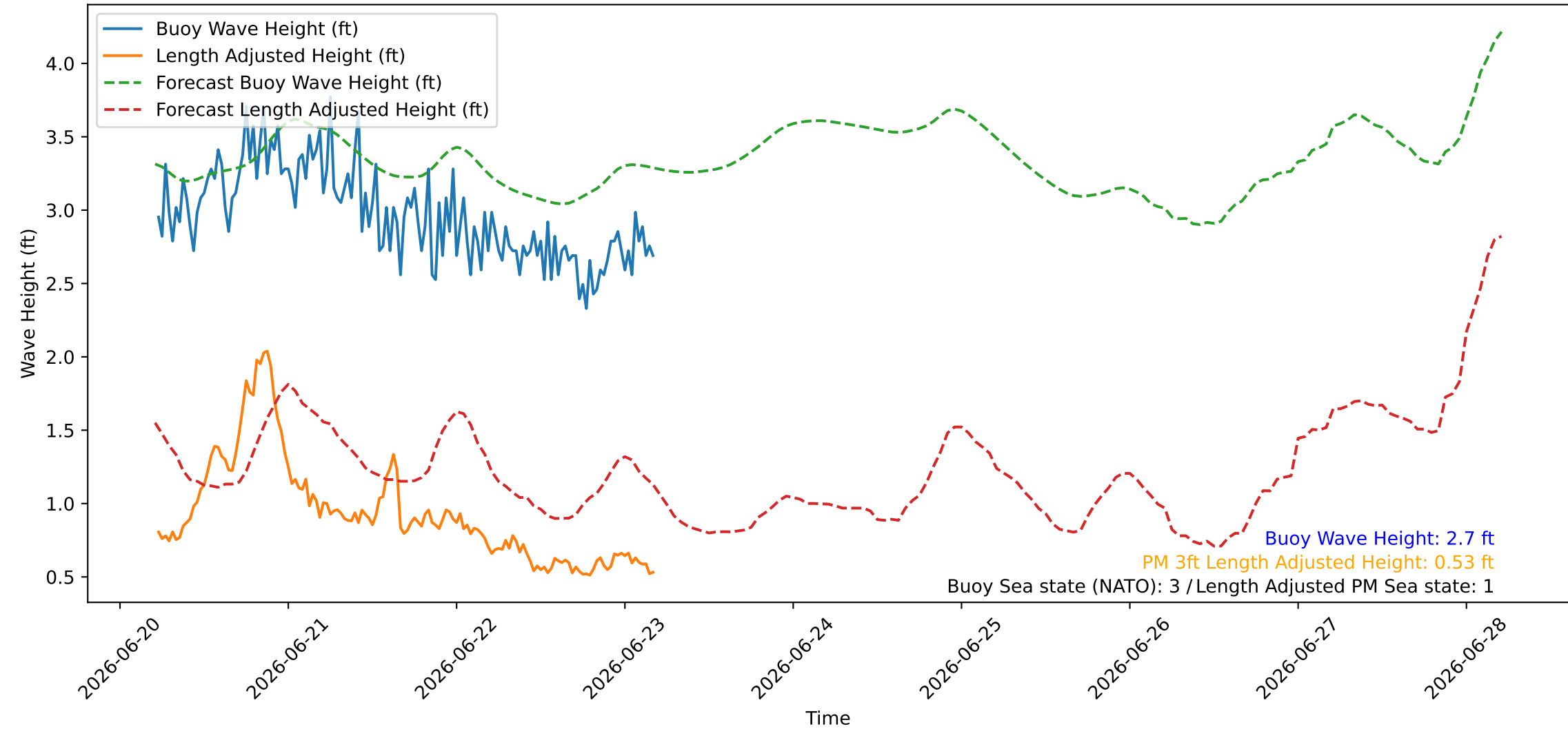
Wave Heights over Time for Red Beach at 2026-06-23 05:00:44
