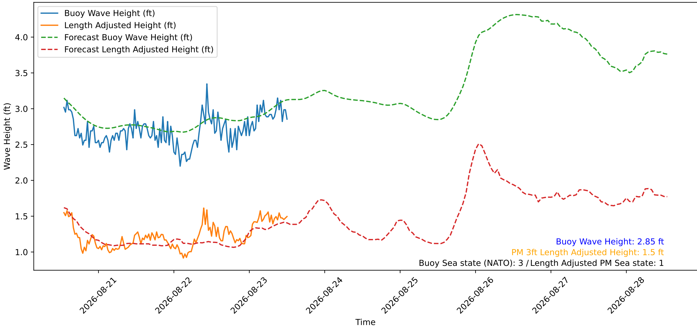
Wave Heights over Time for Oceanside Harbor at 2026-08-23 13:10:30
