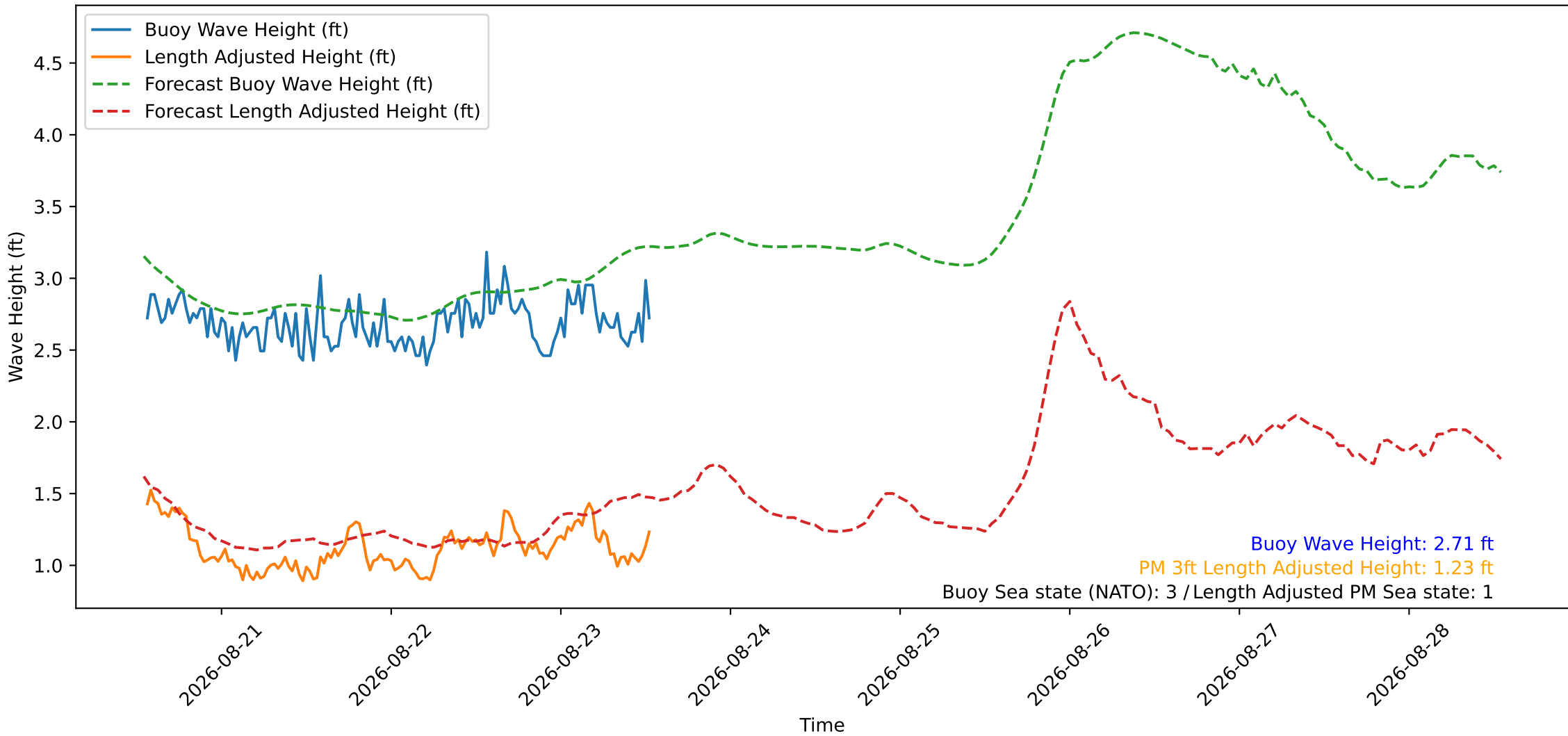
Wave Heights over Time for Green Beach at 2026-08-23 13:11:12
