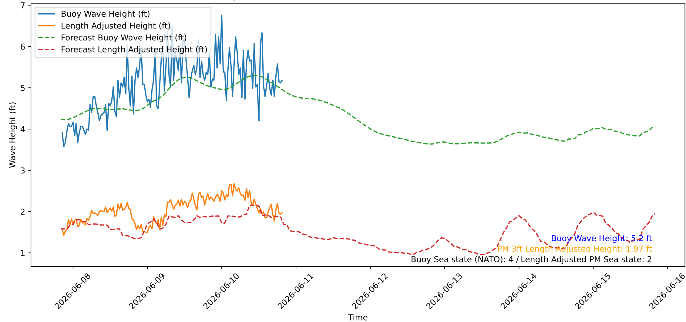
Wave Heights over Time for Oceanside Harbor at 2026-06-10 20:20:26
