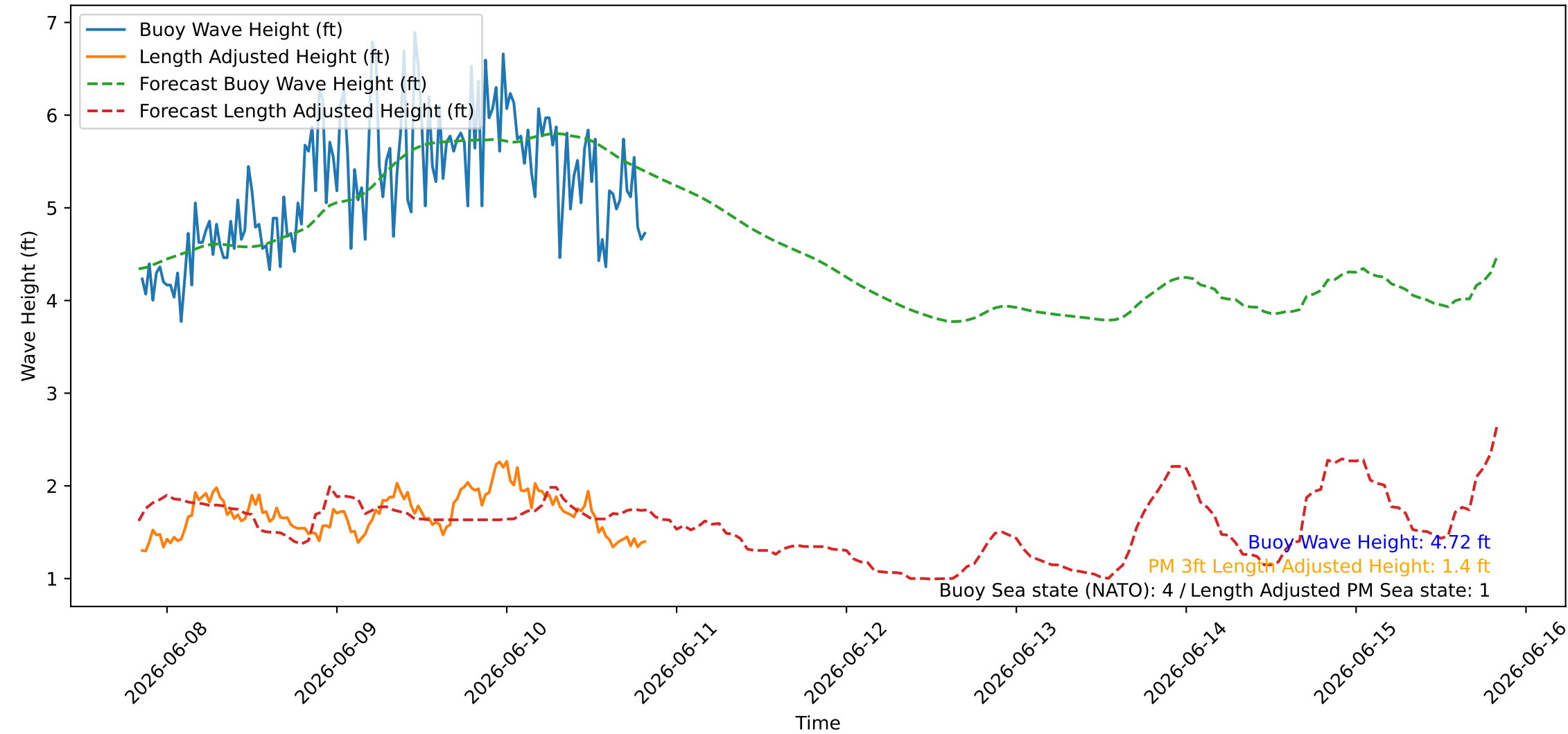
Wave Heights over Time for Green Beach at 2026-06-10 20:21:11
