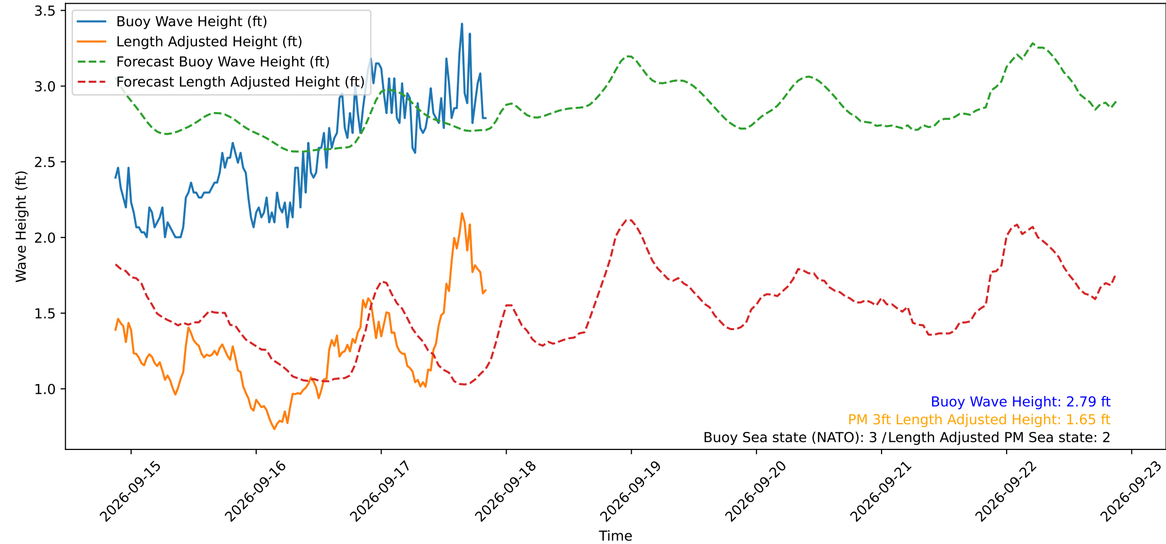
Wave Heights over Time for Red Beach at 2026-09-17 20:40:49
