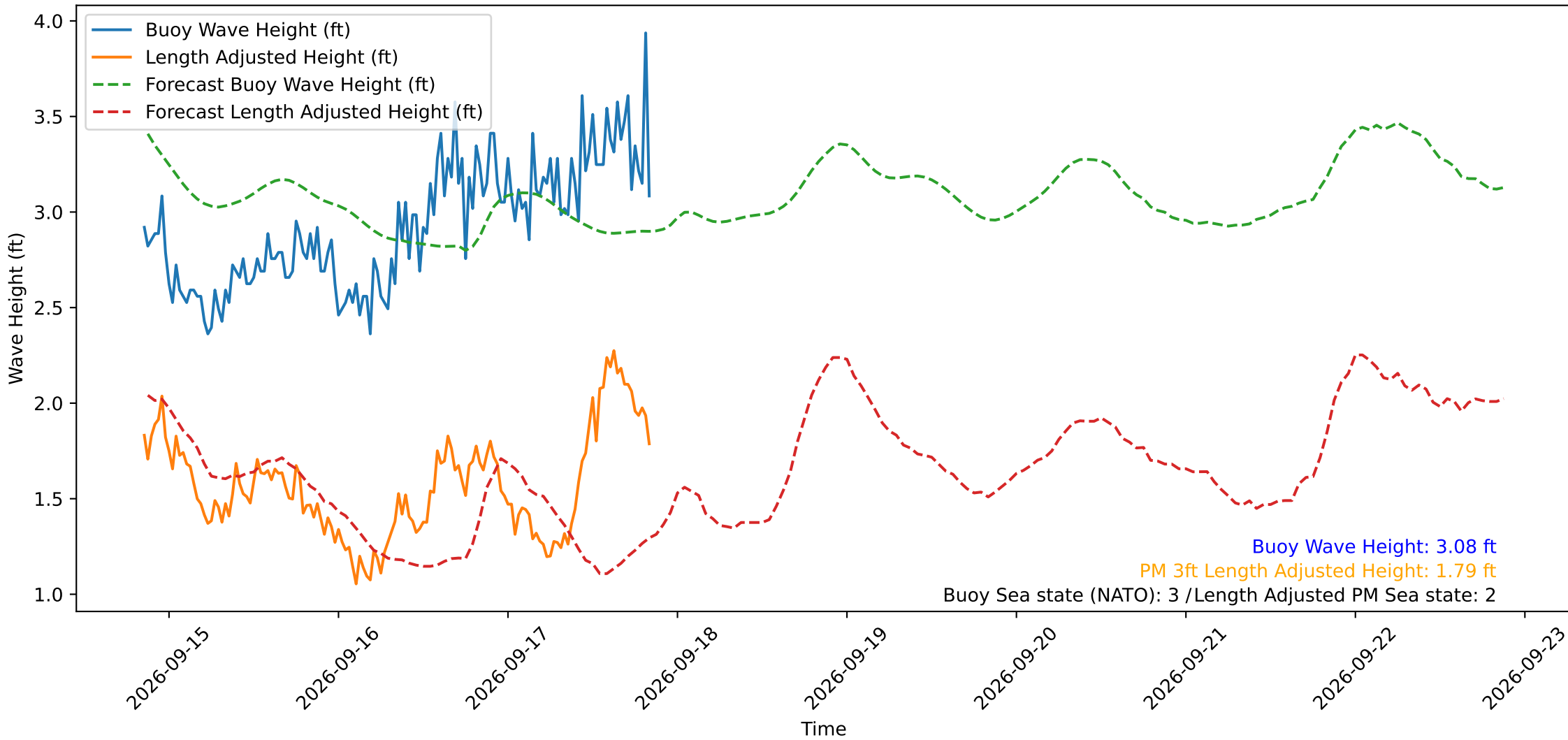
Wave Heights over Time for Oceanside Harbor at 2026-09-17 20:40:29
