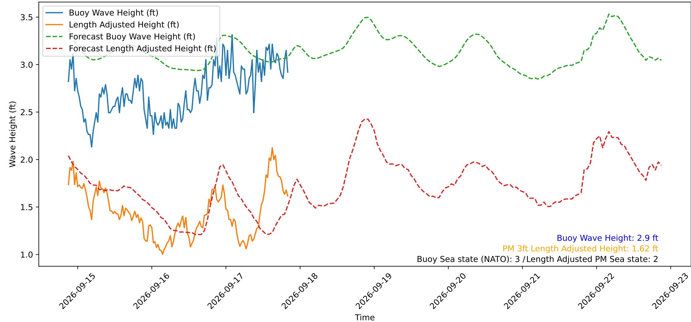
Wave Heights over Time for Green Beach at 2026-09-17 20:41:11
