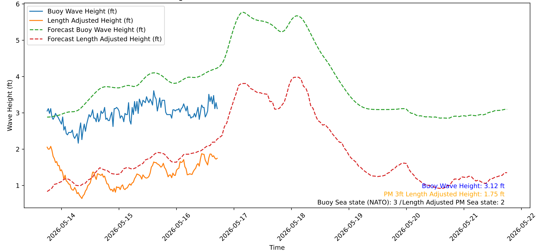
Wave Heights over Time for Oceanside Harbor at 2026-05-16 17:50:31
