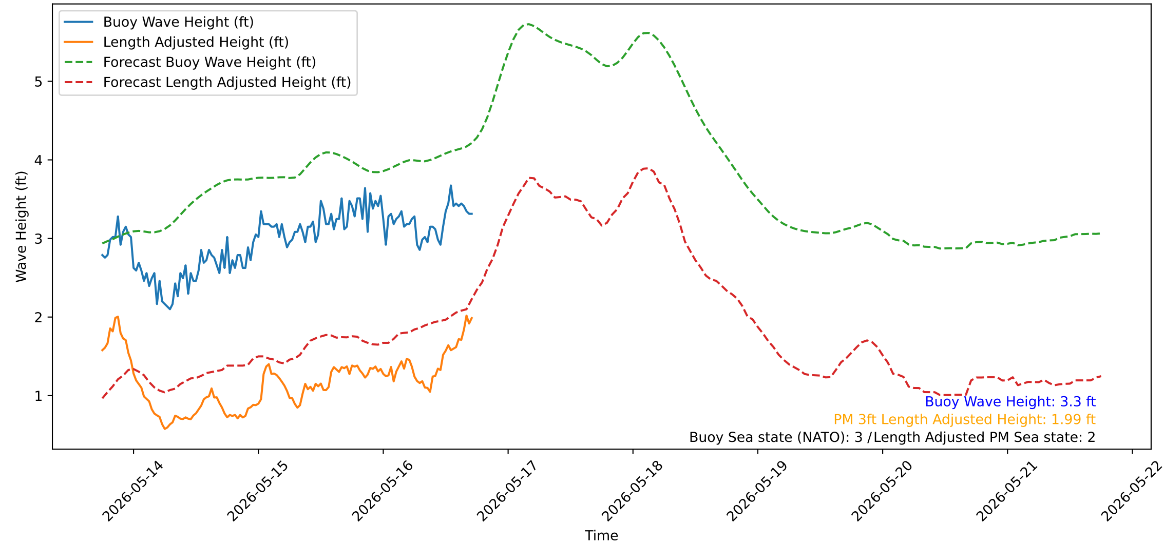
Wave Heights over Time for Green Beach at 2026-05-16 17:51:14
