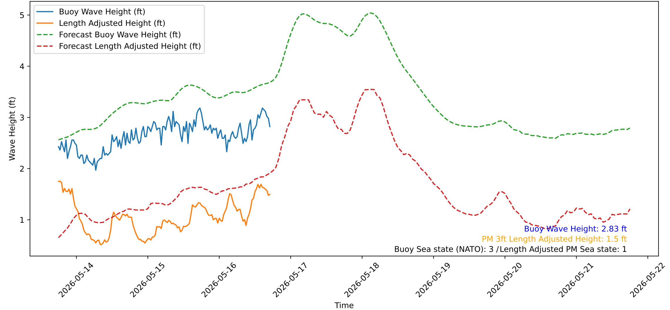
Wave Heights over Time for Red Beach at 2026-05-16 17:50:51
