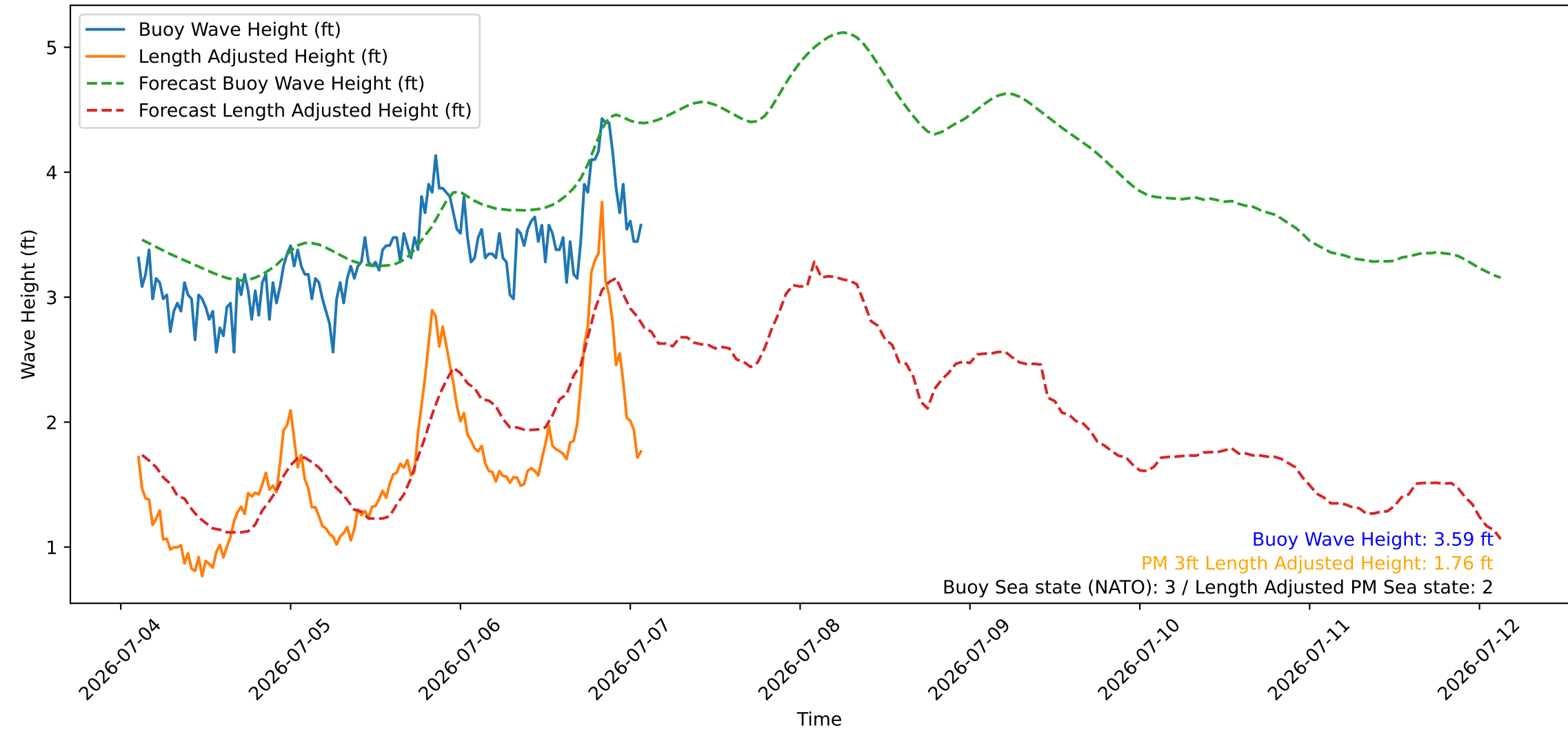
Wave Heights over Time for Green Beach at 2026-07-07 02:31:08
