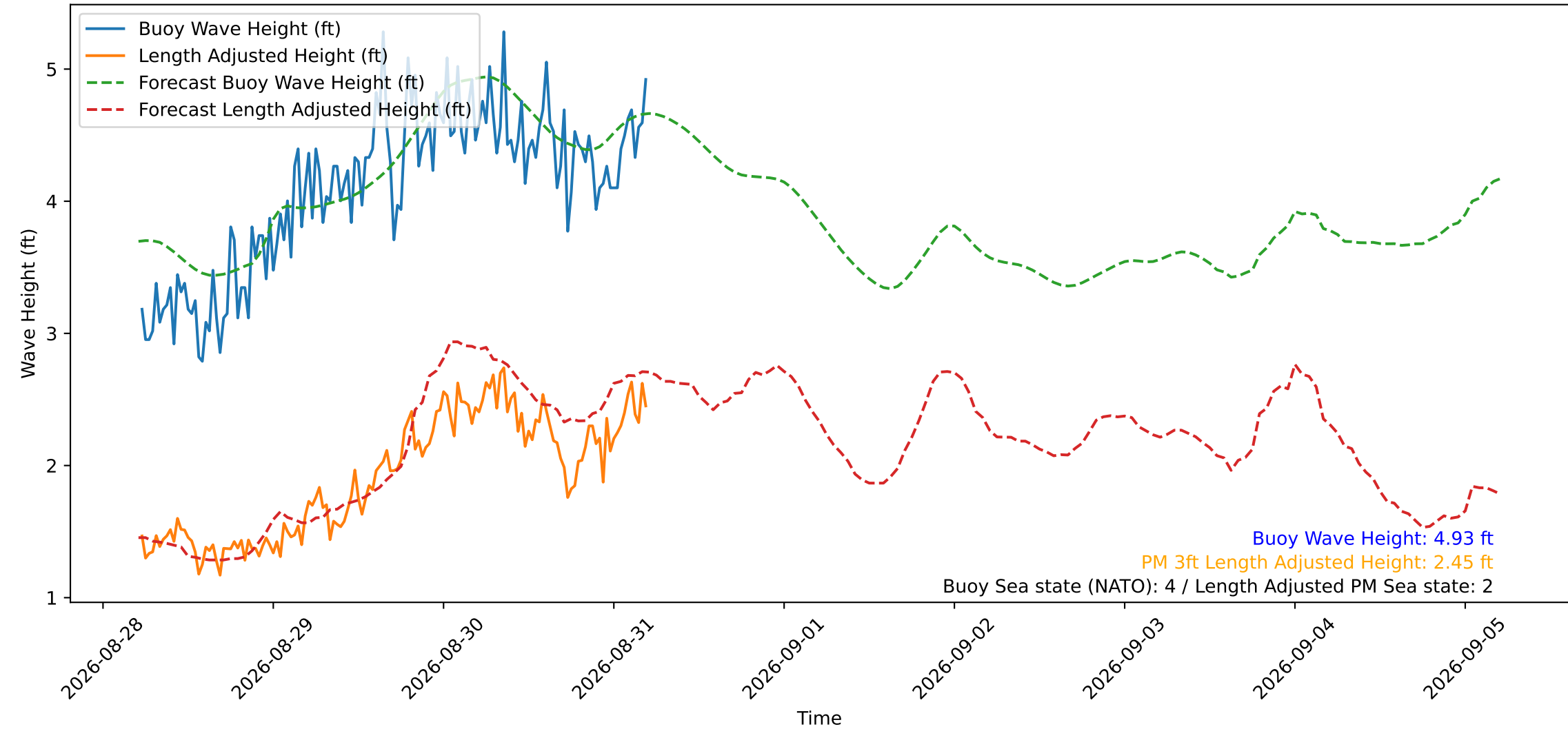
Wave Heights over Time for Oceanside Harbor at 2026-08-31 05:20:30
