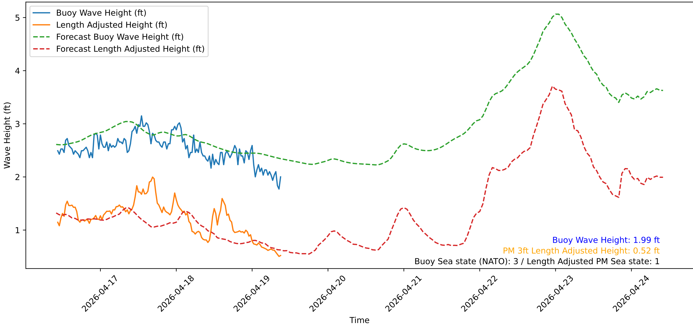
Wave Heights over Time for Red Beach at 2026-04-19 10:10:50
