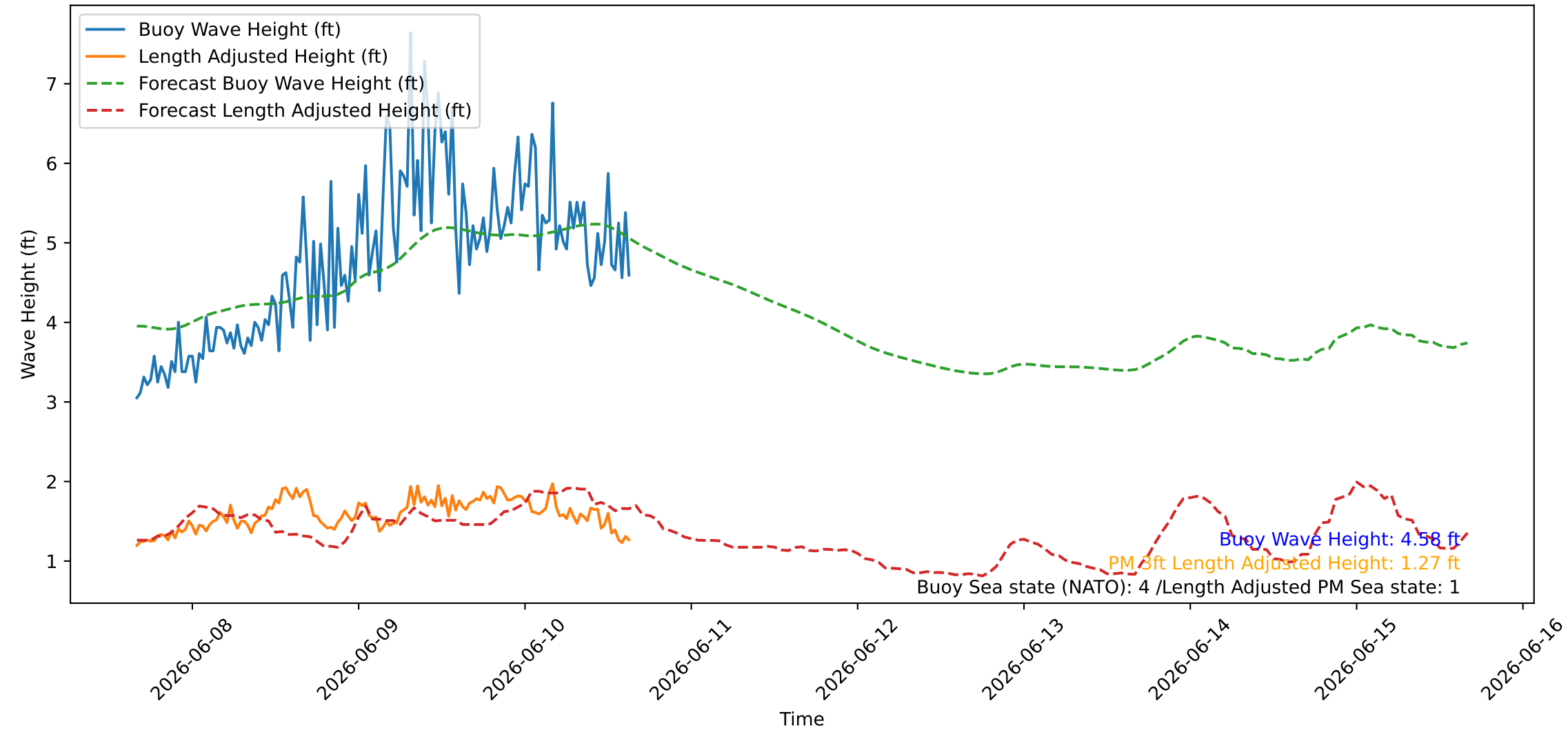
Wave Heights over Time for Red Beach at 2026-06-10 15:50:48
