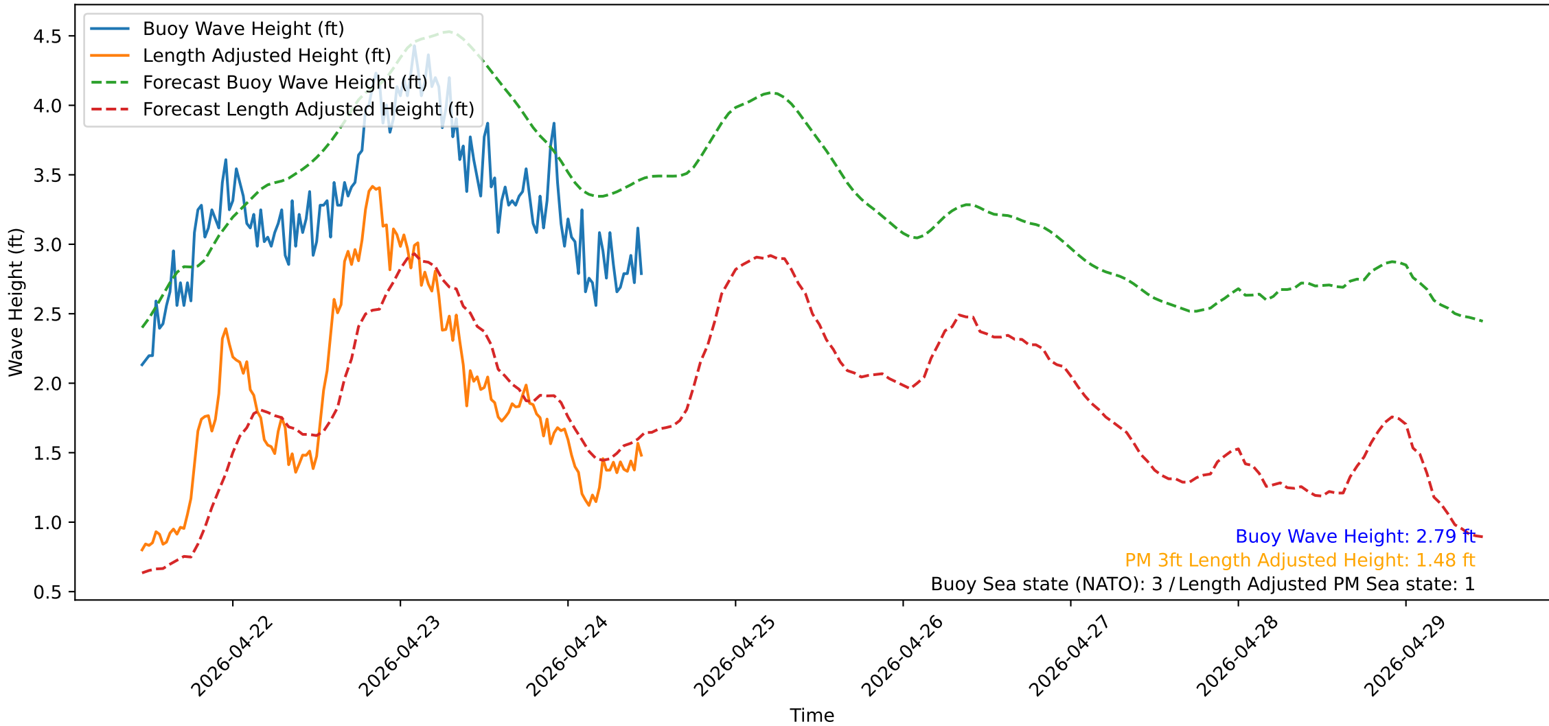
Wave Heights over Time for Oceanside Harbor at 2026-04-24 11:10:31
