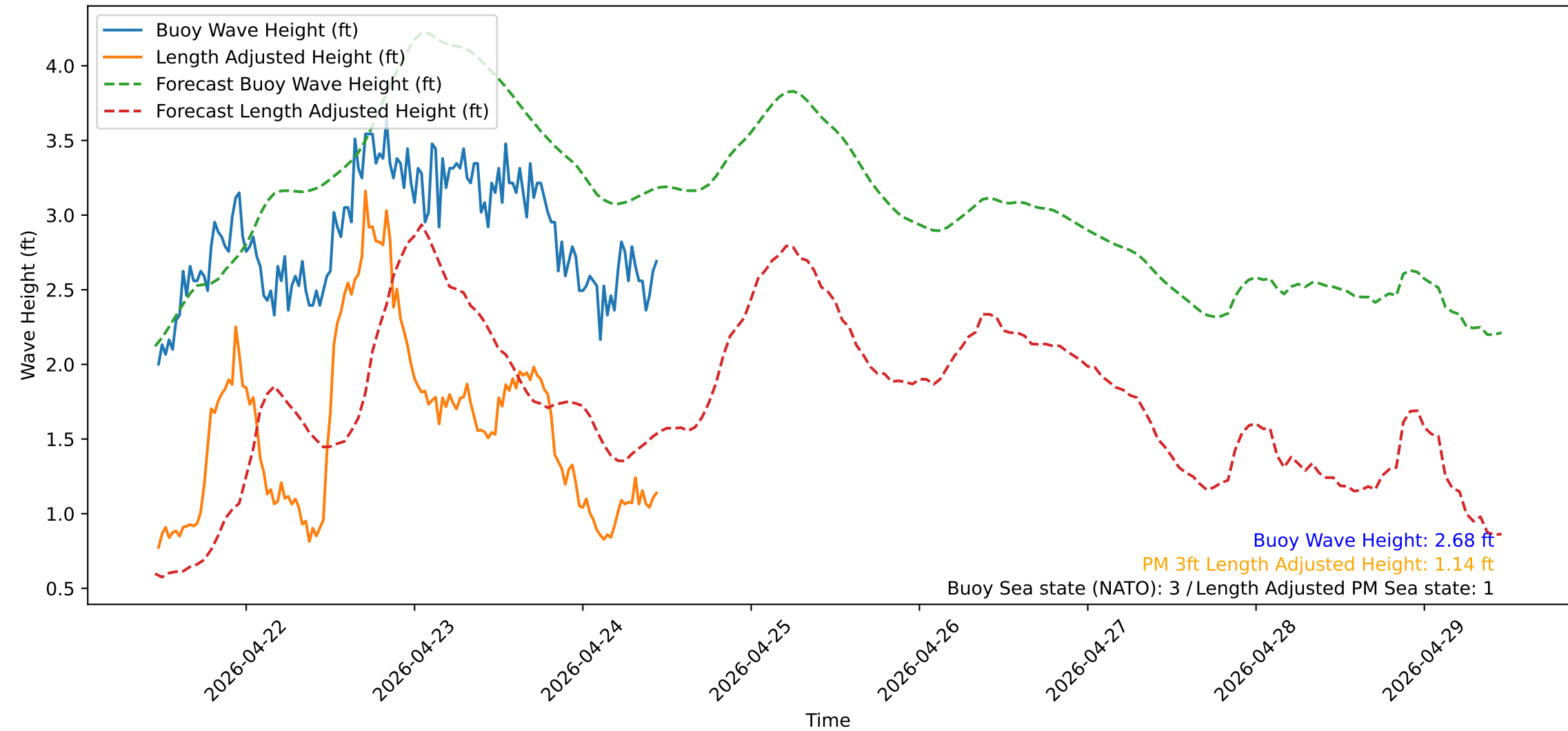
Wave Heights over Time for Red Beach at 2026-04-24 11:10:51
