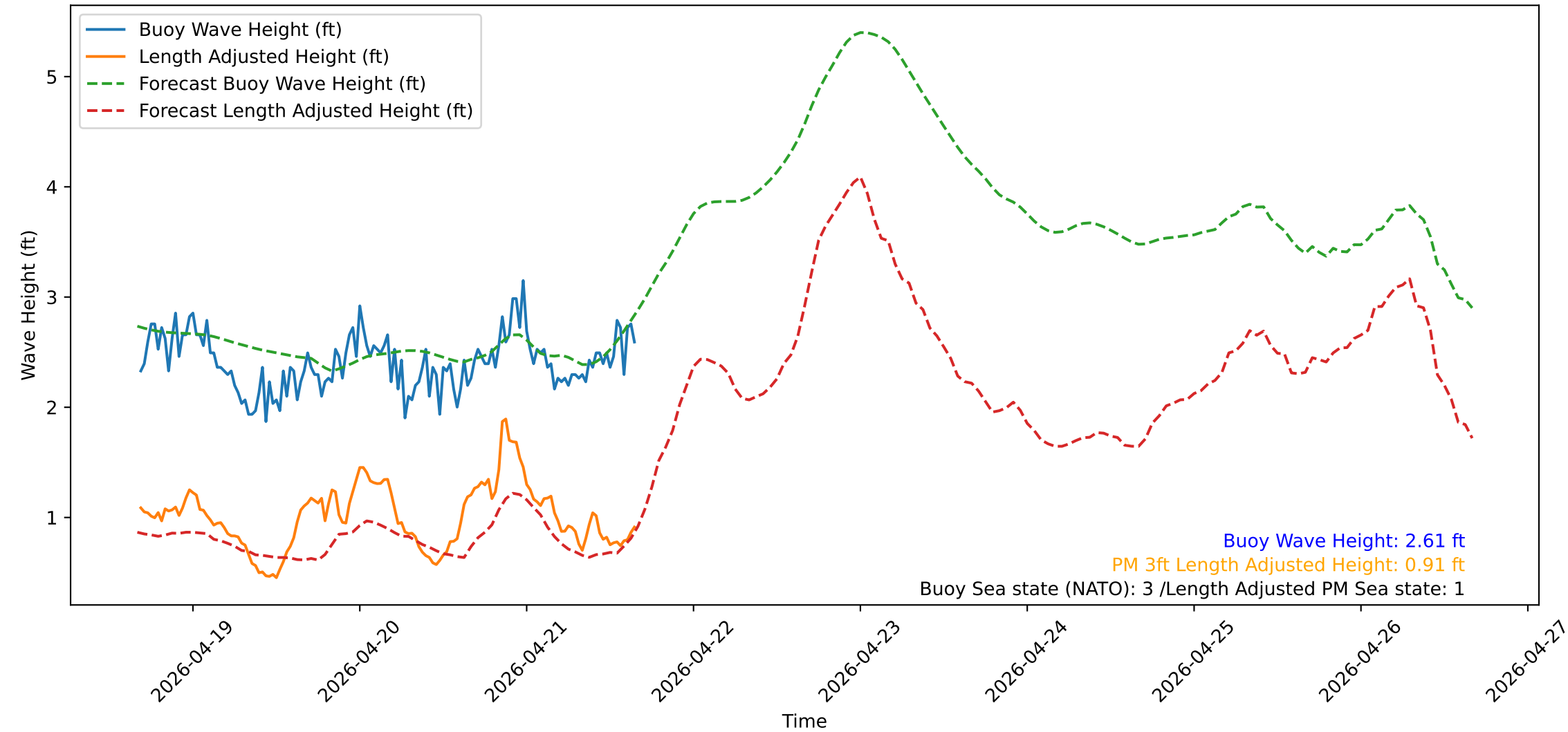
Wave Heights over Time for Green Beach at 2026-04-21 16:21:15
