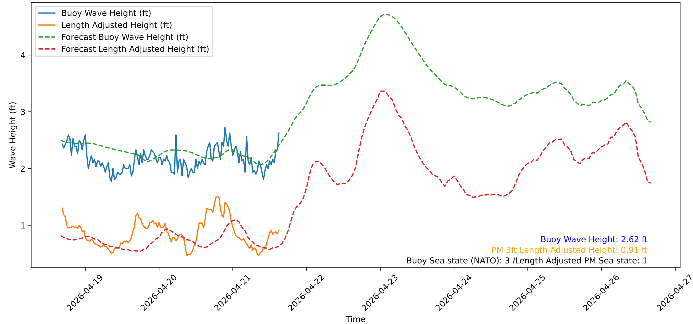
Wave Heights over Time for Red Beach at 2026-04-21 16:20:53
