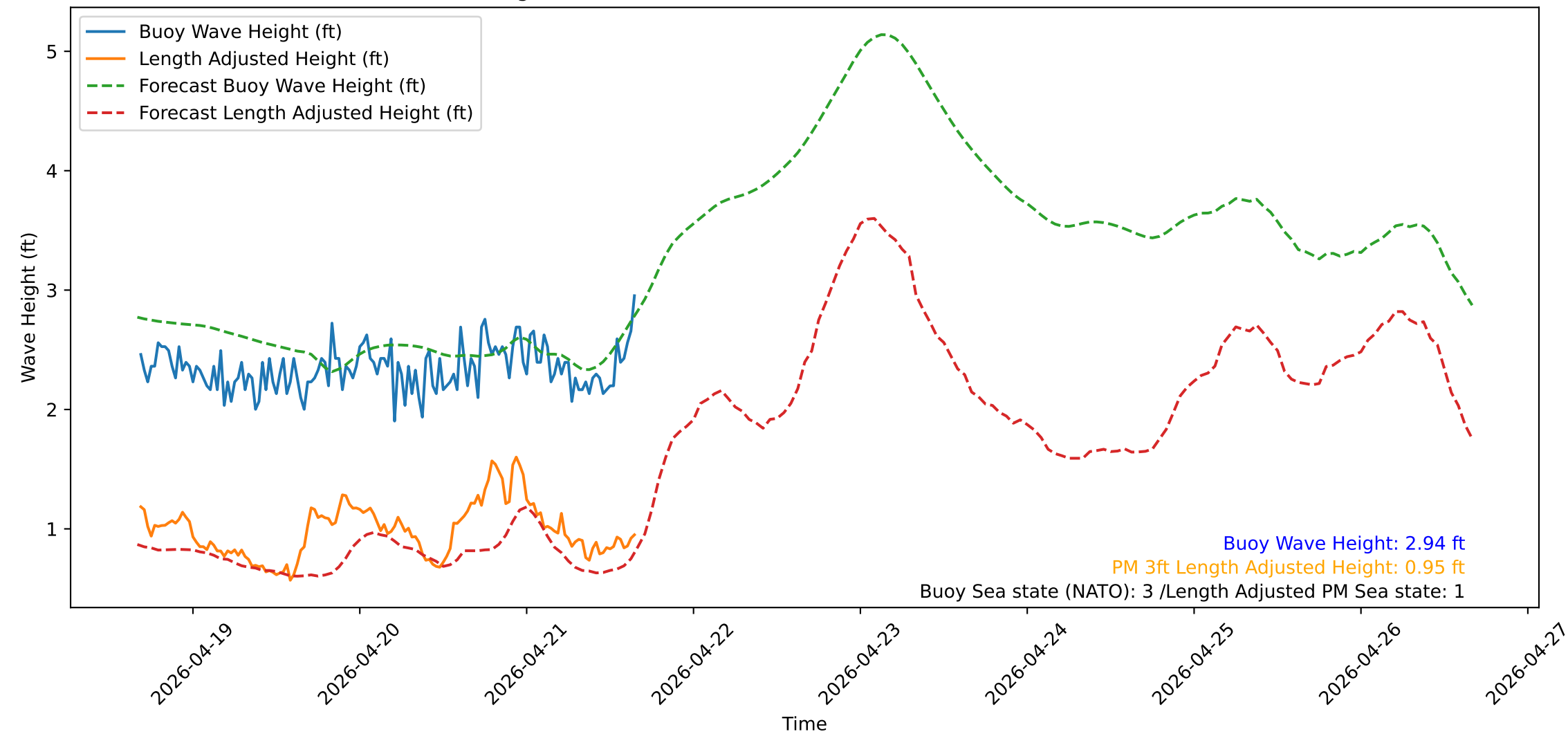
Wave Heights over Time for Oceanside Harbor at 2026-04-21 16:20:33
