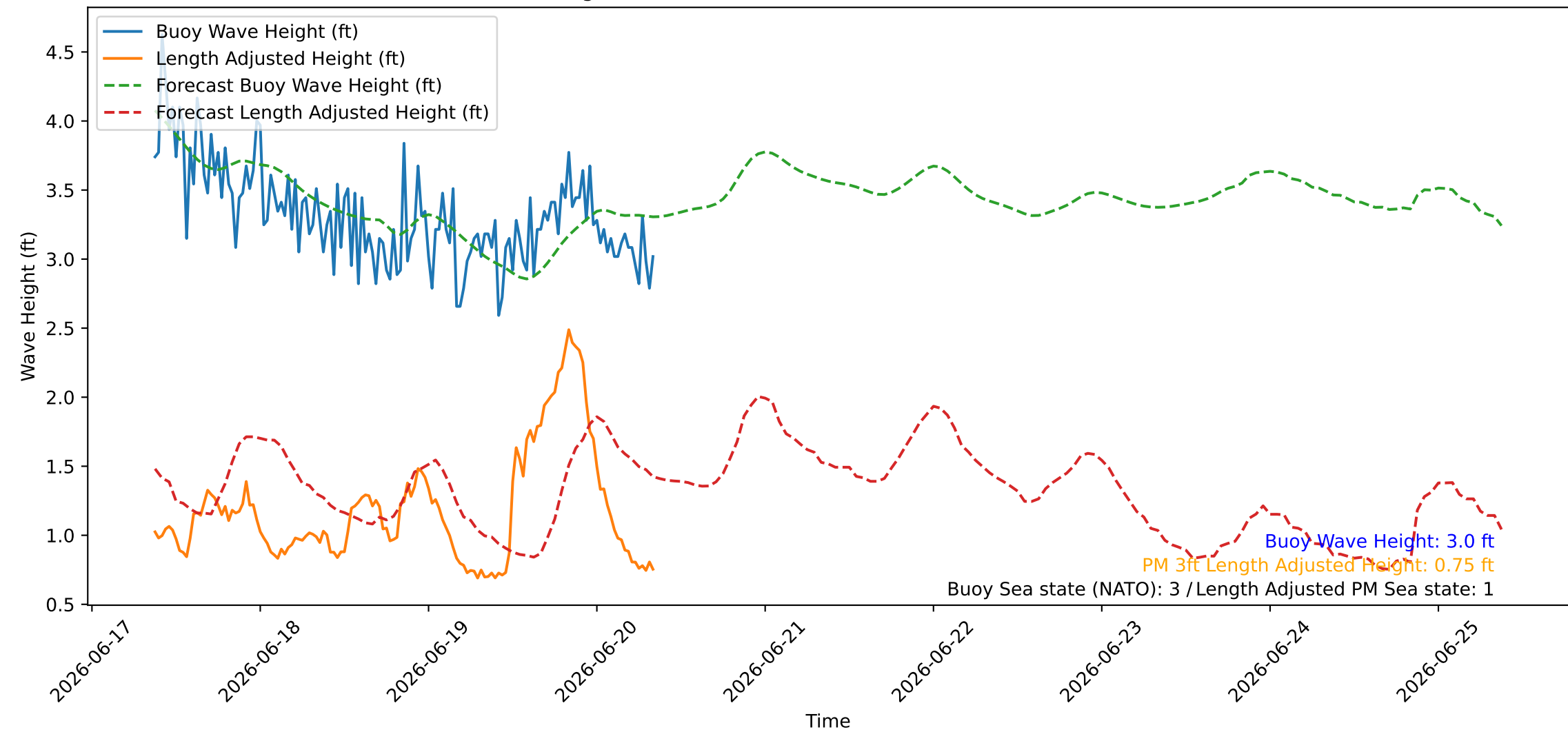
Wave Heights over Time for Red Beach at 2026-06-20 08:50:46
