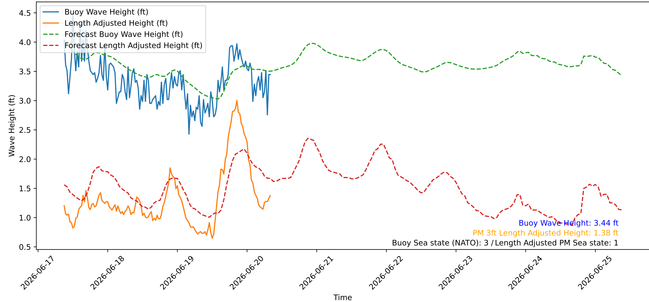
Wave Heights over Time for Green Beach at 2026-06-20 08:51:09
