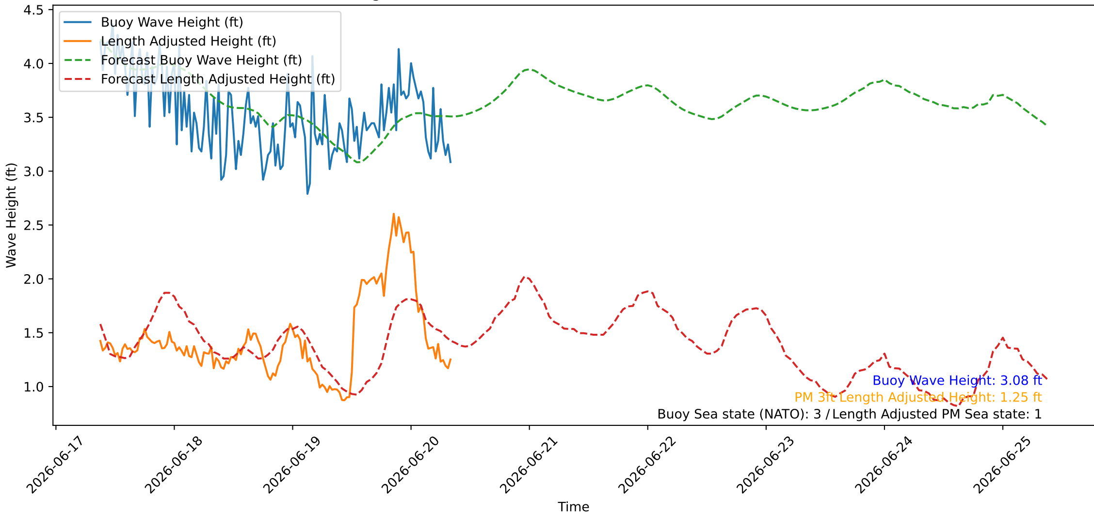
Wave Heights over Time for Oceanside Harbor at 2026-06-20 08:50:26
