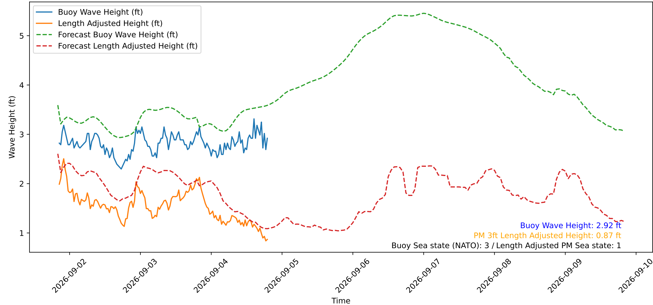
Wave Heights over Time for Red Beach at 2026-09-04 20:00:50
