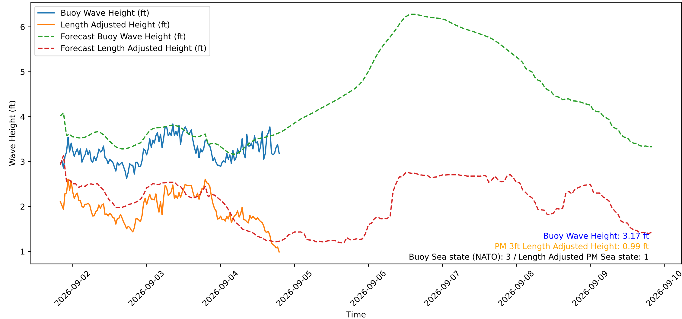
Wave Heights over Time for Oceanside Harbor at 2026-09-04 20:00:30
