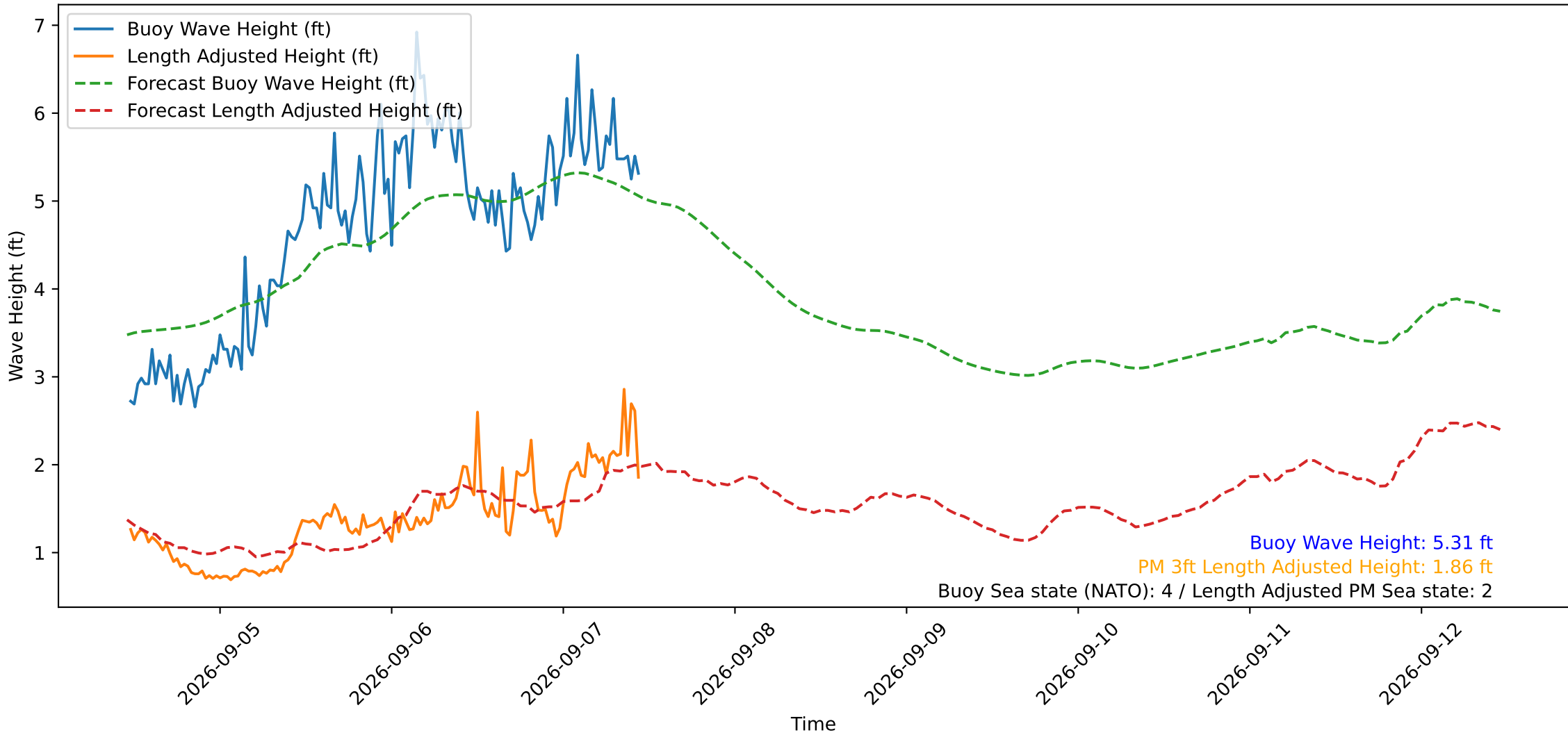
Wave Heights over Time for Red Beach at 2026-09-07 11:10:50
