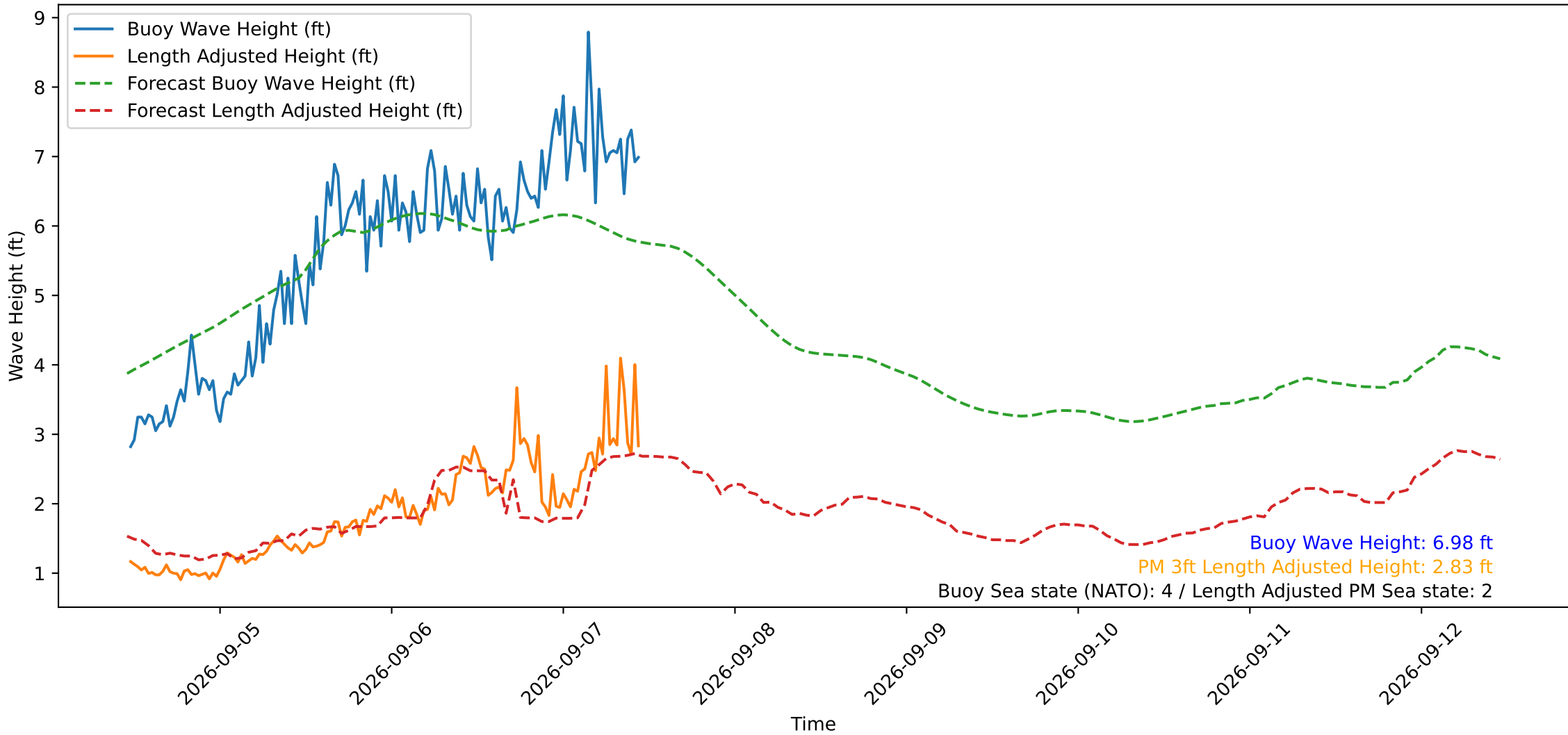
Wave Heights over Time for Green Beach at 2026-09-07 11:11:12
