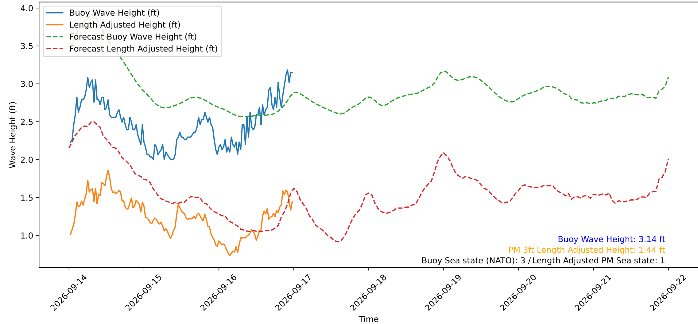
Wave Heights over Time for Red Beach at 2026-09-17 00:20:51
