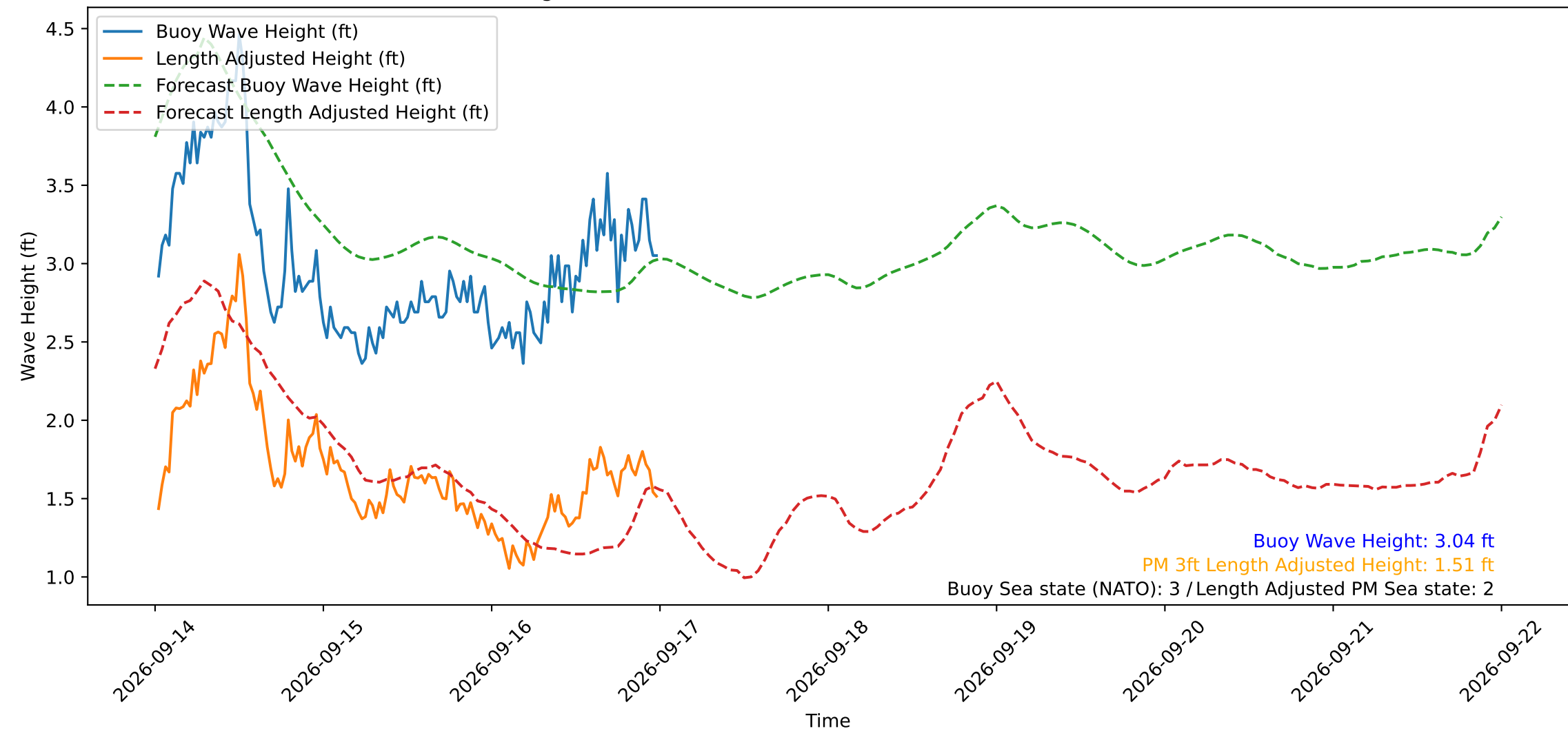
Wave Heights over Time for Oceanside Harbor at 2026-09-17 00:20:30
