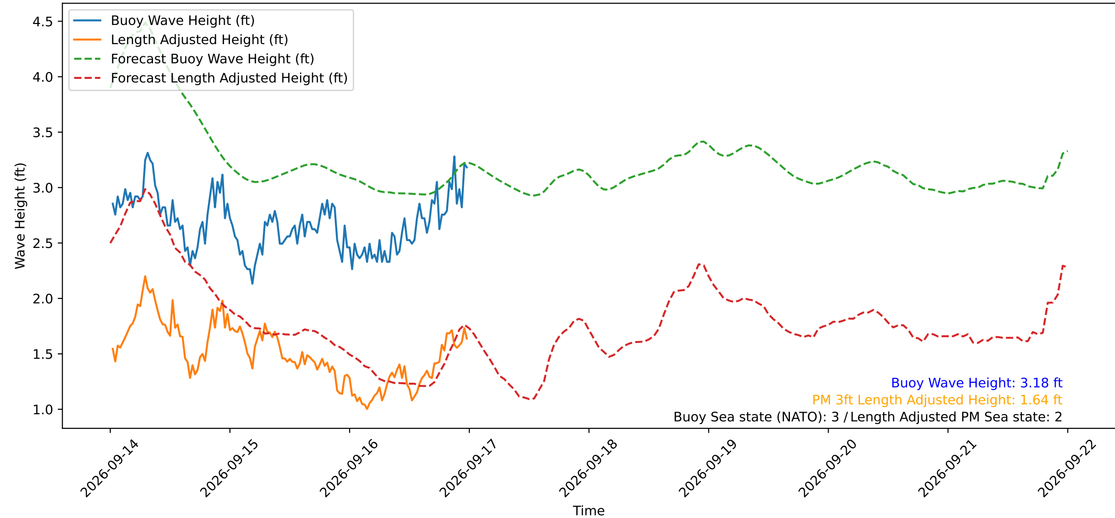
Wave Heights over Time for Green Beach at 2026-09-17 00:21:15
