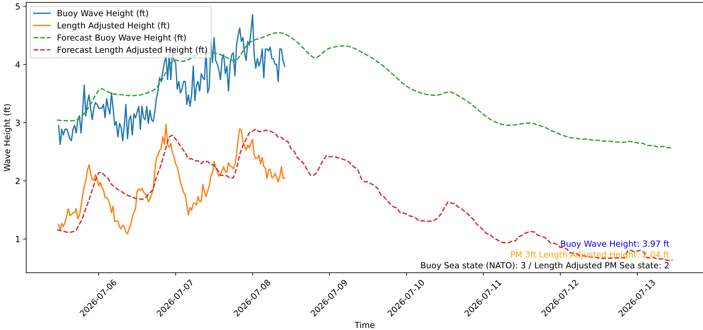
Wave Heights over Time for Red Beach at 2026-07-08 11:10:46
