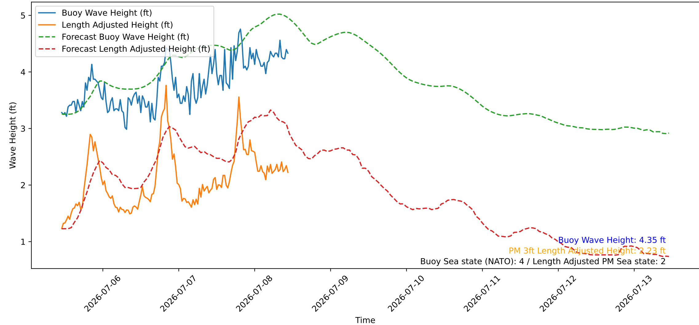
Wave Heights over Time for Green Beach at 2026-07-08 11:11:08
